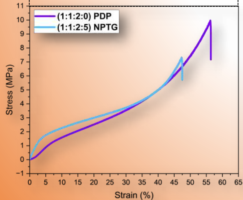
Stress-strain curve of PDP & NPTG
