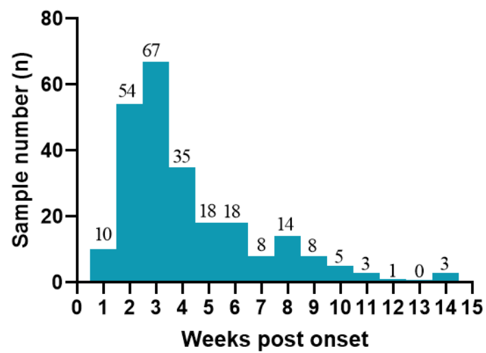
Supplementary Figure 3 Time distribution of samples collection
