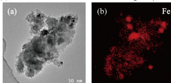
Fig. S4 (a) TEM image of 10Fe 2 O 3 /Al 2 O 3 ; (b) Distribution of Fe element in EDS image of 10Fe 2 O 3 /Al 2 O 3
