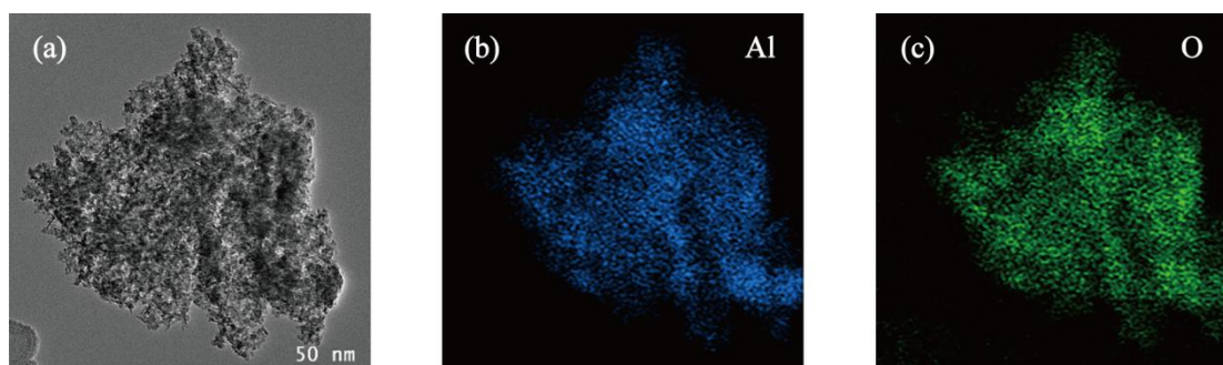
Fig. S3 (a) TEM image of \gamma -Al 2 O 3 ; (b) Distribution of Al element in EDS image of \gamma -Al 2 O 3 ; (c) Distribution of O element in EDS image of \gamma -Al 2 O 3
