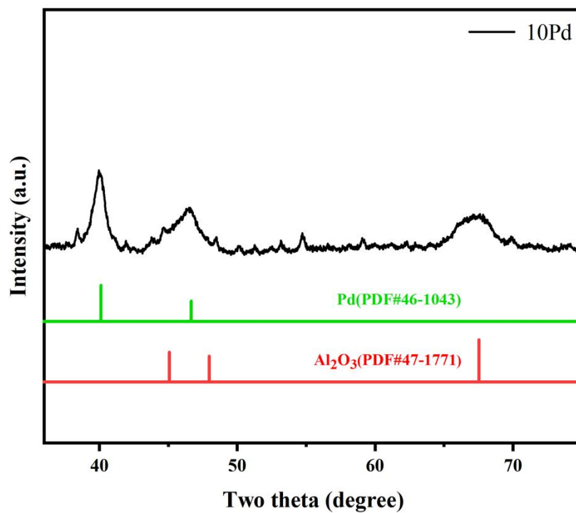
Fig. S2 XRD patterns of 10Pd/Al 2 O 3
