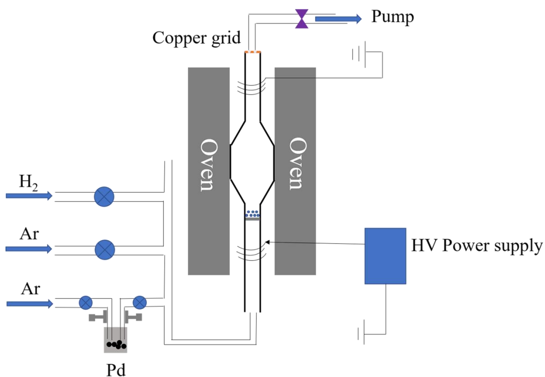
Figure S1. Schematic of the experimental set-up
