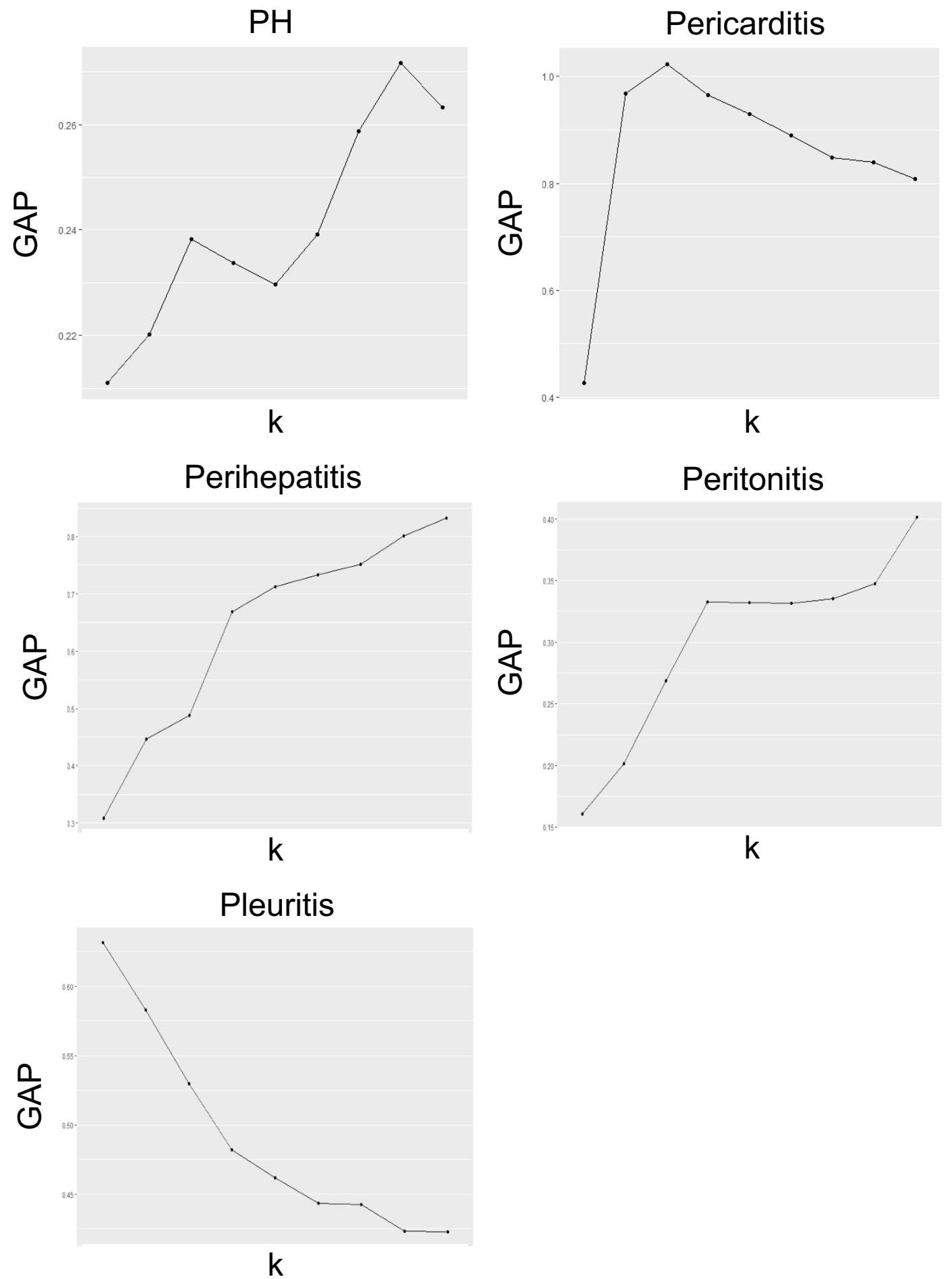
The figure shows the gap statistics for each disease. In the figure, the vertical axis indicates gap statistics, and the horizontal axis k indicates the number of clusters.
