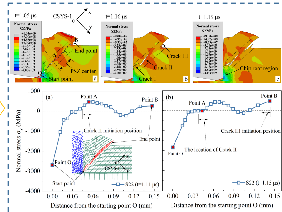
Formation mechanism of discontinuously segmented chip
