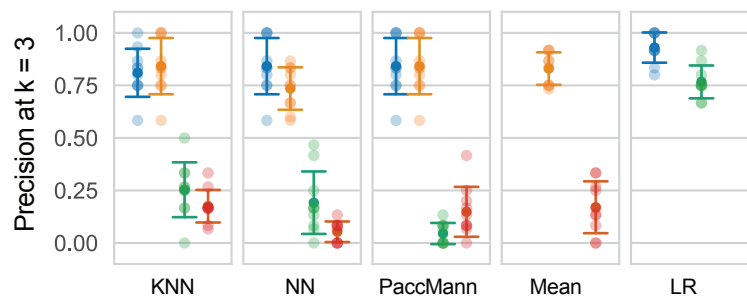
Trained and tested on PCPL
