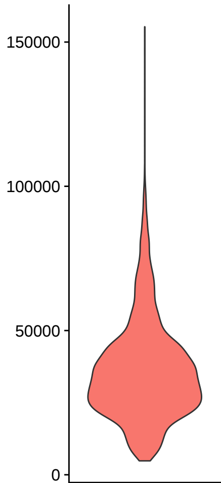
nCount_RNA
