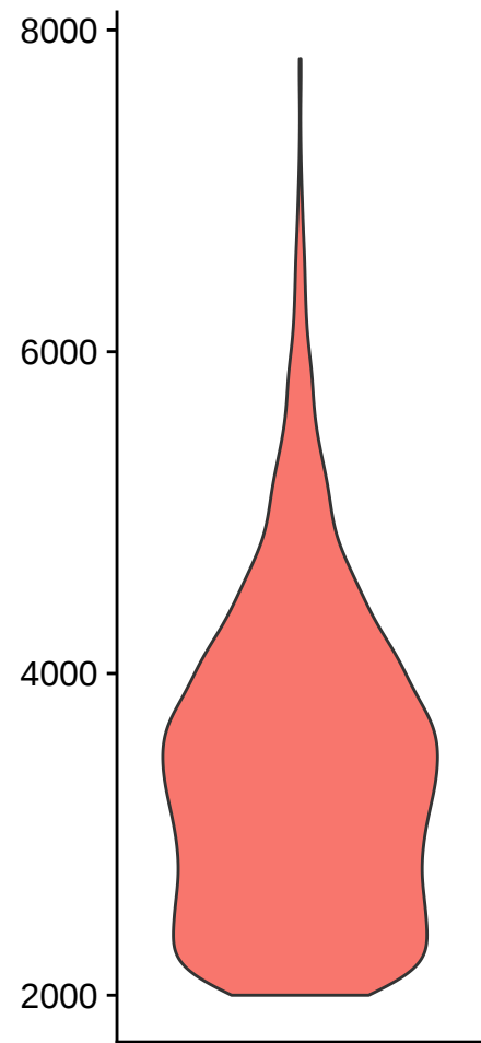
nFeature_RNA
