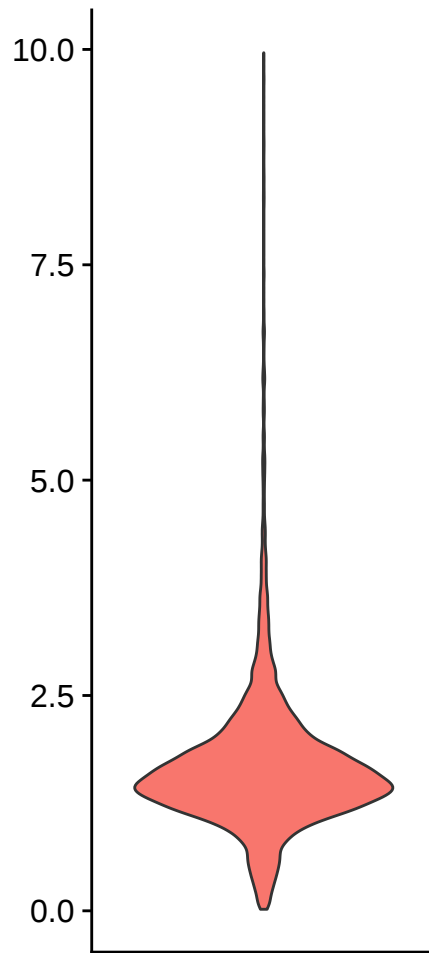
percent.mt
