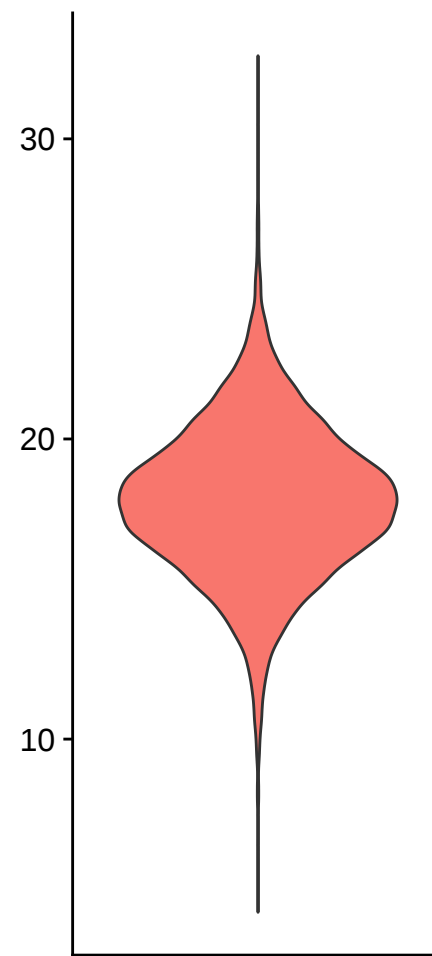
percent.ribo
