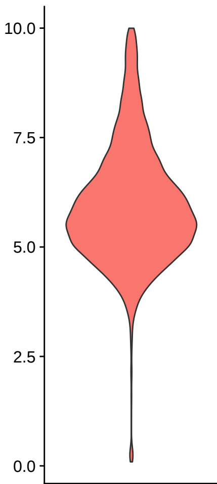
percent.mt
