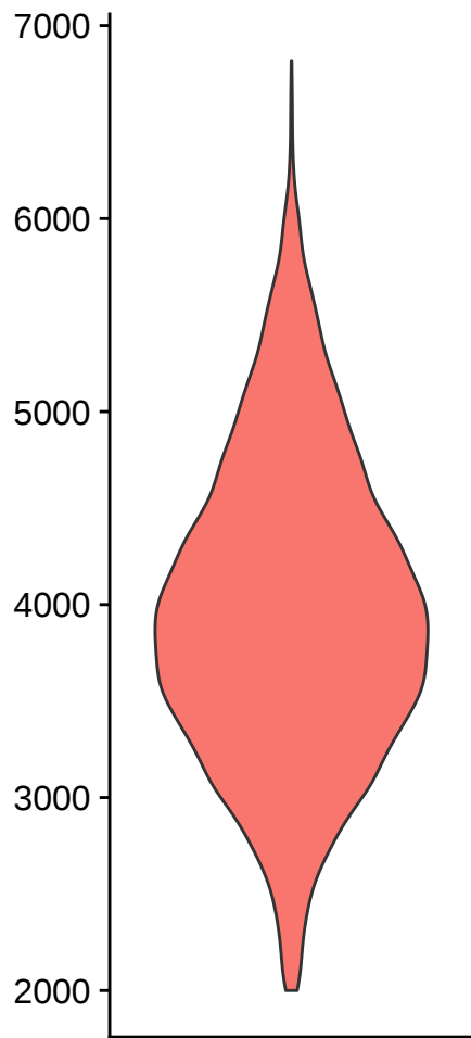
nFeature_RNA
