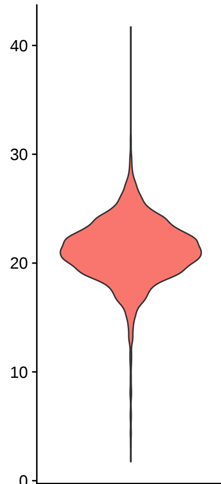
percent.ribo
