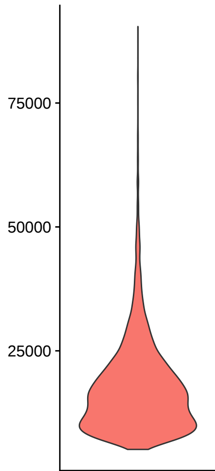
nCount_RNA
