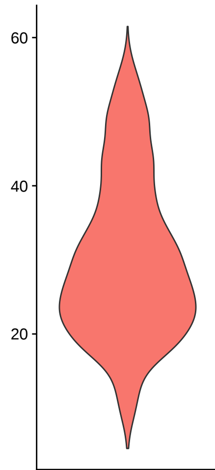
percent.ribo
