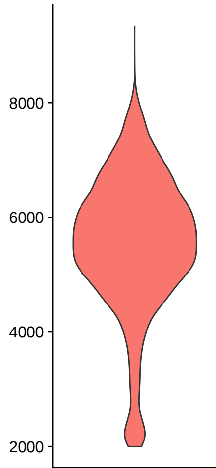
nFeature_RNA
