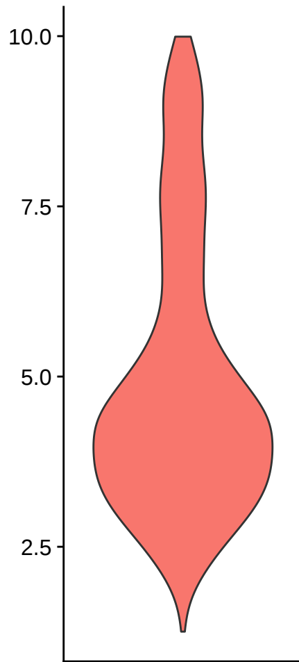
percent.mt
