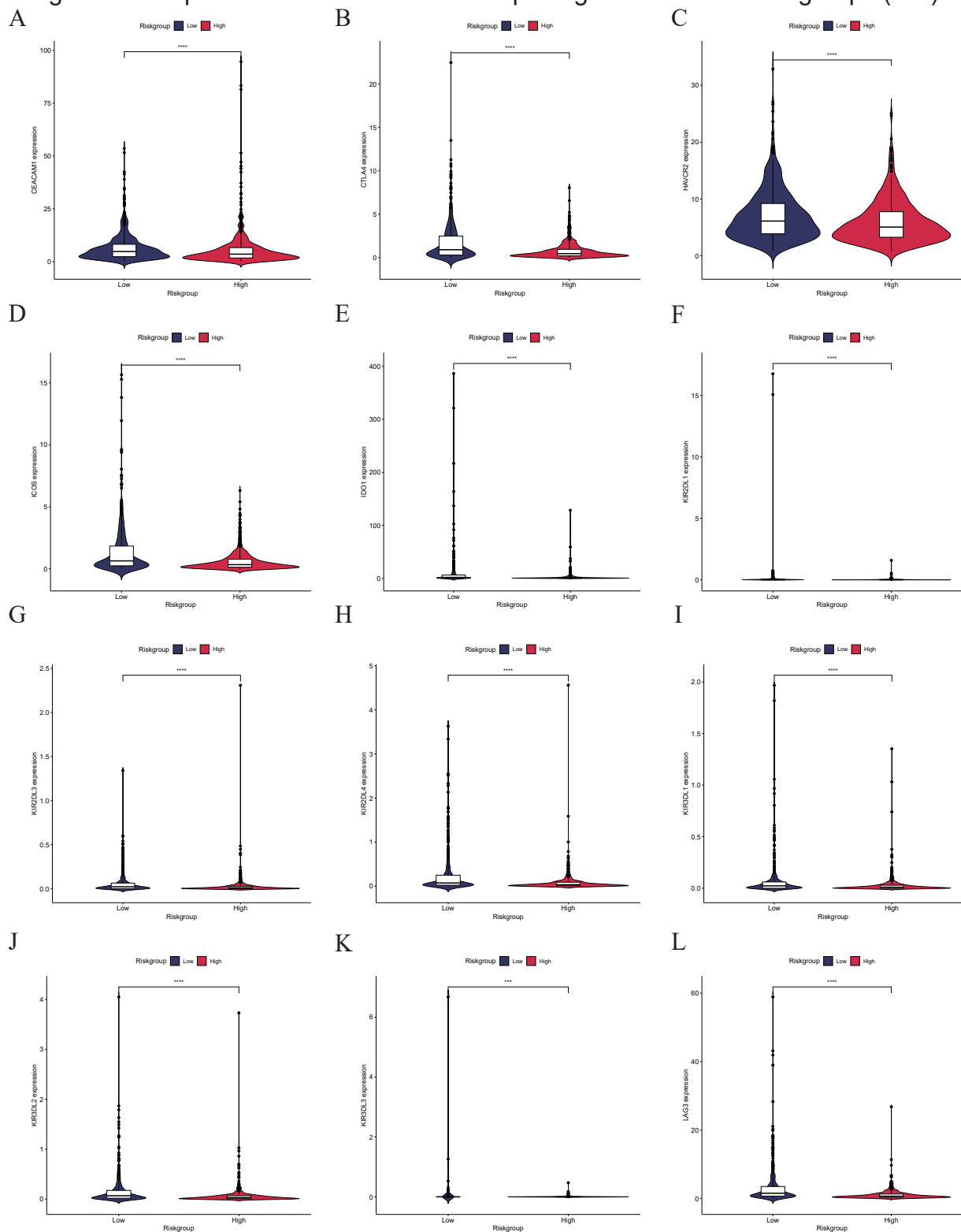
Fig S1 The expression of 12 immune checkpoint genes between two groups (A-L).
