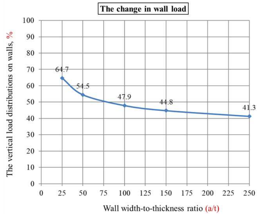
Figure 8. The vertical load distribution on walls with various width-to-thickness ratios ( a/t )
