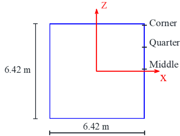
Figure 16. Slender silo cross section with a 16-meter height [h/a = 2.5]
