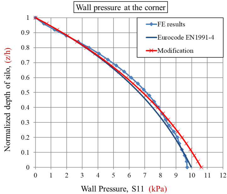
Figure 14. Comparison of the modified Janssen approach, the current Eurocode approach, and the FE results, (a) at the middle, (b) at the quarter, (c) at the corner [ h/a= 1.67 ]
