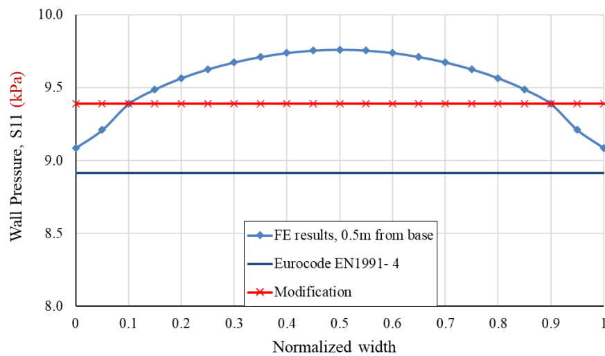
Figure 13. Comparison of different lateral wall pressures in the squat silo, (a) at the middle, (b) above the base by 0.5 m [ h/a = 1.67 ]
