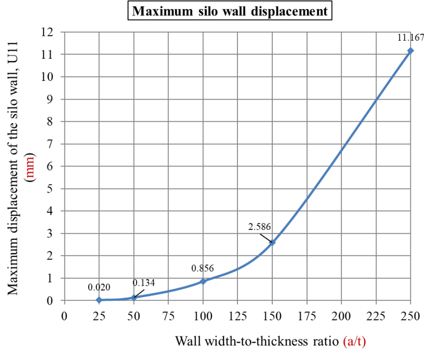
Figure 7. Wall deformation as wall width-to-thickness ratios ( a/t ) change
