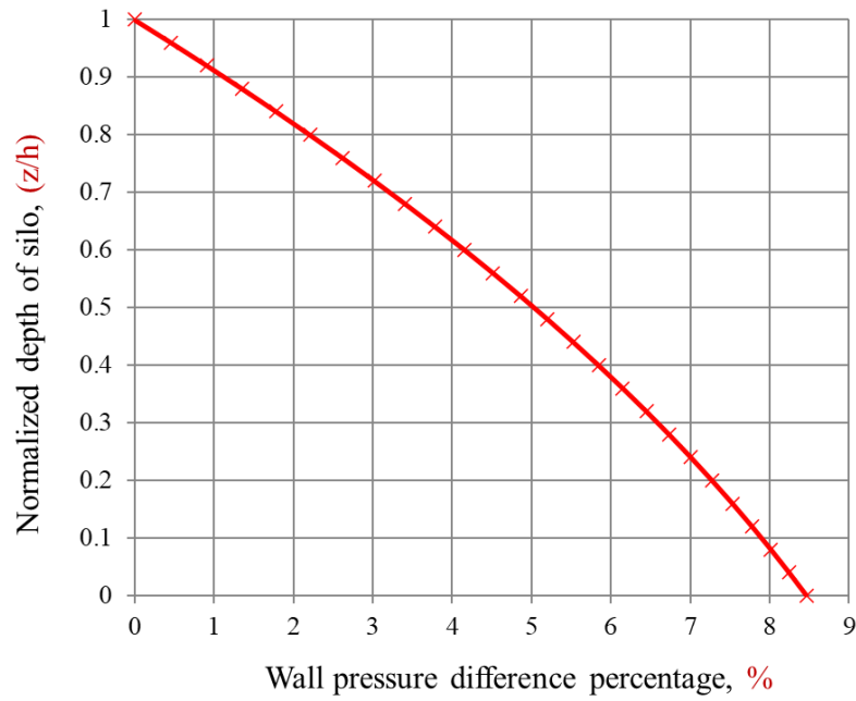
Figure 19. The normalized difference percentage of wall pressure between the modified and the existing Eurocode approaches for a slender silo
