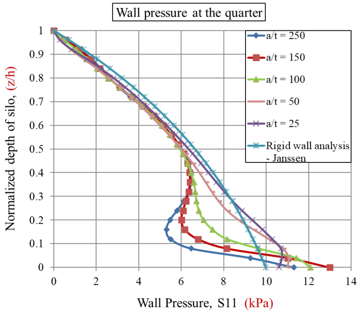
Figure 3. Wall-filling pressures for various wall width-to-thickness ratio models, (a) square silo cross section sketch, (b) at the middle, (c) at the quarter, (d) at the corner [ h/a = 1.67 ]
