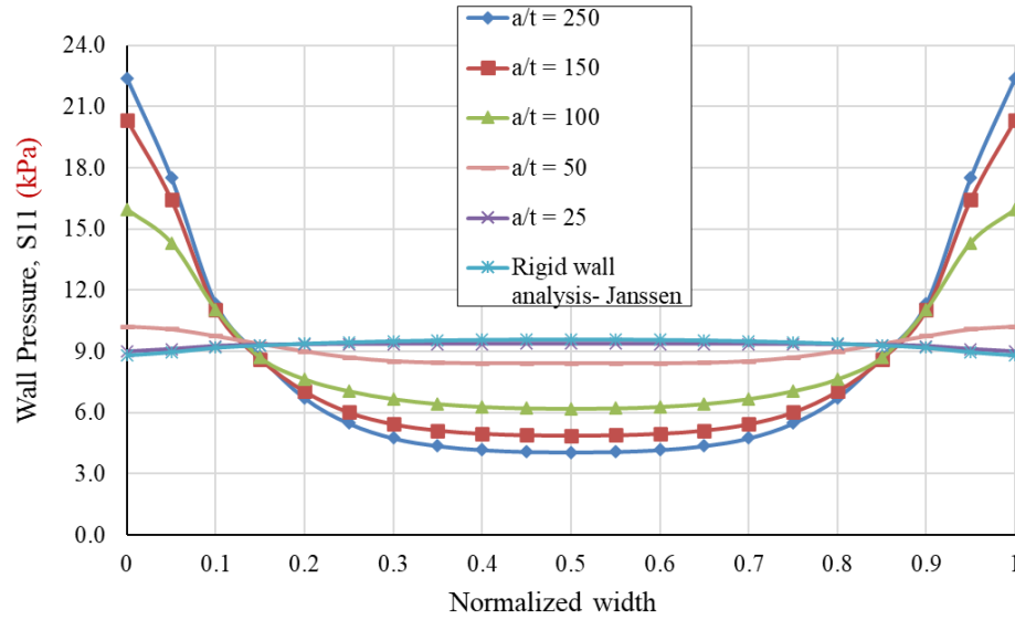
Figure 4. Effect of wall width-to-thickness ratios on lateral wall pressure above the base by 0.5 m (20% of the silo height).
