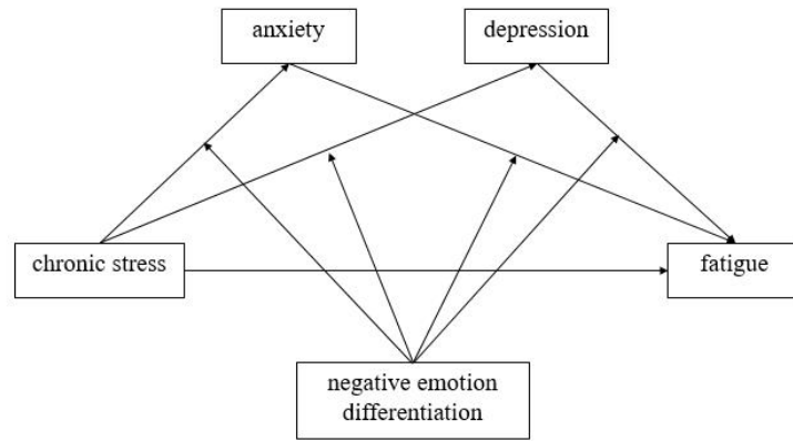
Figure 1 Hypothesized model
