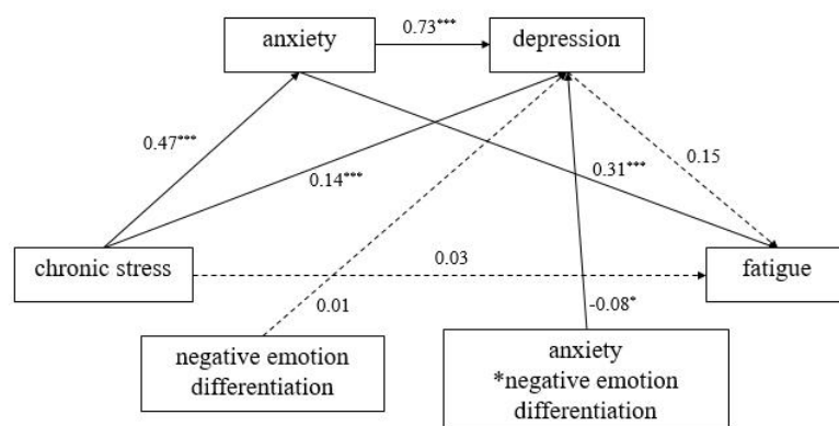
Figure 2 Statistical model
