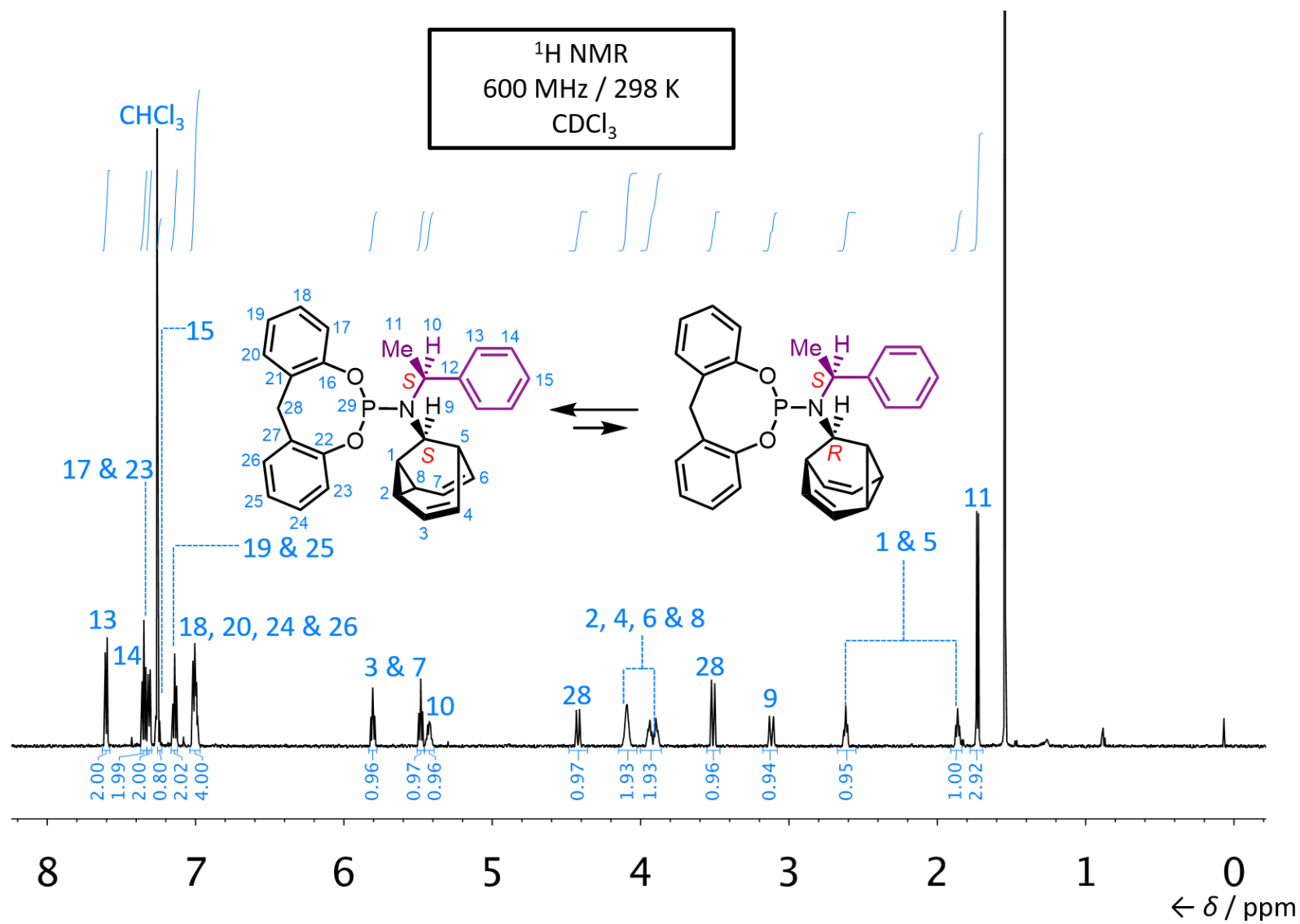
Figure S26. ^1\text{H} NMR spectrum of (R,S)/(S,S)\text{-LBB} .
