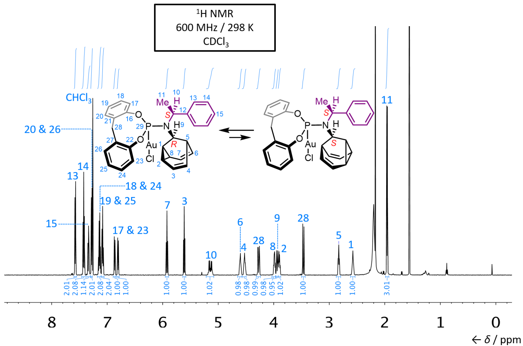
Figure S29. 1 H NMR spectrum of (R,S)/(S,S)-LBBAuCl.
