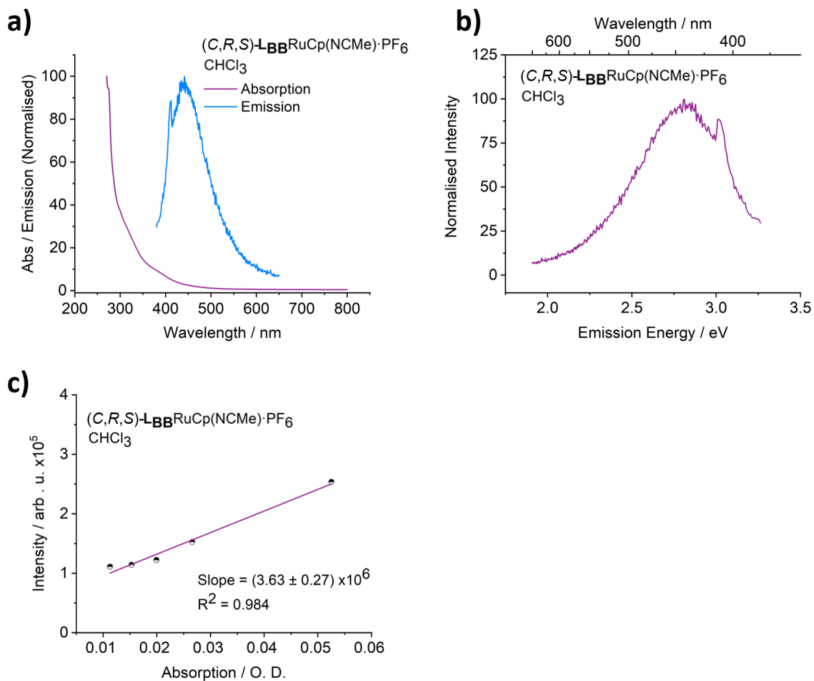
Figure S55. The (a) combined absorption and emission spectra (380 \mu M, \lambda_{\text{ex}} = 365 nm), (b) emission spectra and (c) emission vs. absorption slope of ( C,R,S )- L BB RuCp(NCMe)·PF 6 in CHCl 3 .
