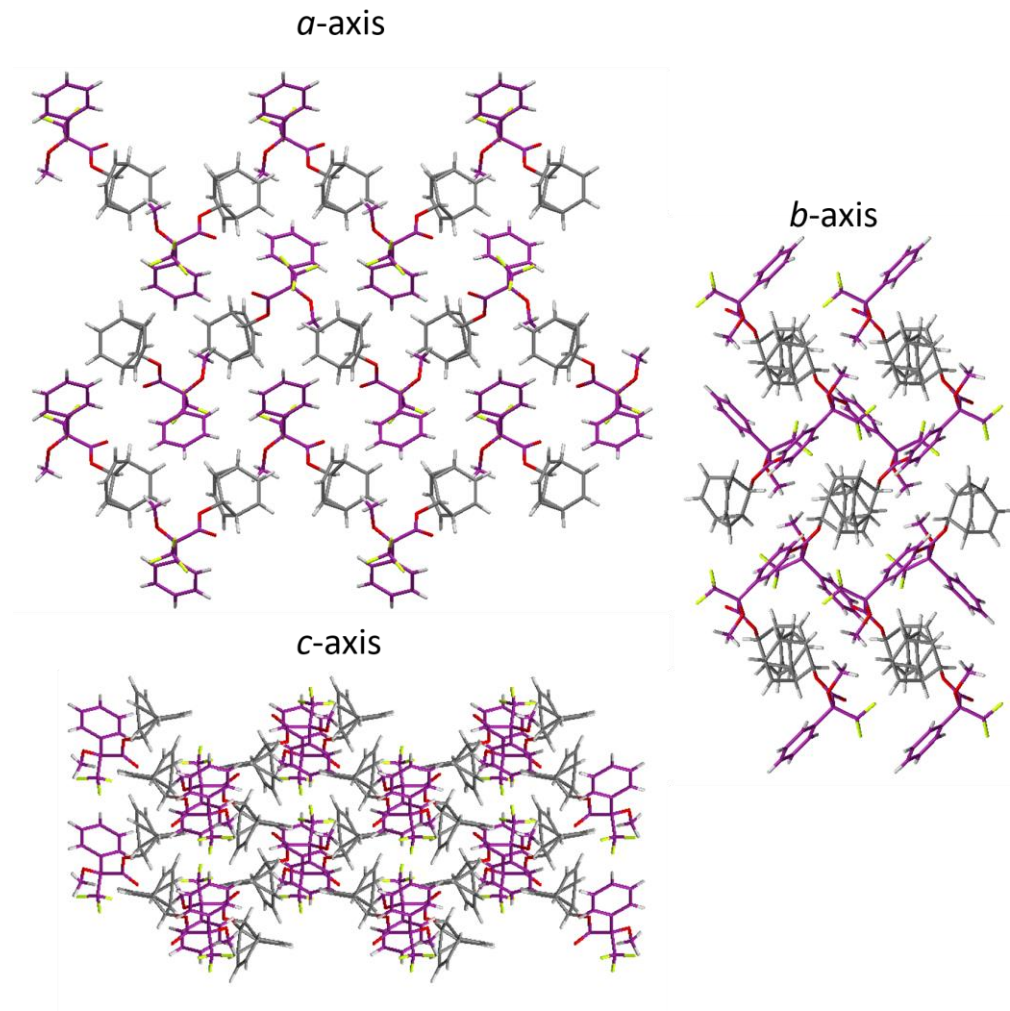
Figure S60. Solid-state superstructure of ( S,S )- 2 viewed along the three unit cell axes.
