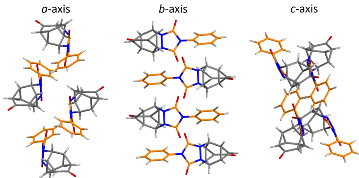
Figure S69. Solid-state superstructure of S1 viewed along the three unit cell axes.
