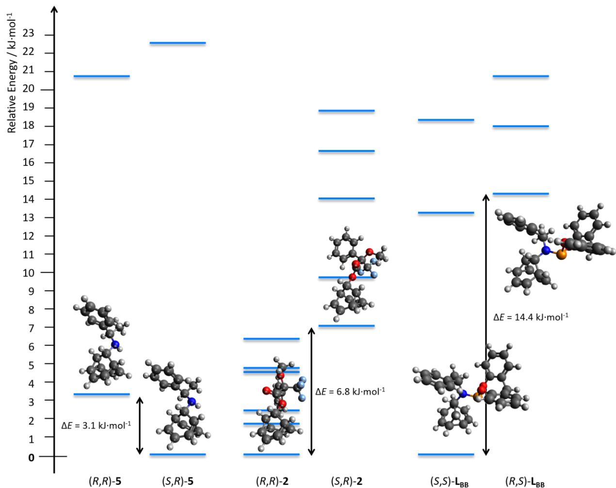
Figure S77. Relative energies of DFT optimised conformers of 2 , 5 , and L BB . The geometries of the minimum energy structures are shown.
