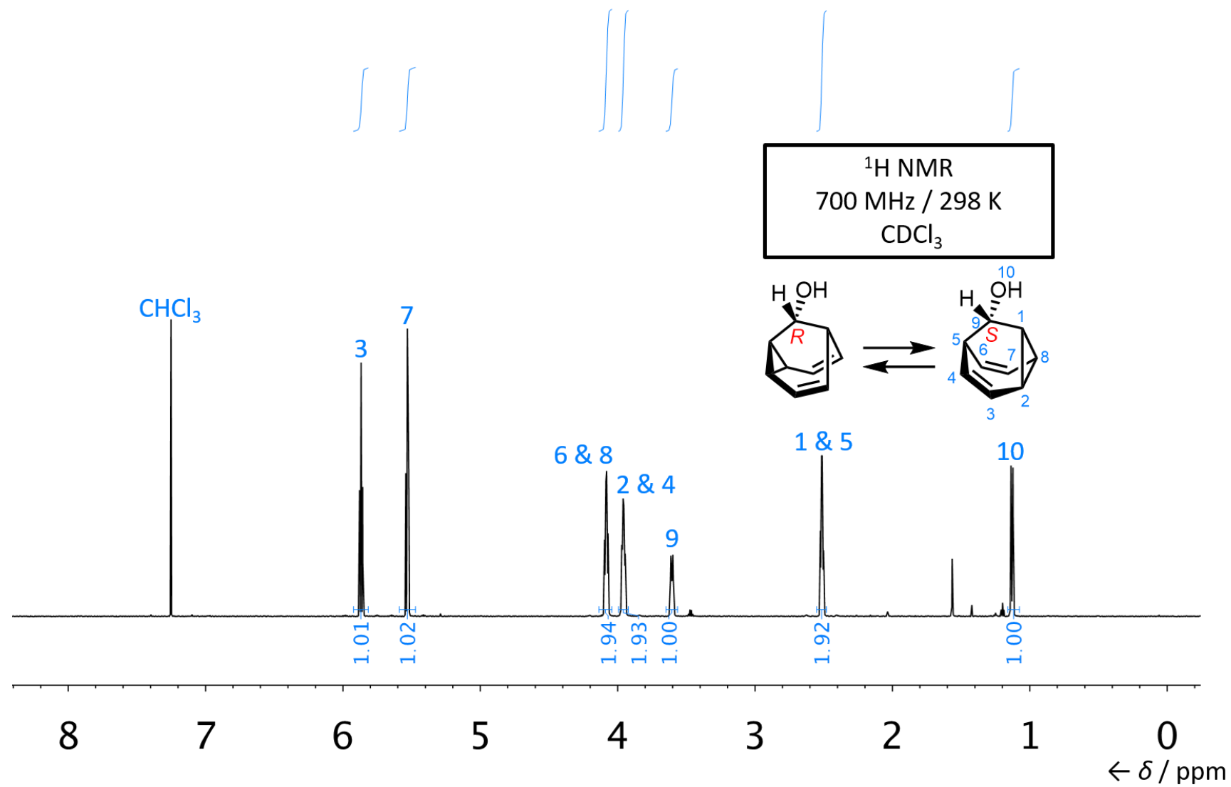
Figure S6. 1 H NMR spectrum of ( R )/( S )- 1 .
