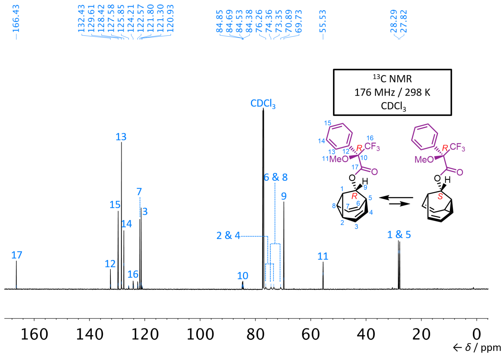
Figure S12. 13 C NMR spectrum of (R,R)/(S,R) -2.
