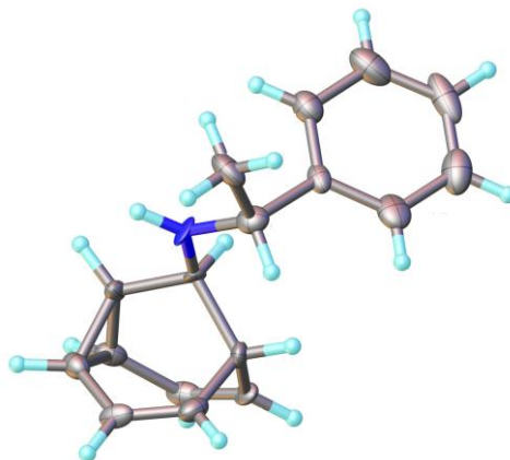
Figure S70. Solid-state structure of ( R,S )- 5 including probability ellipsoids at 50%.
