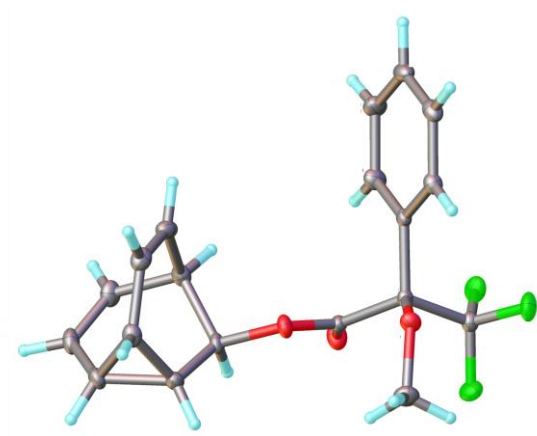
Figure S61. Solid-state structure of ( R,R )-2 including probability ellipsoids at 50%.
