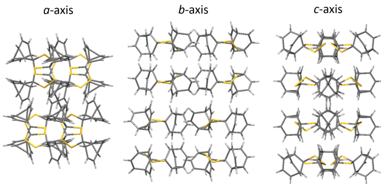
Figure S64. Solid-state superstructure of ( R,R )/( S,S )-4 viewed along the three unit cell axes.
