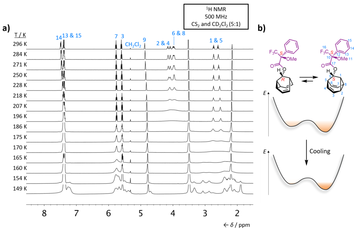
Figure S46. Partial ^1\text{H} VT NMR spectra of (a) (R,S)/(S,S) - 2 (296 K to 149 K) and (b) a schematic illustration of the change in equilibrium population on a simplified potential energy surface as the temperature decreases.
