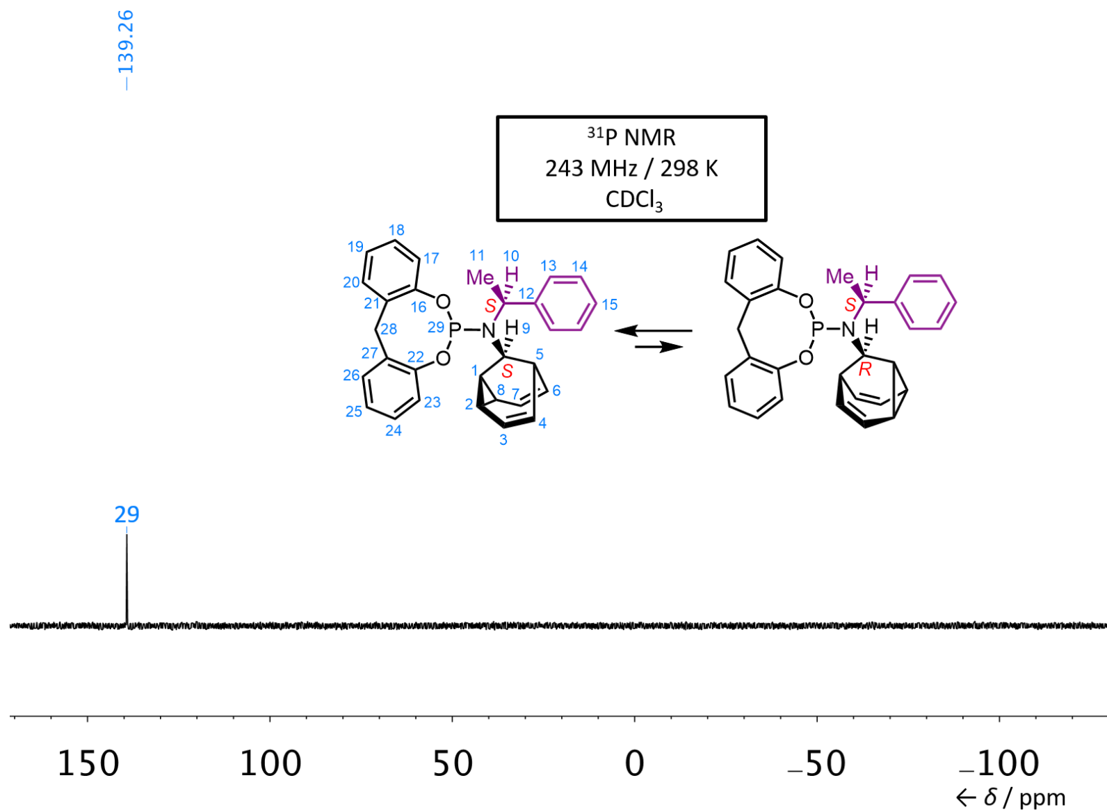
Figure S28. ^{31}\text{P} NMR spectrum of (R,S)/(S,S)\text{-L}_{\text{BB}} .
