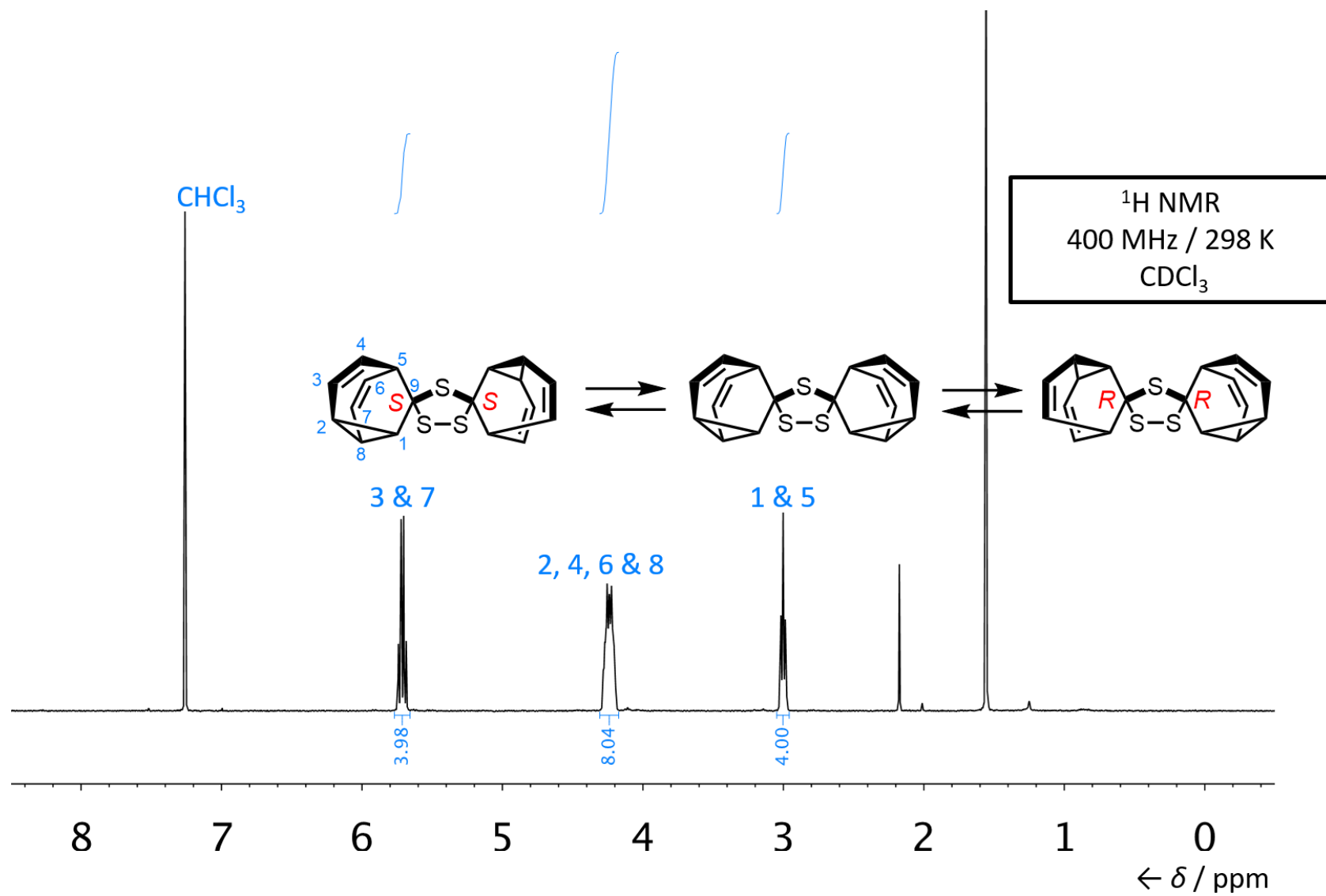
Figure S14. 1 H NMR spectrum of ( R,R )/ meso /( S,S )-4.
