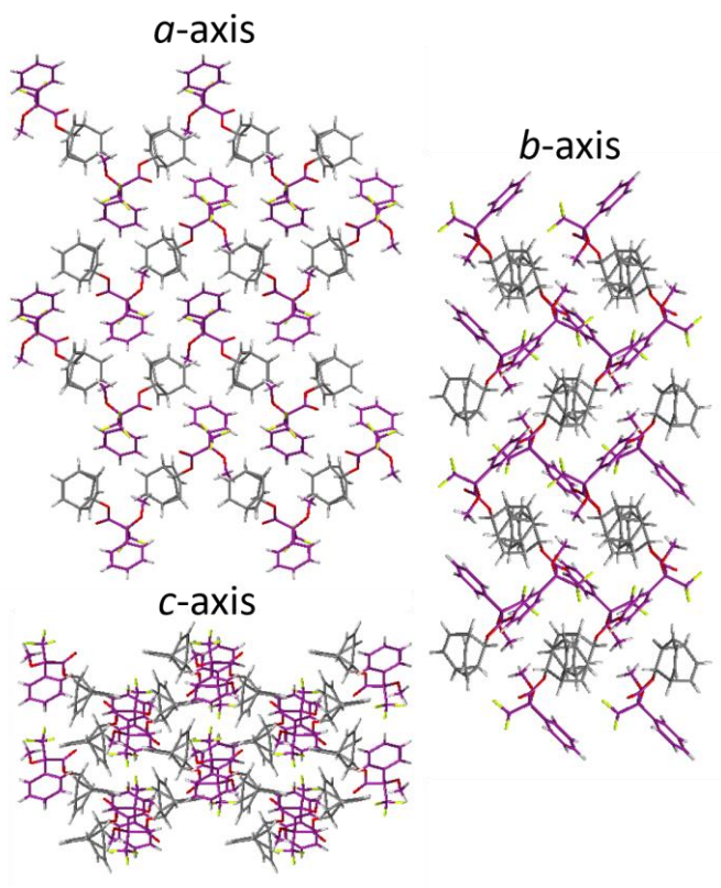
Figure S62. Solid-state superstructure of ( R,R )- 2 viewed along the three unit cell axes.
