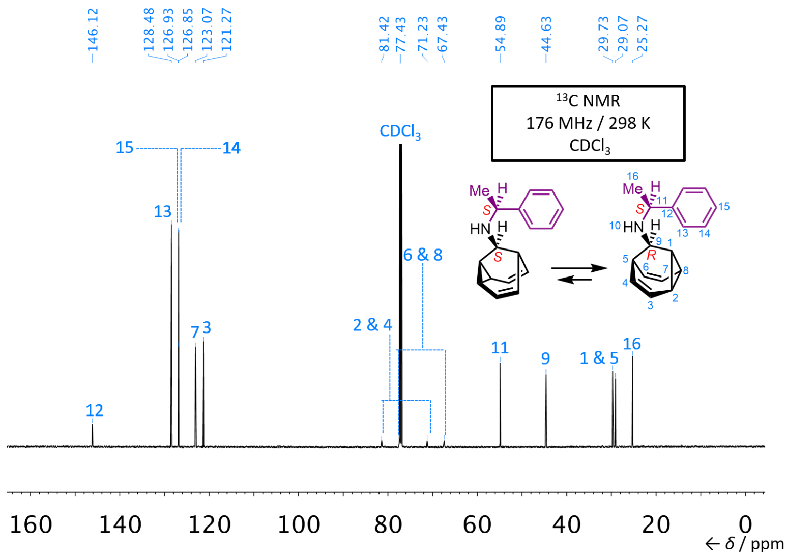
Figure S23. 13 C NMR spectrum of (S,S)/(R,S)-5.
