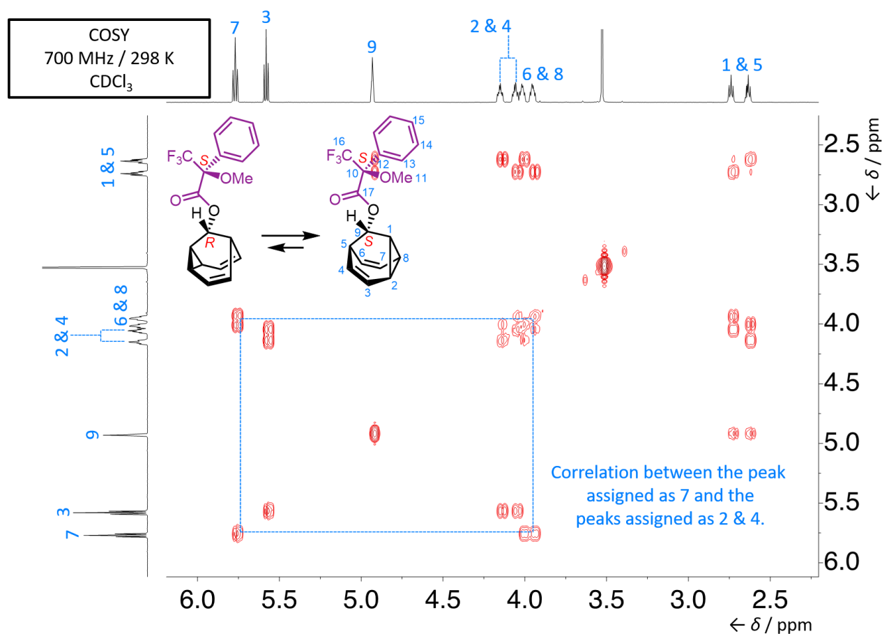
Figure S41. Partial COSY spectrum of (R,S)/(S,S) -2.
