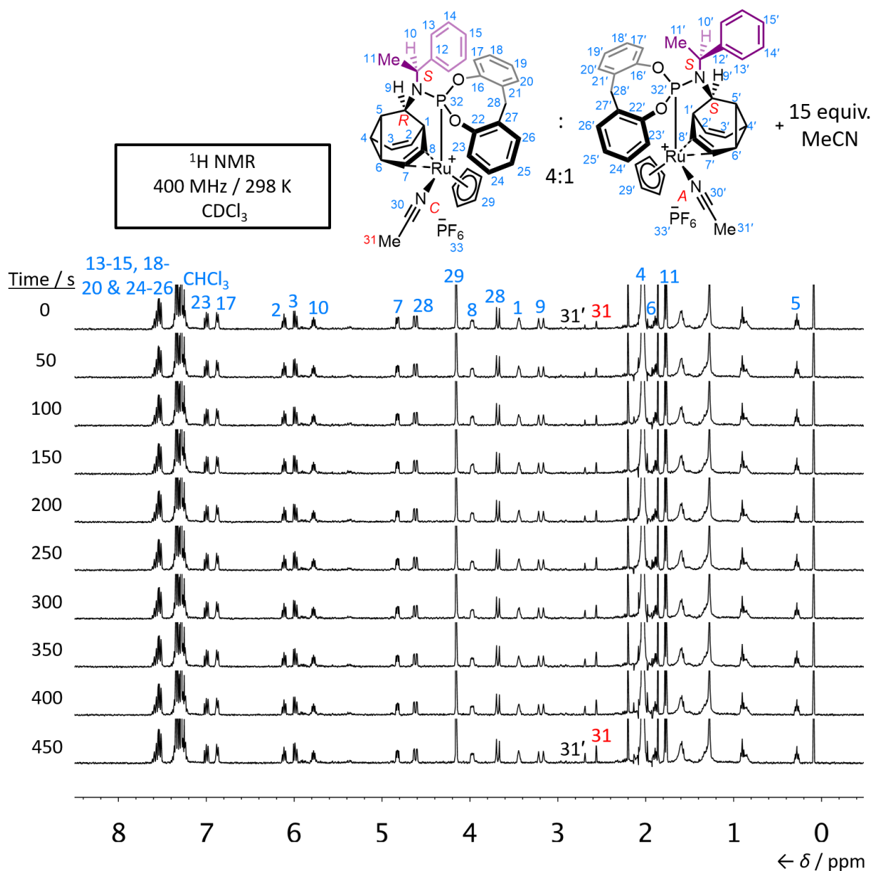
Figure S52. Partial ^1\text{H} NMR spectra of a 4:1 equilibrium mixture of (C,R,S)\text{-L}_{\text{BB}}\text{RuCp}(\text{NCCD}_3)\cdot\text{PF}_6 and (A,S,S)\text{-L}_{\text{BB}}\text{RuCp}(\text{NCCD}_3)\cdot\text{PF}_6 immediately after the addition of 15 equiv. MeCN showing the increase in the intensity of signals (31 and 31') corresponding to coordinated MeCN. Note: Although the spectra show a 4:1 equilibrium mixture of (C,R,S)\text{-L}_{\text{BB}}\text{RuCp}(\text{NCCD}_3)\cdot\text{PF}_6 and (A,S,S)\text{-L}_{\text{BB}}\text{RuCp}(\text{NCCD}_3)\cdot\text{PF}_6 , only the assignment of the major diastereoisomer ( (C,R,S)\text{-L}_{\text{BB}}\text{RuCp}(\text{NCCD}_3)\cdot\text{PF}_6 ) is shown (blue and red labels), with the exception bar the signal corresponding to 31' (black label).
