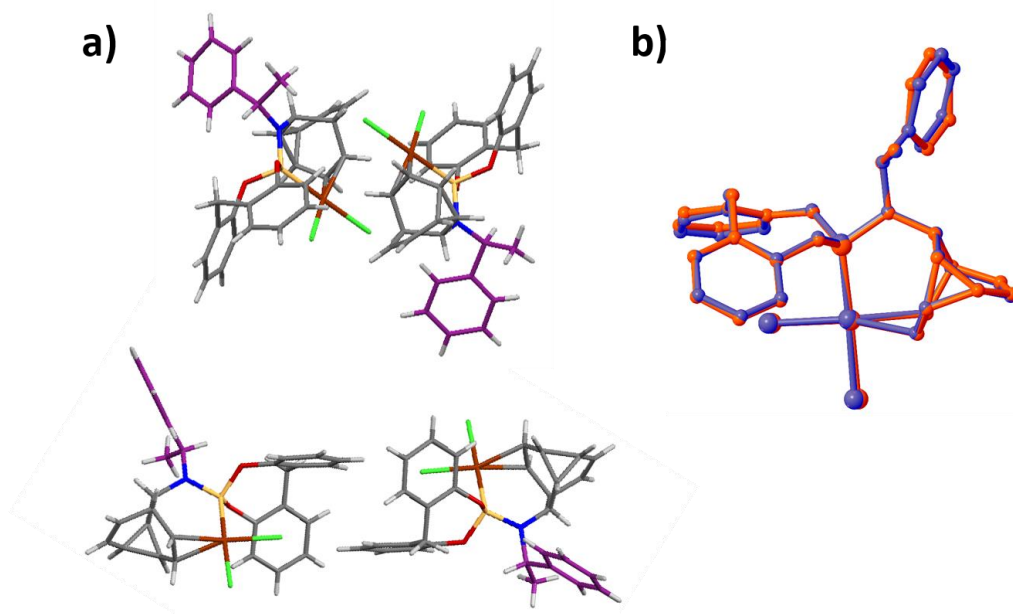
Figure S72. Solid-state structure of (a) the two near-identical conformers of ( A,S,S )- L BB PdCl 2 as well as the two near-identical conformers of ( C,R,S )- L BB PdCl 2 and (b) an overlay of two of the near-identical conformers of ( C,R,S )- L BB PdCl 2 showing the similarity of their geometries.
