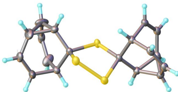
Figure S63. Solid-state structure of ( R,R )/( S,S )-4 including probability ellipsoids at 50%.
