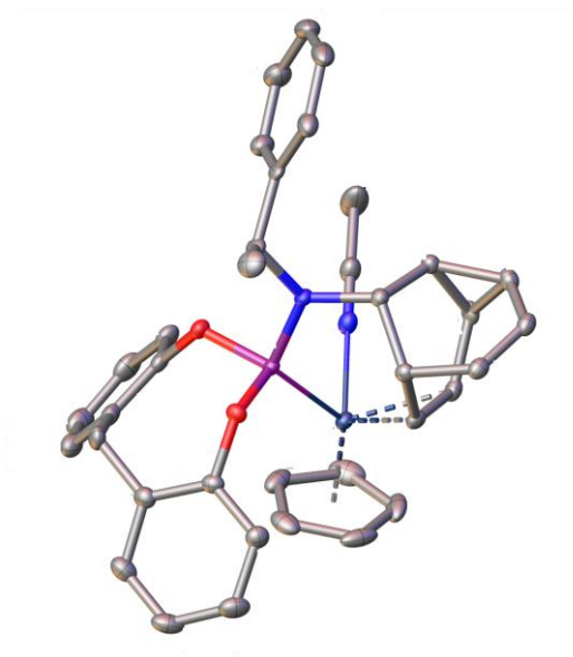
Figure S75. Solid-state structure of (C,R,S)\text{-L}_{\text{BB}}\text{RuCp}(\text{NCMe})\cdot\text{PF}_6 including probability ellipsoids at 50%. The \text{PF}_6^- counterion is omitted for clarity.
