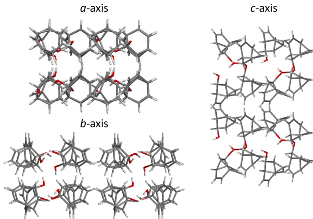
Figure S58. Solid-state superstructure of ( R )/( S )- 1 viewed along the three unit cell axes.
