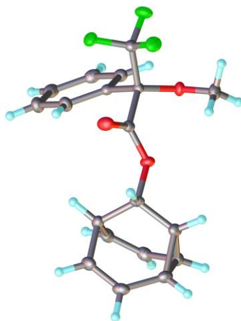
Figure S59. Solid-state structure of ( S,S )- 2 including probability ellipsoids at 50%.
