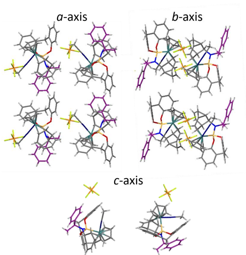
Figure S76. Solid-state superstructure of (C,R,S)\text{-L}_{\text{BB}}\text{RuCp}(\text{NCMe})\cdot\text{PF}_6 viewed along the three unit cell axes.
