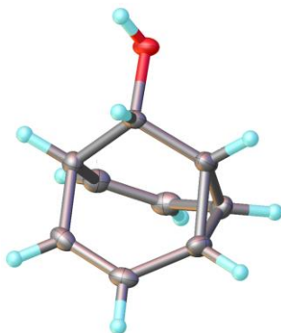
Figure S57. Solid-state structure of ( R )/( S )-1 including probability ellipsoids at 50%.
