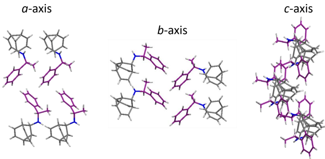
Figure S71. Solid-state superstructure of ( R,S )- 5 viewed along the three unit cell axes.
