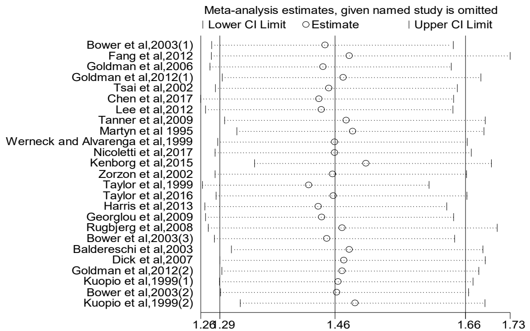
S1 Fig.sensitivity analysis of head injury and PD risk
