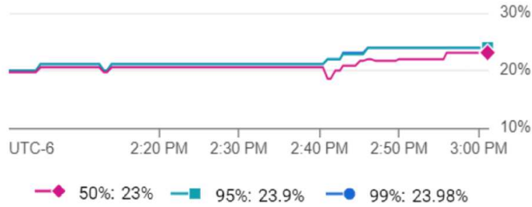
Fig. 5 CPU Utilization for Google Cloud Run.
