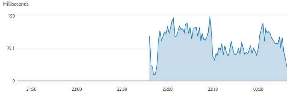
Fig. 3 Request Latency for AWS App Runner.
