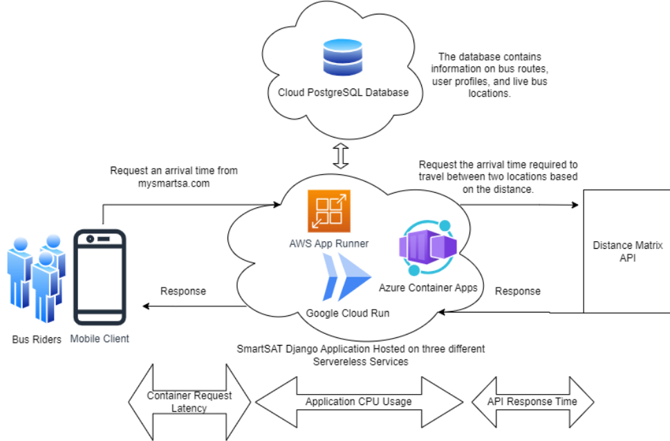
Fig. 1 Visual representation of the concepts of Request Latency, CPU Usage, and API Response Time.
