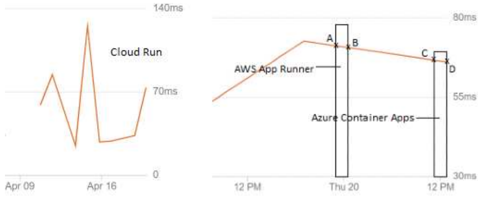
Fig. 4 Response Time for Google Cloud Run, AWS App Runner, and Azure Container Apps (A=71.66, B=71.11, C=67.22, D=66.38).
