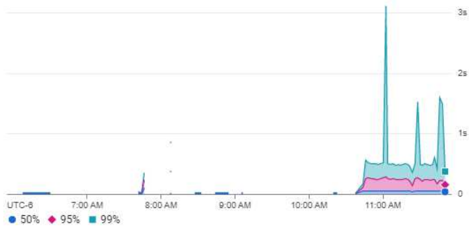
Fig. 2 Request Latency for Google Cloud Run.
