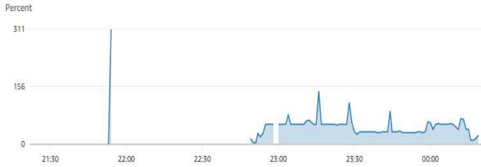
Fig. 6 CPU Utilization for AWS App Runner.
