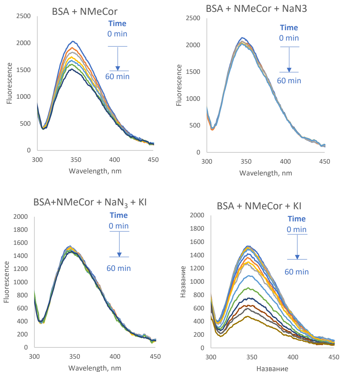
Figure S6. Corrected fluorescence spectra upon irradiation of a complex of BSA (0.08 wt %) with NMeCor ( 1.7 \cdot 10^{-5} M) depending on the presence of KI (50 mM) and NaN 3 (15 mM).
