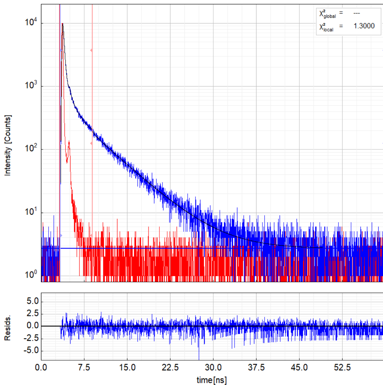
Figure S3. Fluorescence decay rate of NMeCor in Tris-HCl buffer.
