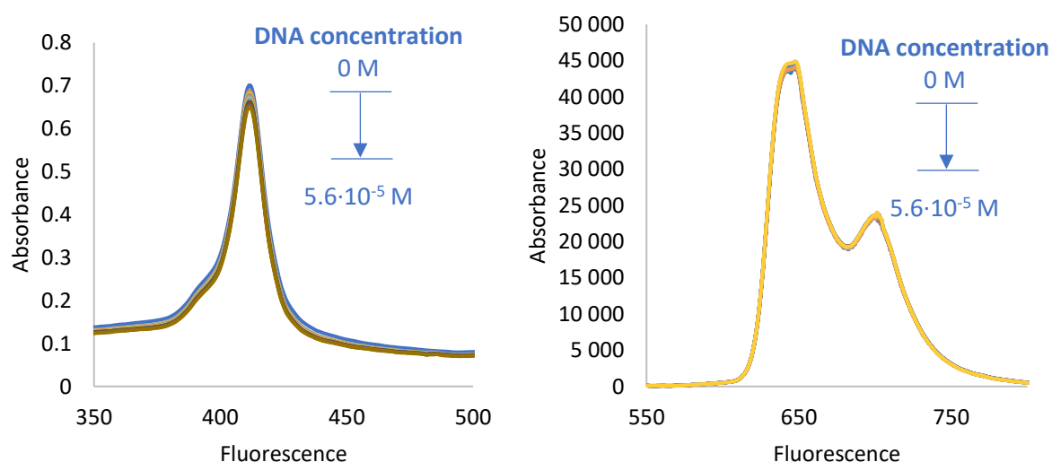
Figure S1. UV-Vis and fluorescence ( \lambda_{\text{ex}}=425 nm) spectra of pSCor during titration with DNA. Titration was performed by adding DNA (1.6 mM) 10 \mu\text{l} (7 steps) to 2 ml of corrole solution in Tris-HCl buffer in a cuvette with stirring at a temperature of 25^\circ\text{C} .
