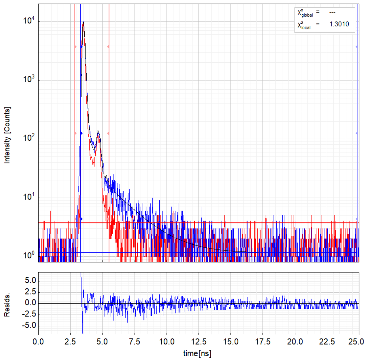
Figure S4. Fluorescence decay rate of complex NMeCor with DNA in Tris-HCl buffer.
