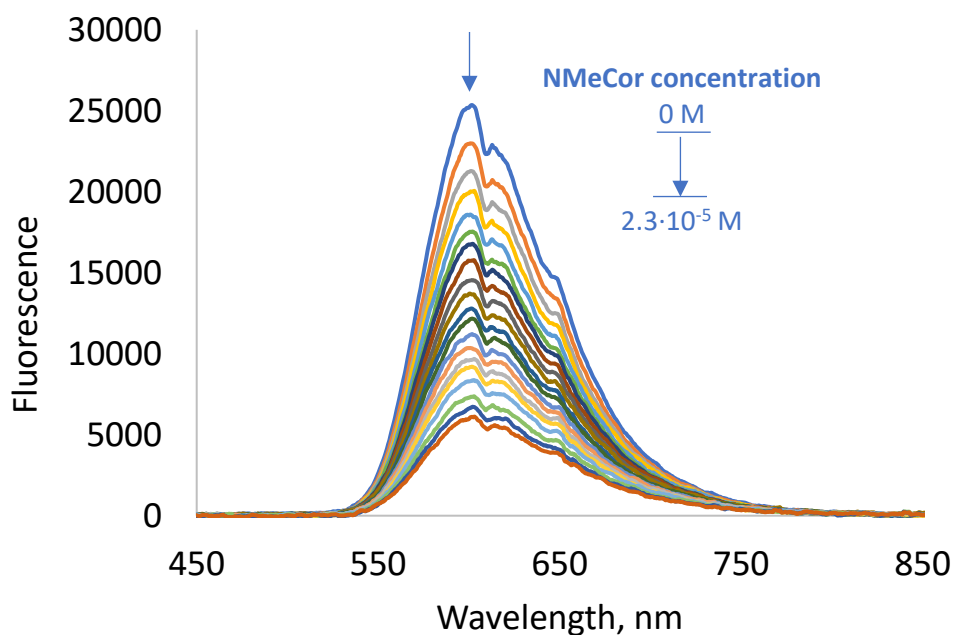
Figure S2. Fluorescence spectra ( \lambda_{\text{ex}}=295 nm) of titration of DNA ( 1.1 \cdot 10^{-4} M)-EtBr ( 1.3 \cdot 10^{-5} M) complex with NMeCor . Titration was performed by adding of NMeCor (0.45 mM) 5 \mu l (19 steps) to 2 ml of DNA-EtBr complex in Tris-HCl buffer in a cuvette with stirring at a temperature of 25 °C.
