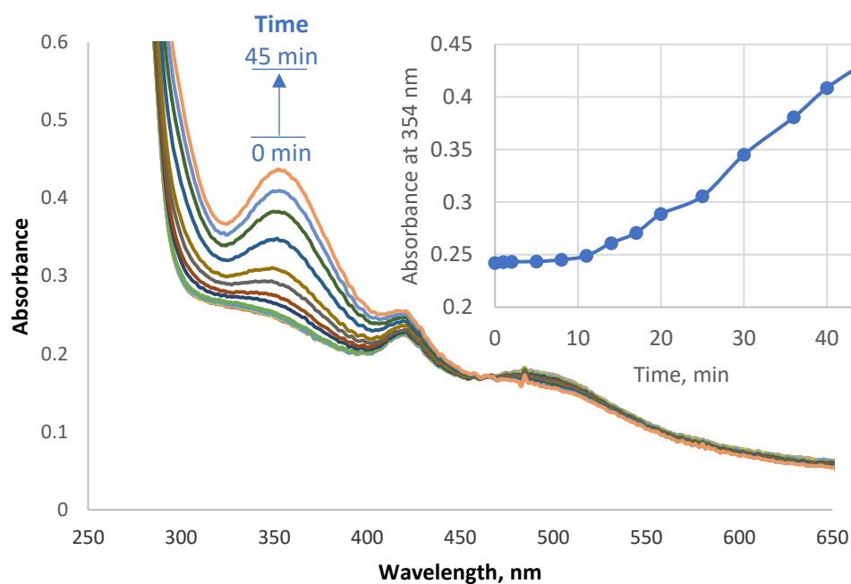
Figure S8. UV-Vis spectra of solution of BSA (0.08 wt %) with NMeCor ( 1.7 \cdot 10^{-5} M) and KI (50 mM) in PBS irradiated with light 425 nm. Absorbance at 354 nm on inset.
