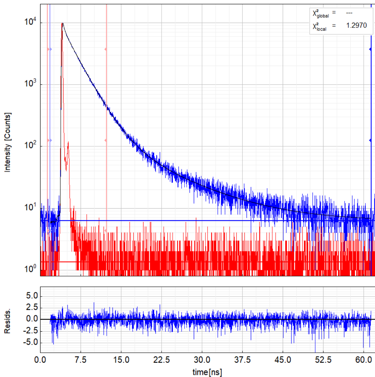
Figure S5. Fluorescence decay rate of pSCor in Tris-HCl buffer.
