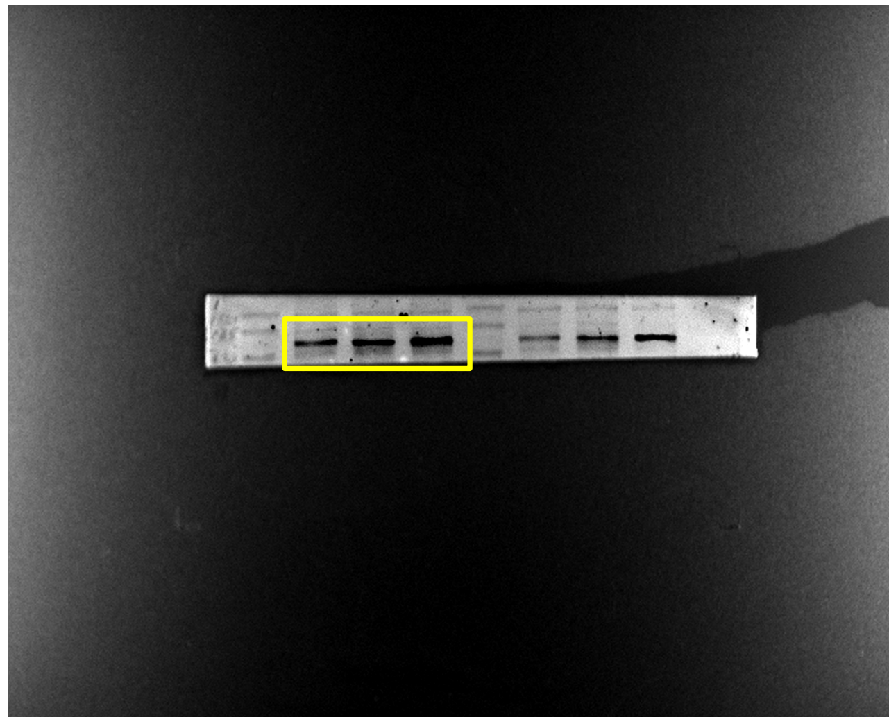
Nrf2-125KD
