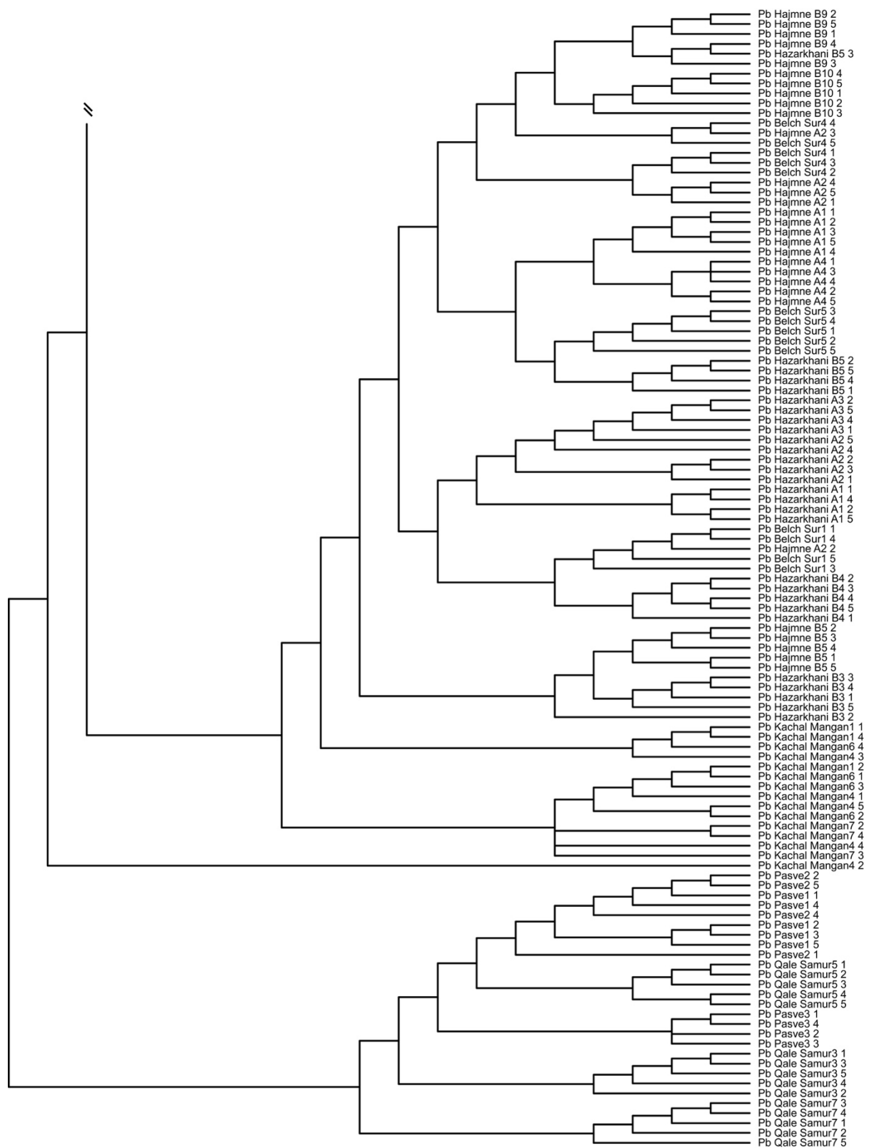
Figure S3. Strict consensus derived from 120 MP trees resulting from the parsimony analysis of the GBS dataset, including 244 P. bracteatum individuals.
