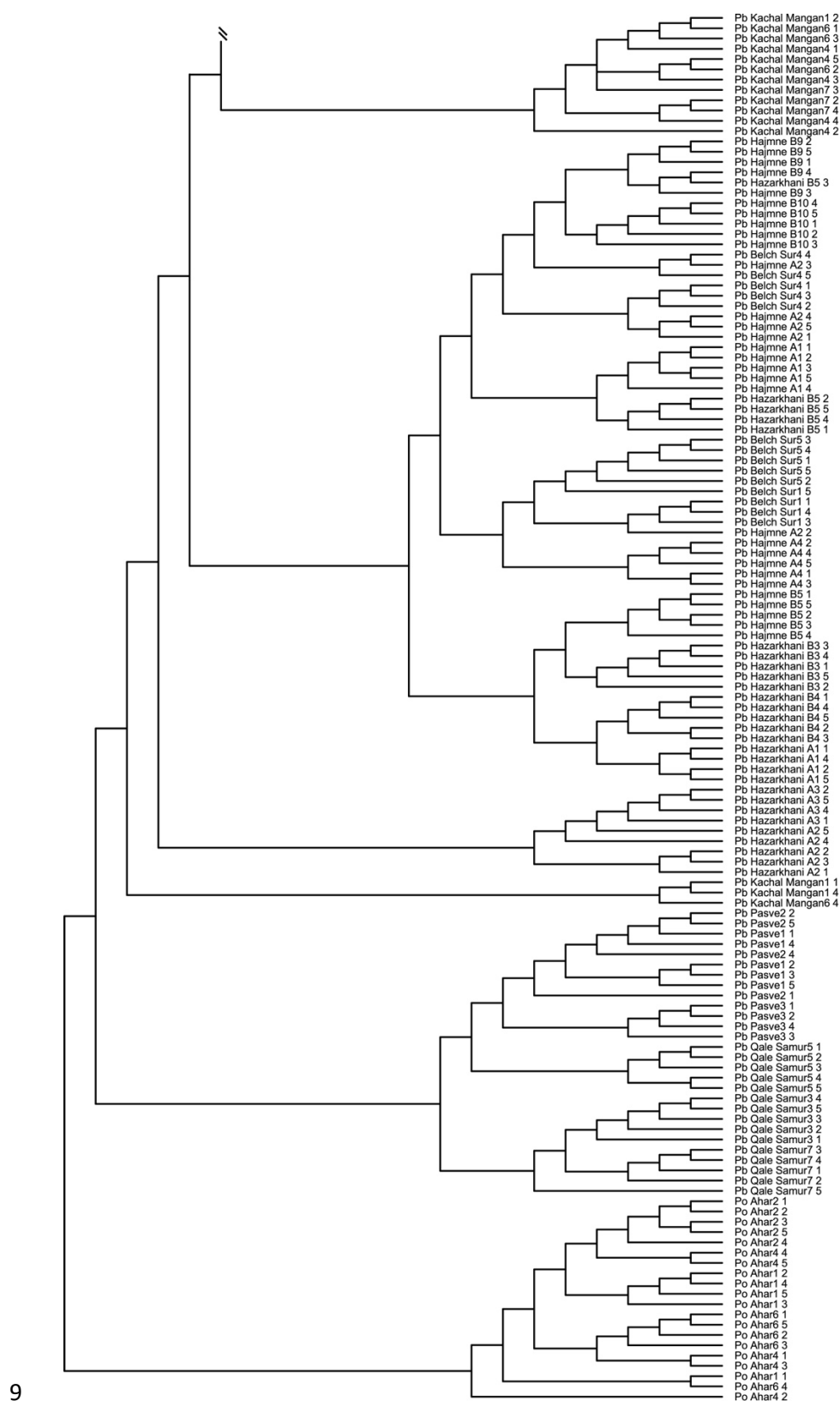
Figure S2. Strict consensus derived from 80 MP trees resulting from the parsimony analysis of the GBS dataset, including 264 individuals of P. orientale (Po; outgroup) and P. bracteatum (Pb).
