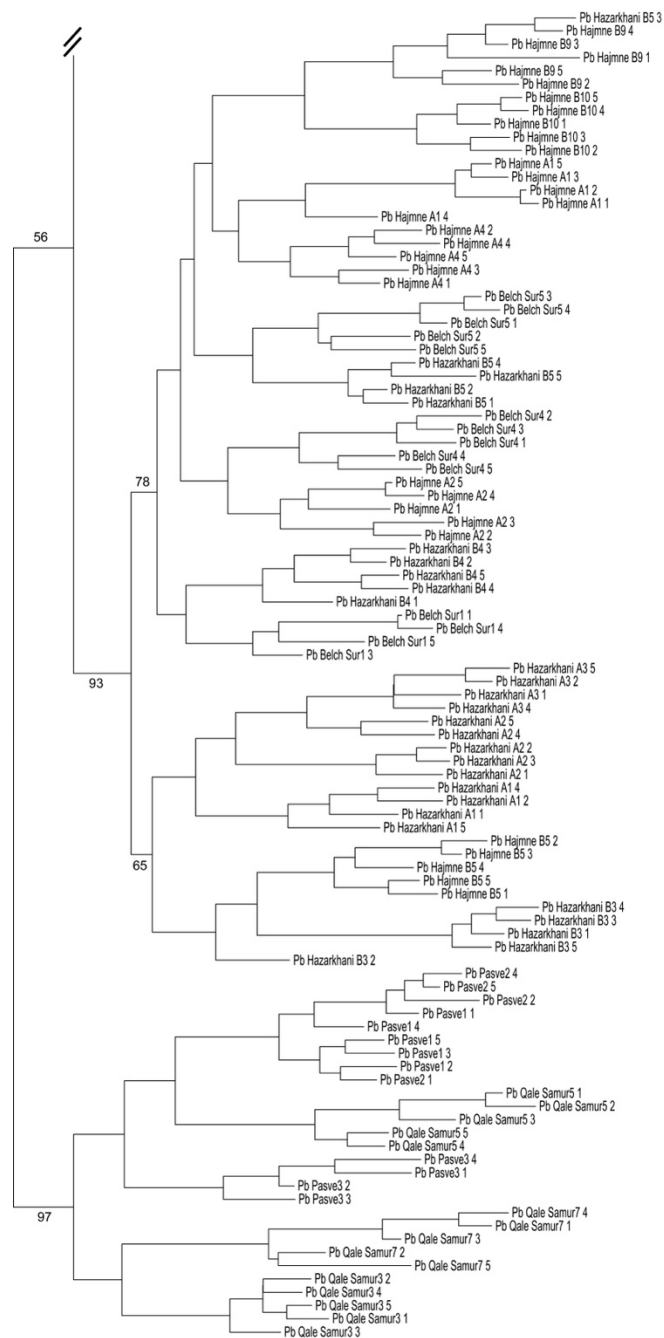
Figure S4. Maximum-likelihood tree for the GBS dataset excluding P. orientale . Numbers along branches on the backbone of the tree depict bootstrap support values (≥50%).
