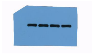
Figure 6c GLUT4
