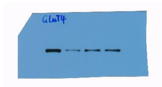
Figure 6c GLUT4
