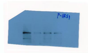
Figure 6a p-IRS1
