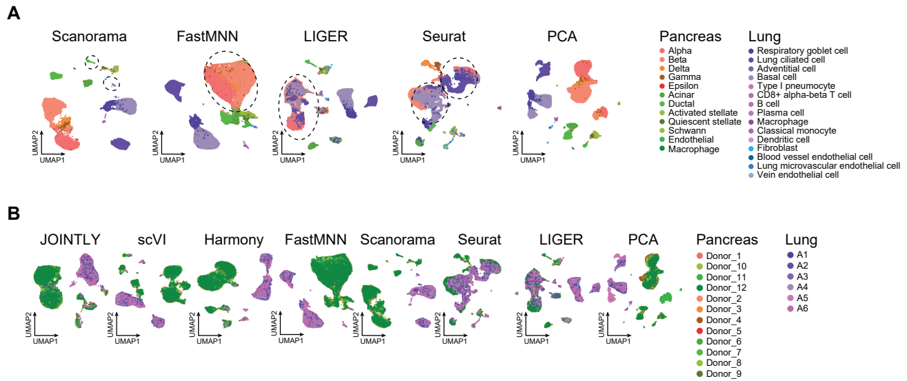
Supplementary Figure 3: A) UMAPs of integration of pancreas and lung tissue (Scanorama, fastMNN, LIGER, Seurat and PCA, from left) superimposed with cell type information. B) UMAPs showing donor labels for the indicated methods.
