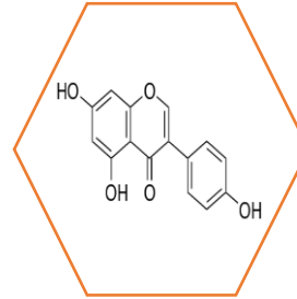
Flavonoids
