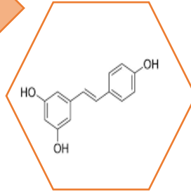
Polyphenols
