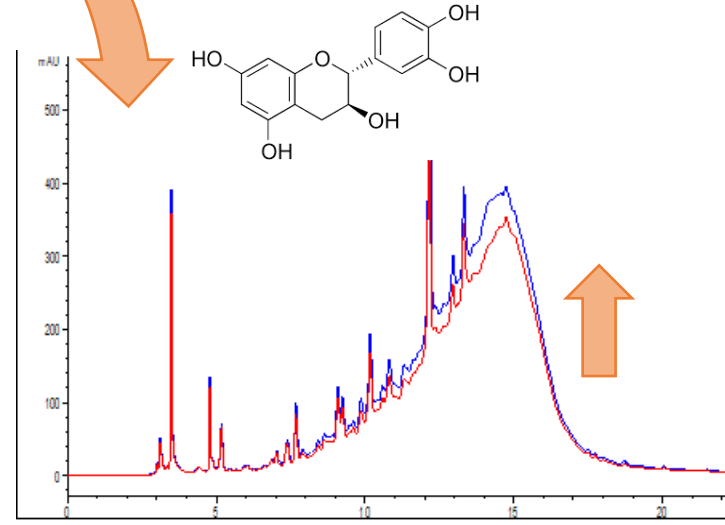
Flavonoids
