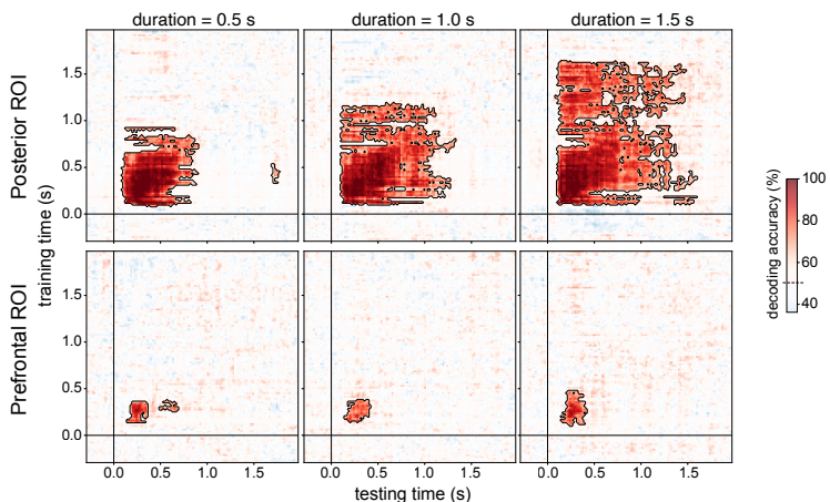
f iEEG cross-task decoding of category (face/object) using pseudotrials (train irrelevant, test relevant)
