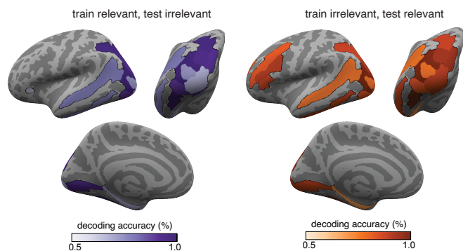
g iEEG cross-task decoding of category (face/object) using pseudotrials
