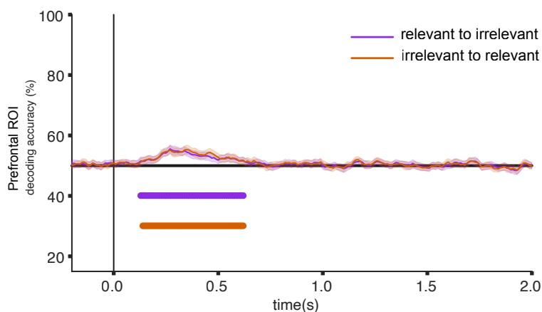
e iEEG cross-task decoding of category (face/object) (train relevant, test irrelevant)
