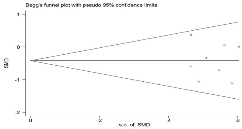
Figure S3. Begg's test for evaluating publication bias.
