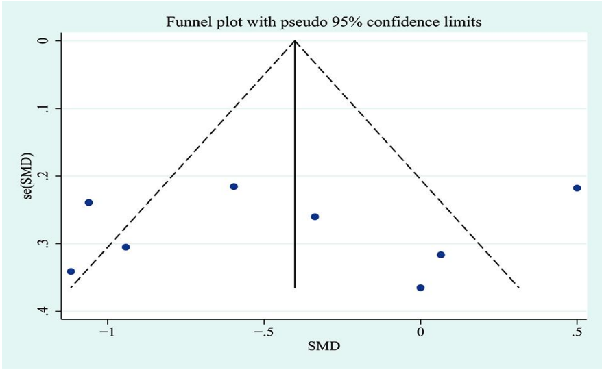
Figure S2. Funnel plot evaluating publication bias
