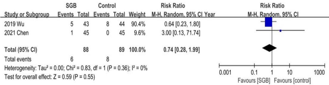
Figure S1 Forest plot for PONV within 24h after surgery.
