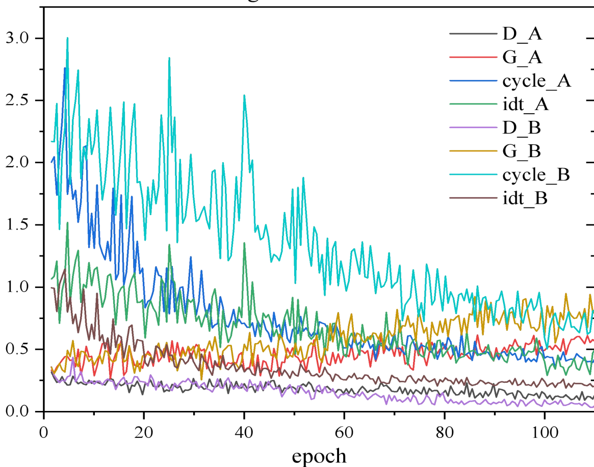
Training loss of Bmode-GAN
