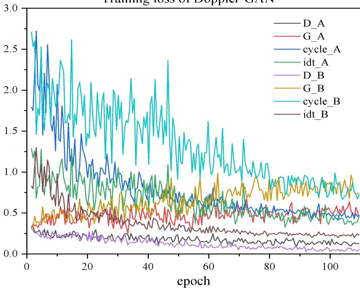
Training loss of Doppler-GAN
