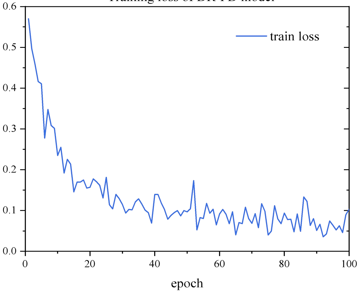
Training loss of DR-FD model
