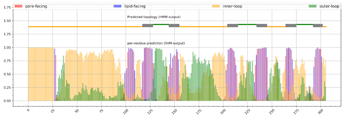
Figure 1 : OipA Topology Modeling
