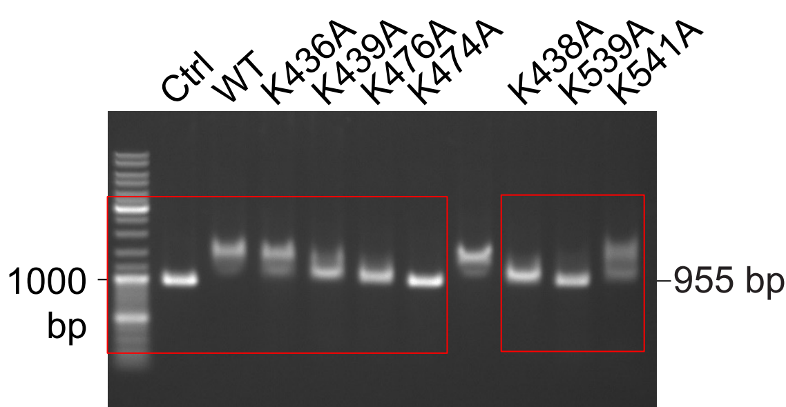
Extended Data Fig. 5h Binding of pUC19-955 DNA
