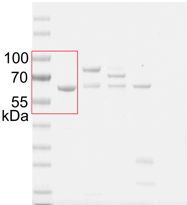
Extended Data Fig. 8t Co-purification of GajA and GajB-Q155A/Y347A
