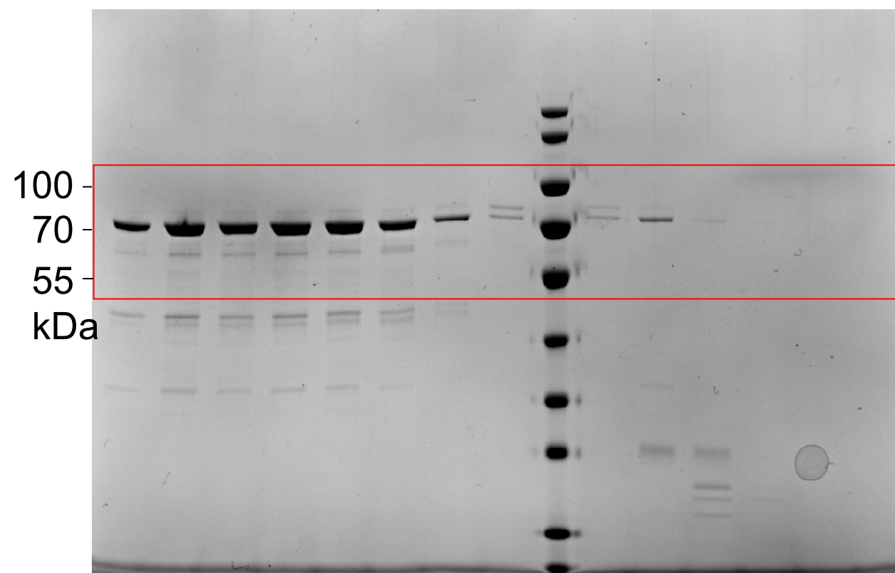
Extended Data Fig. 4c Cleavage of synthetic dsDNA
