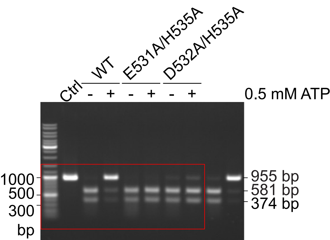
Extended Data Fig. 10m Cleavage of pUC19-955 DNA
