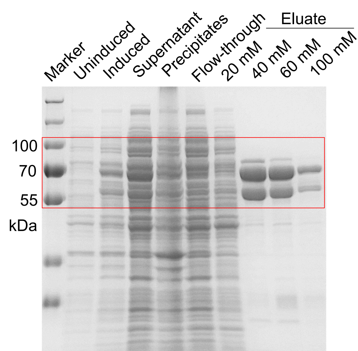
Extended Data Fig. 8s Co-purification of GajA and GajB
