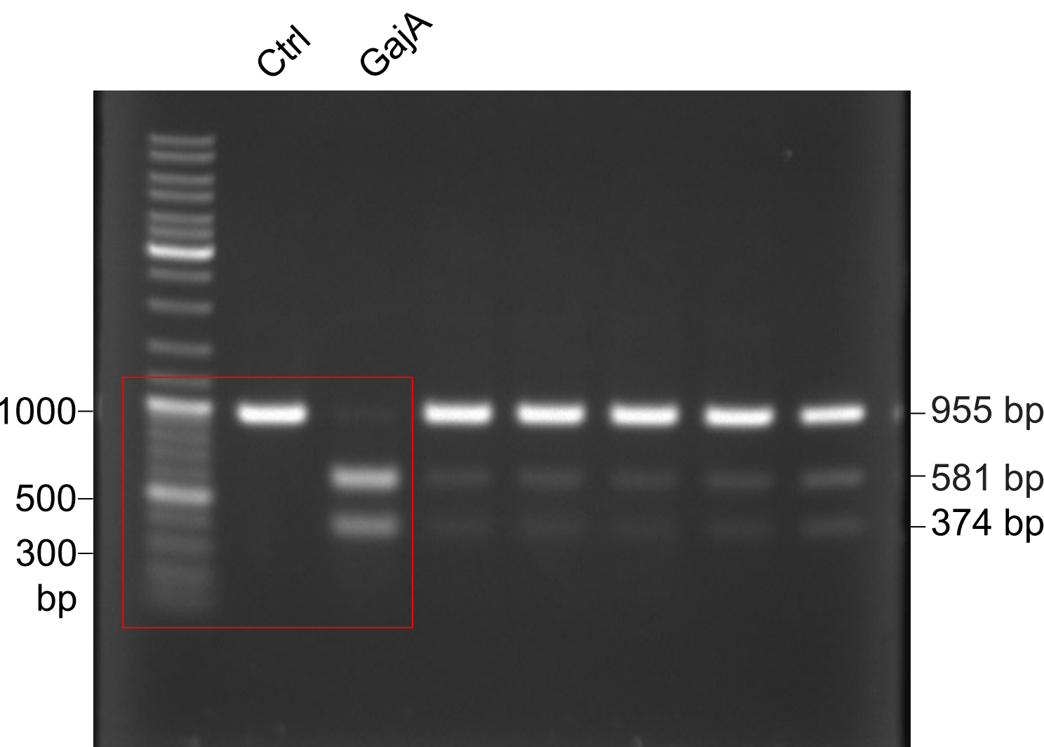
Extended Data Fig. 1e Cleavage of pUC19-955 DNA
