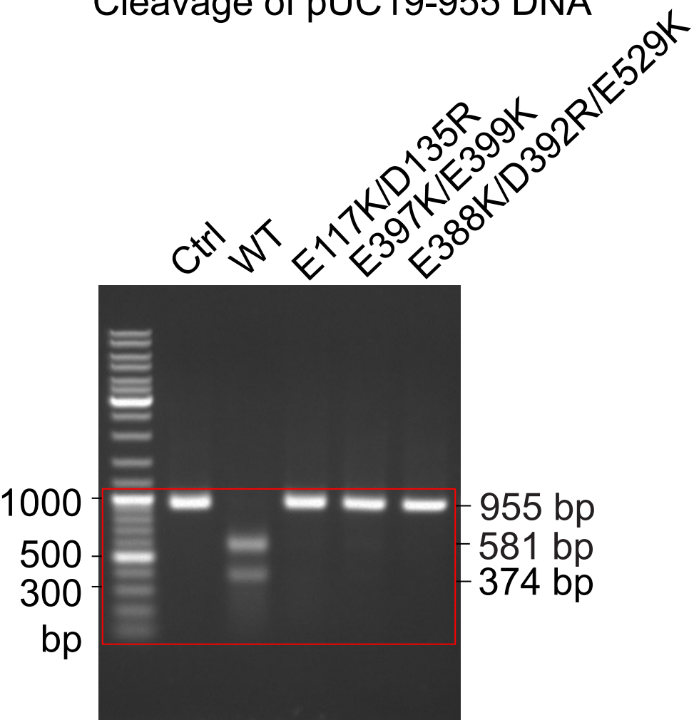
Extended Data Fig. 3e Cleavage of pUC19-955 DNA
