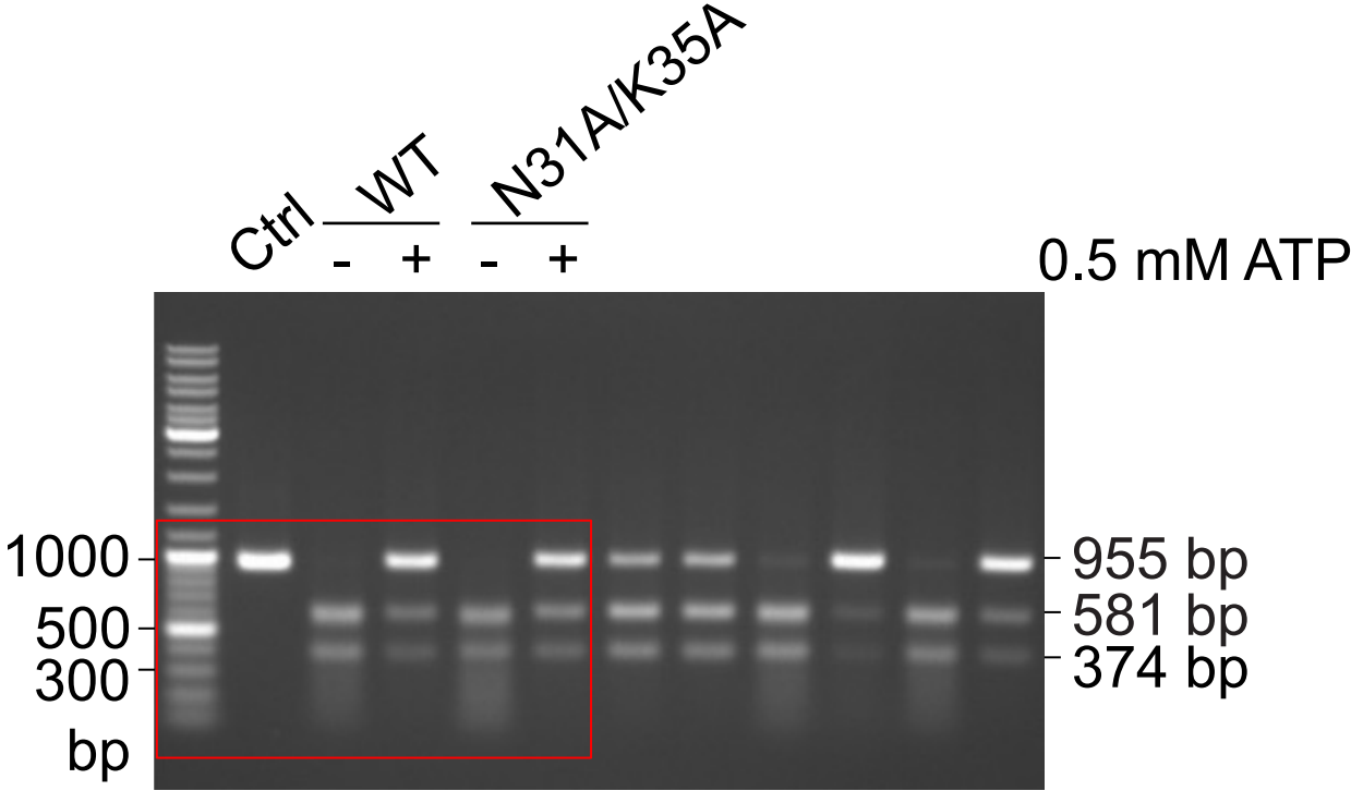
Extended Data Fig. 10i Cleavage of pUC19-955 DNA
