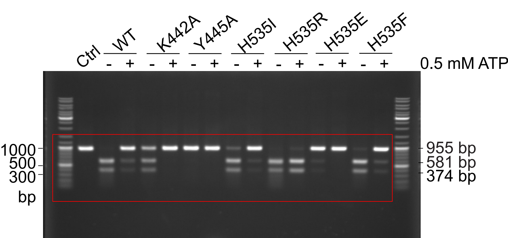
Fig. 4l Cleavage of pUC19-955 DNA
