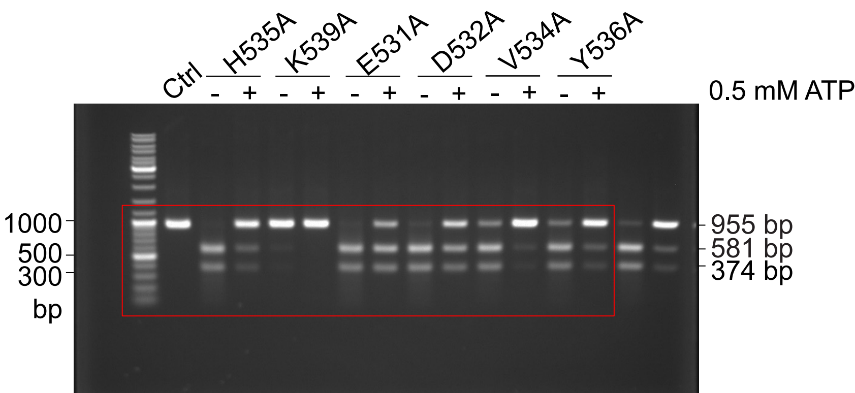
Fig. 4k Cleavage of pUC19-955 DNA
