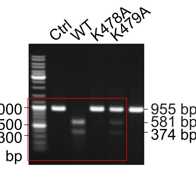
Extended Data Fig. 5b Cleavage of pUC19-955 DNA
