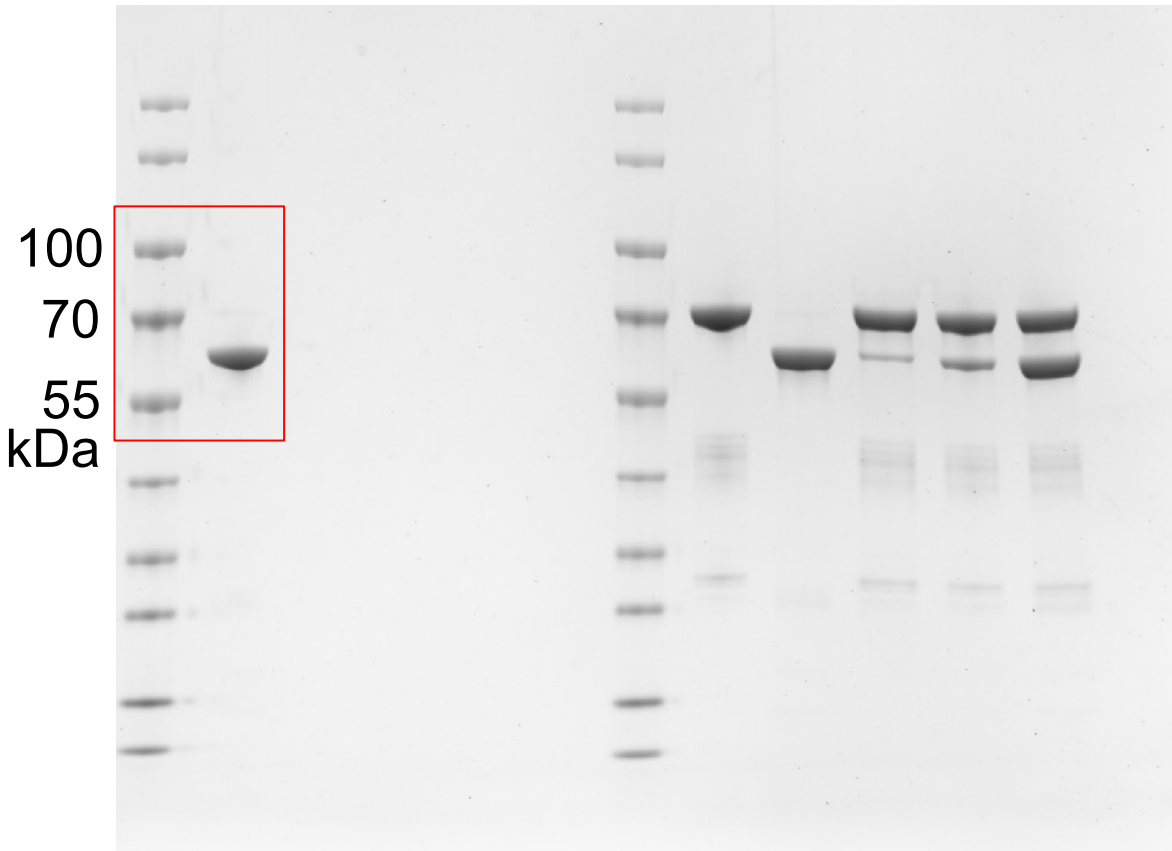
Extended Data Fig. 8l SDS-PAGE of GajA and GajB
