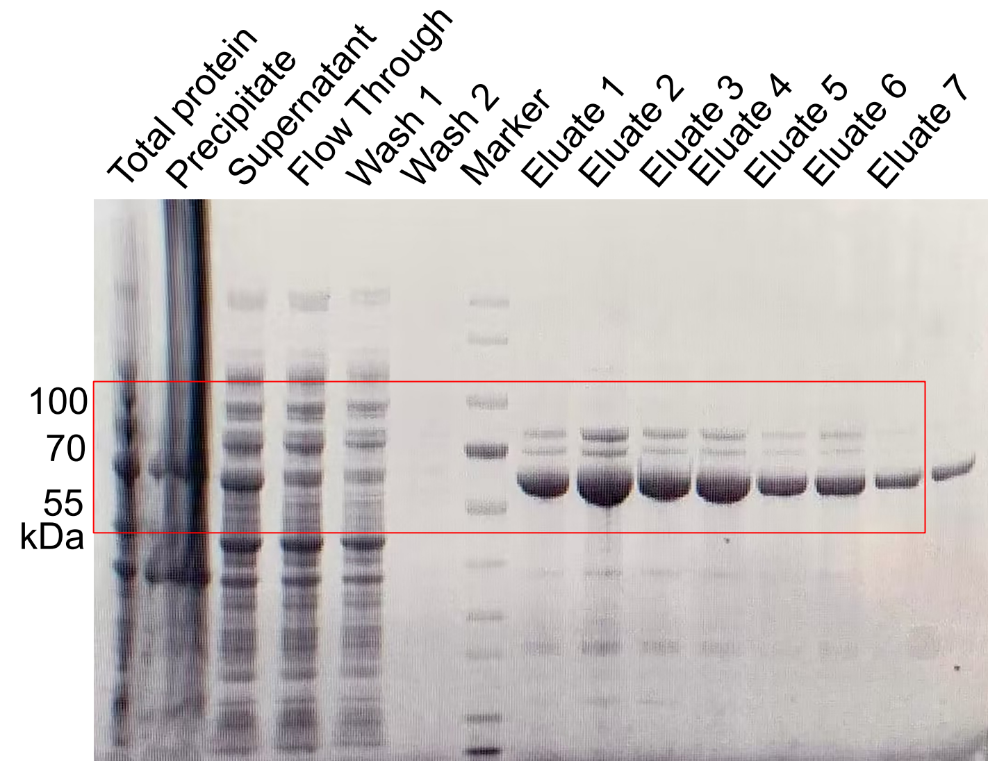
Extended Data Fig. 8o Purification of GajB-Q155A/Y347A
