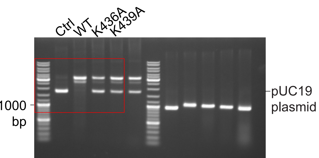
Extended Data Fig. 5f Cleavage of pUC19 plasmid
