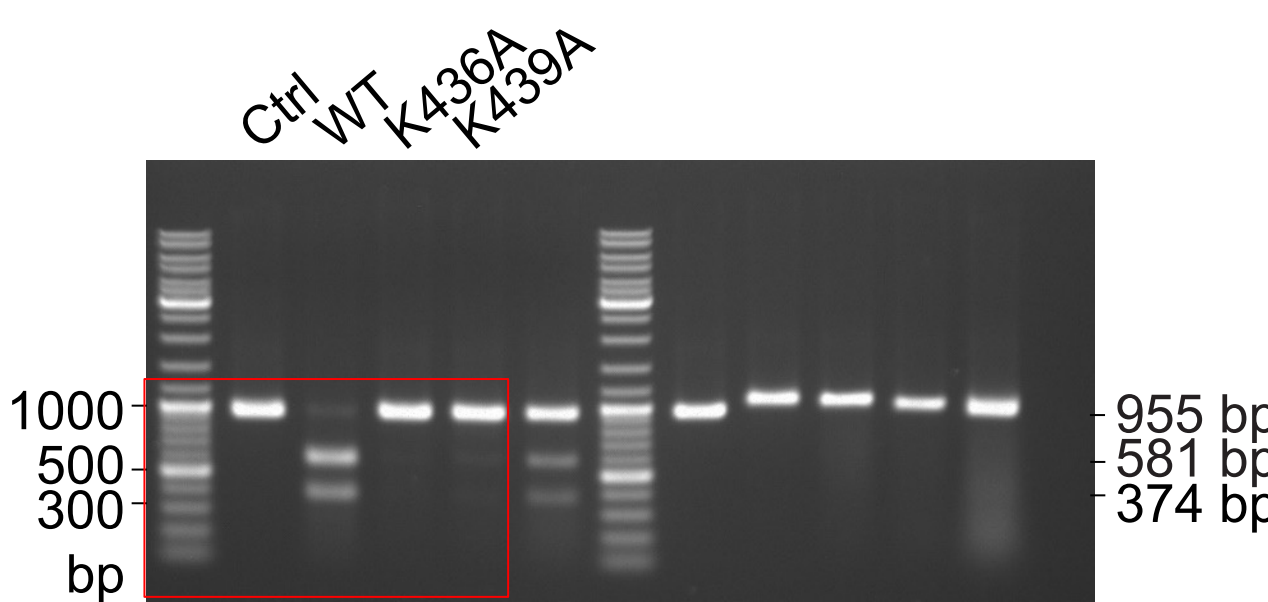
Extended Data Fig. 5e Cleavage of pUC19-955 DNA
