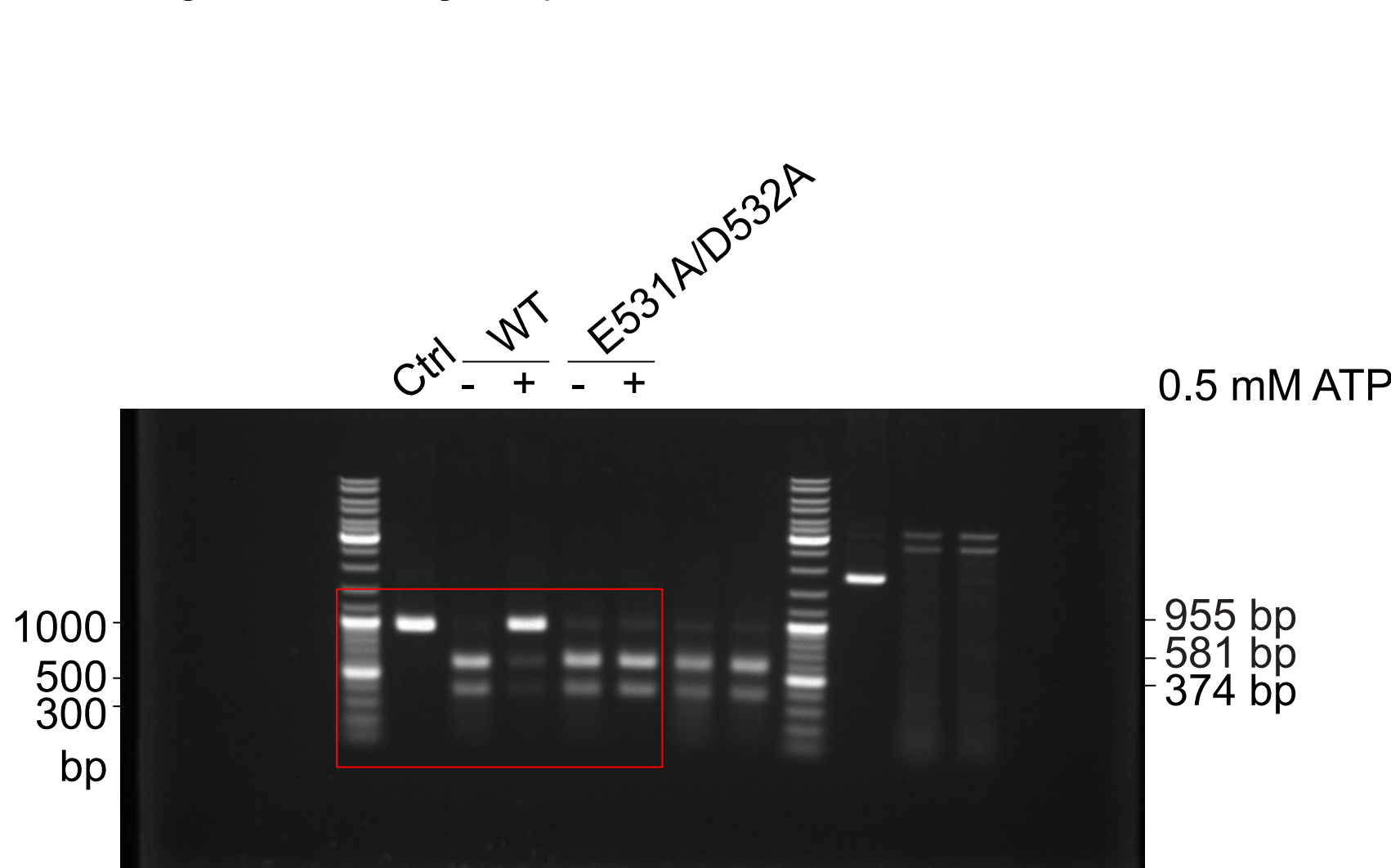
Fig. 4m Cleavage of pUC19-955 DNA
