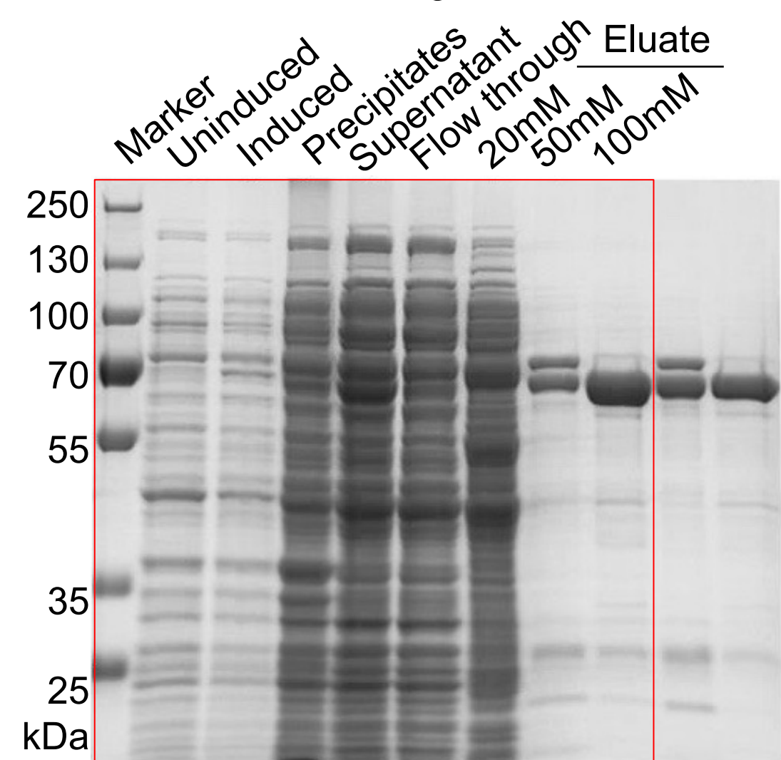
Extended Data Fig. 1a Purification of GajA
