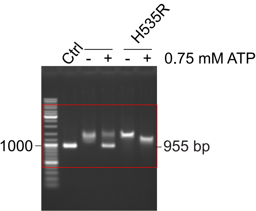
Extended Data Fig. 10n Binding of pUC19-955 DNA
