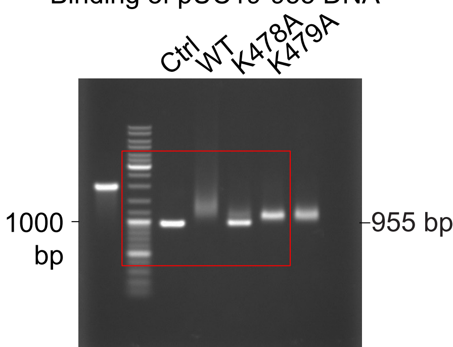
Extended Data Fig. 5g Binding of pUC19-955 DNA
