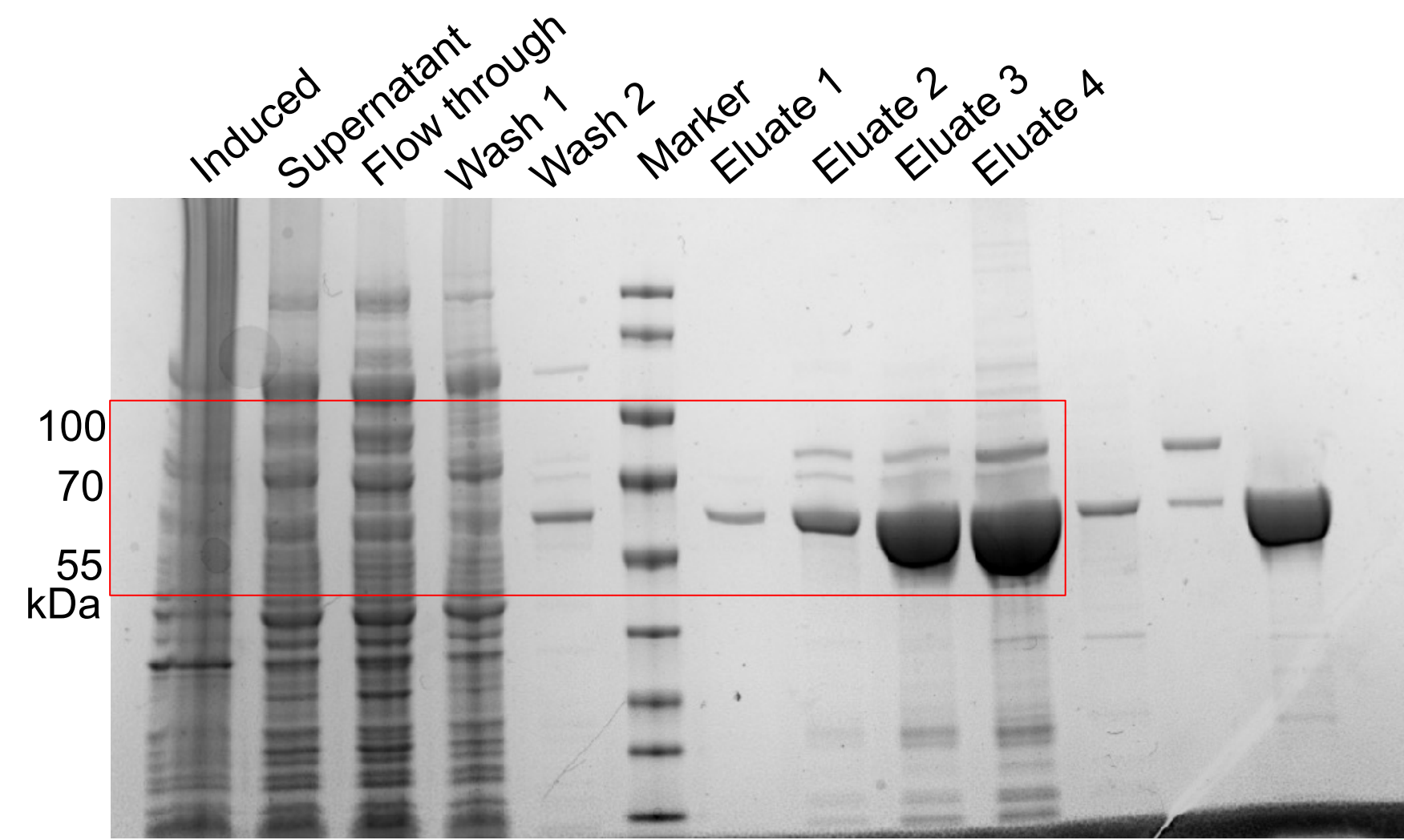
Extended Data Fig. 8a Purification of GajB
