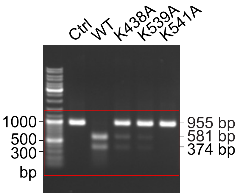
Extended Data Fig. 5d Cleavage of pUC19-955 DNA
