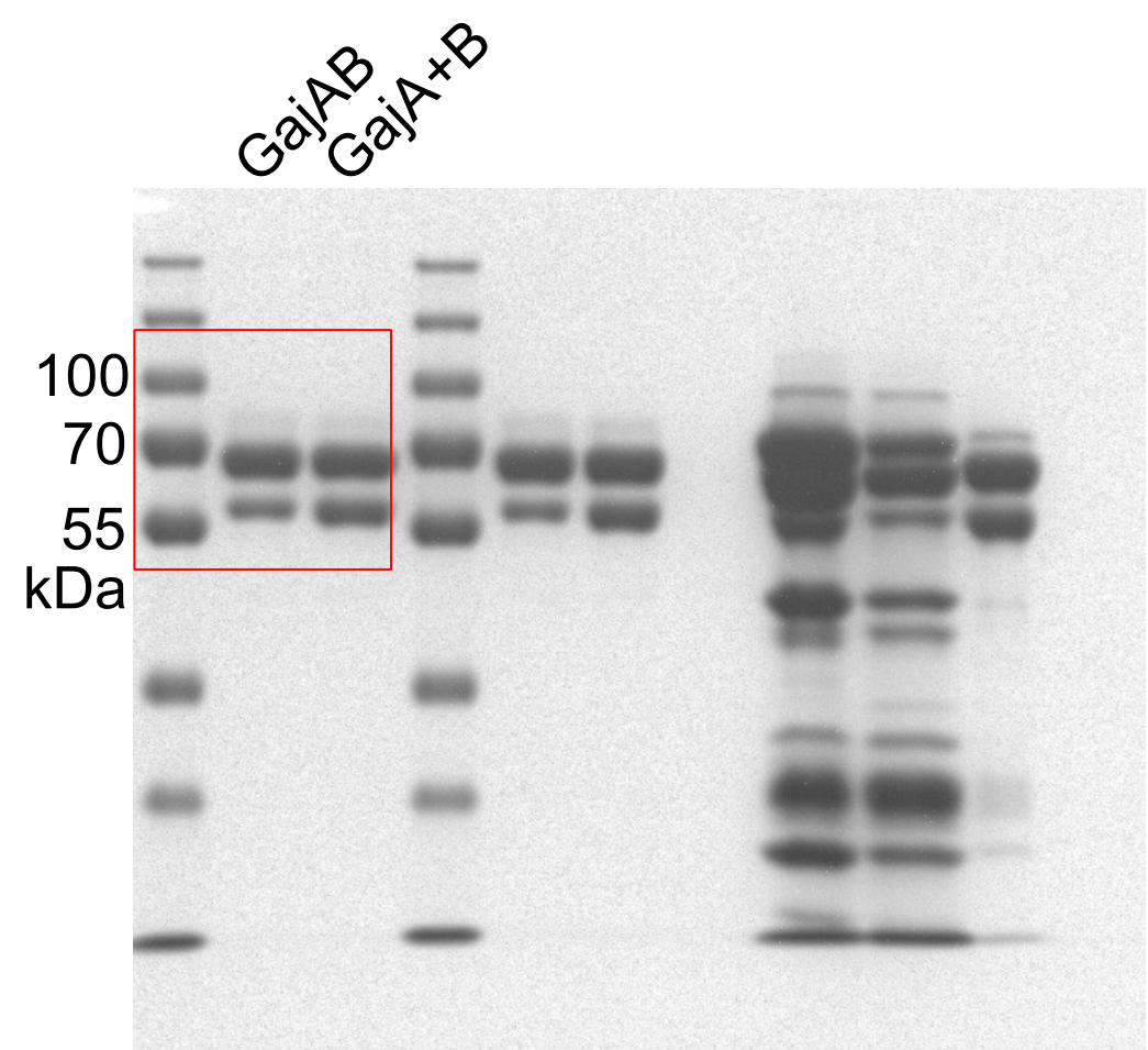
Extended Data Fig. 8l SDS-PAGE of GajA and GajB
