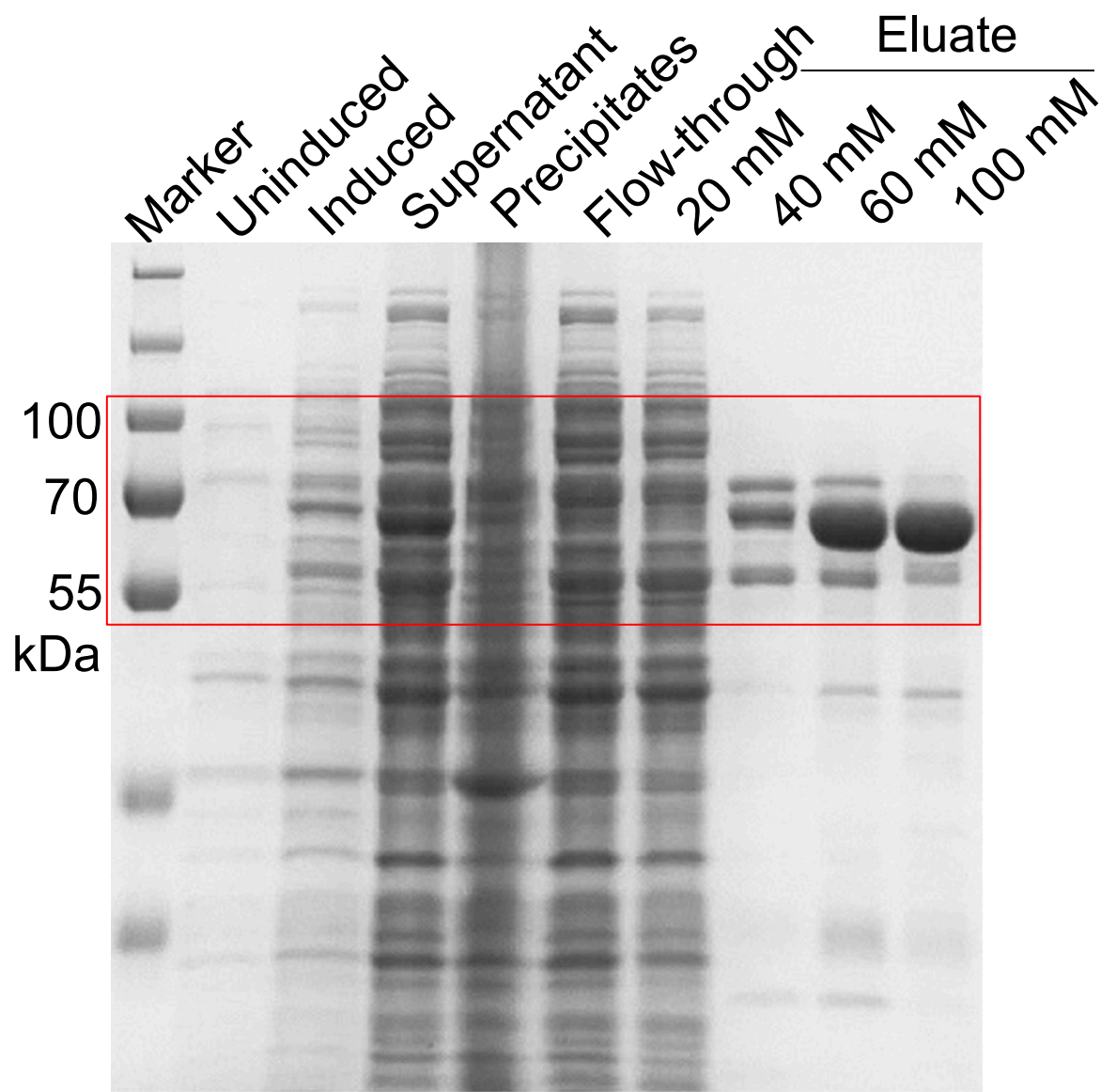
Extended Data Fig. 8t Co-purification of GajA and GajB-Q155A/Y347A
