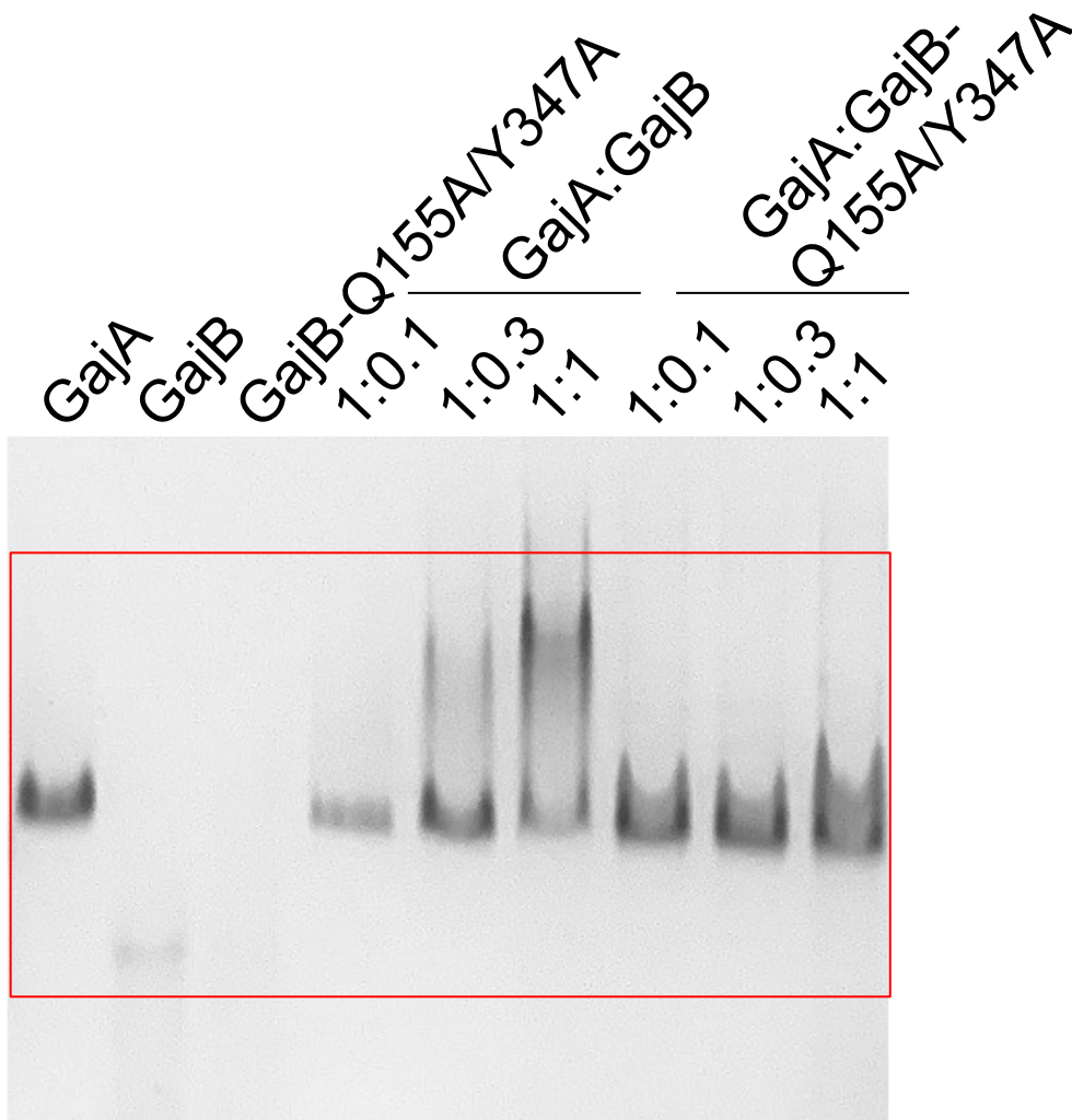
Extended Data Fig. 8t Co-purification of GajA and GajB-Q155A/Y347A
