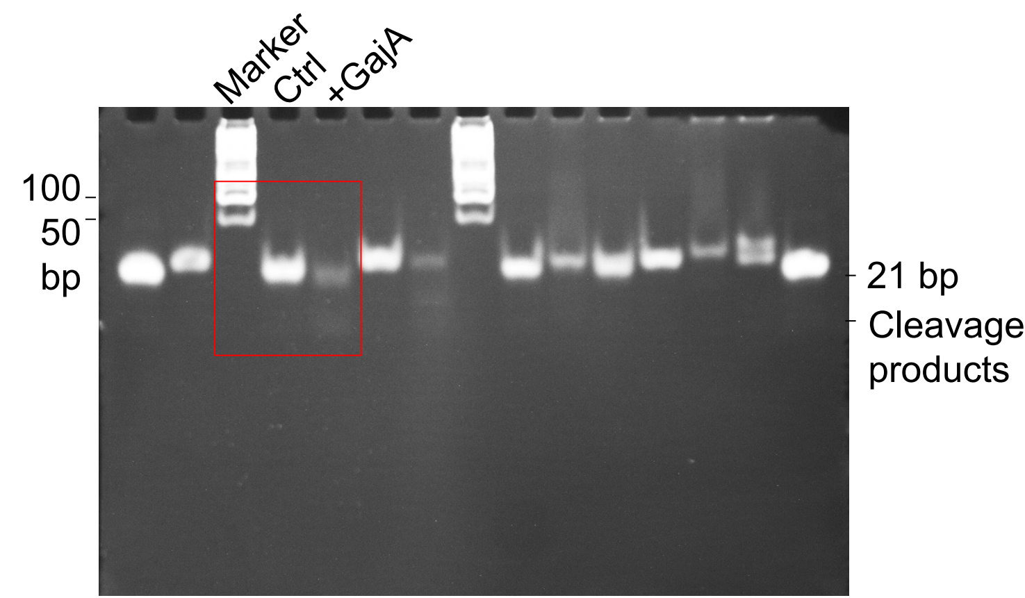
Fig. 2b Cleavage of 21-bp dsDNA
