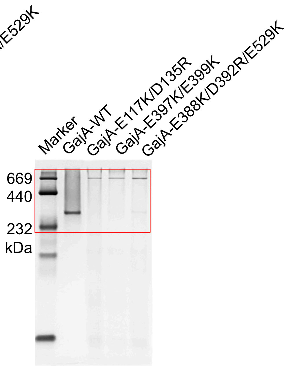
Extended Data Fig. 3c Native PAGE
