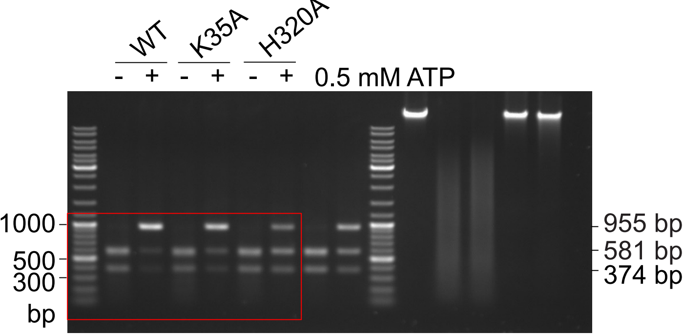
Extended Data Fig. 10g Cleavage of pUC19-955 DNA
