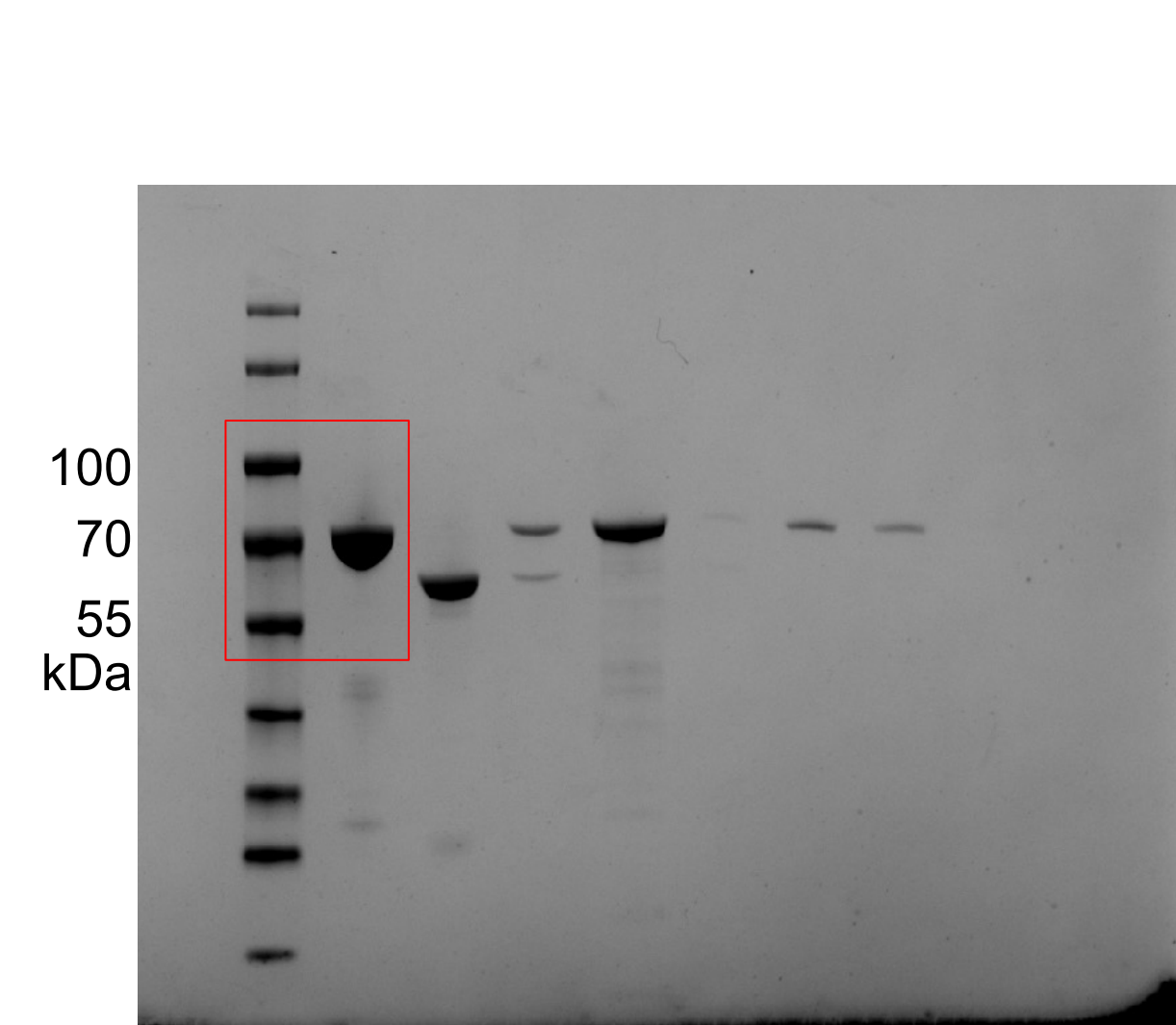
Extended Data Fig. 1c SDS-PAGE of GajA
