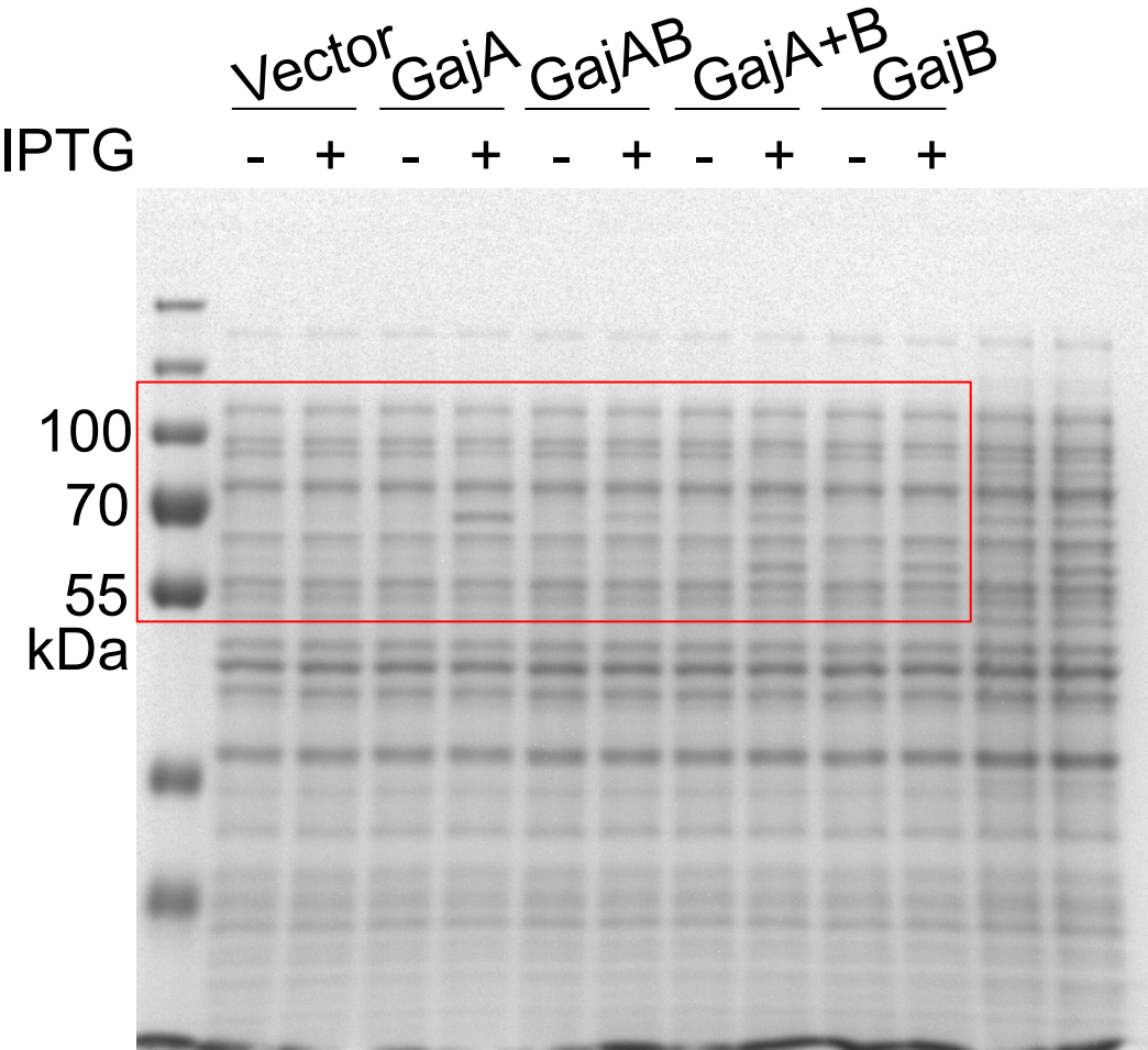
Extended Data Fig. 8k Expression of GajA and GajB
