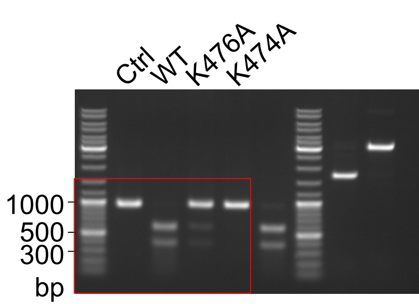
Extended Data Fig. 5c Cleavage of pUC19-955 DNA
