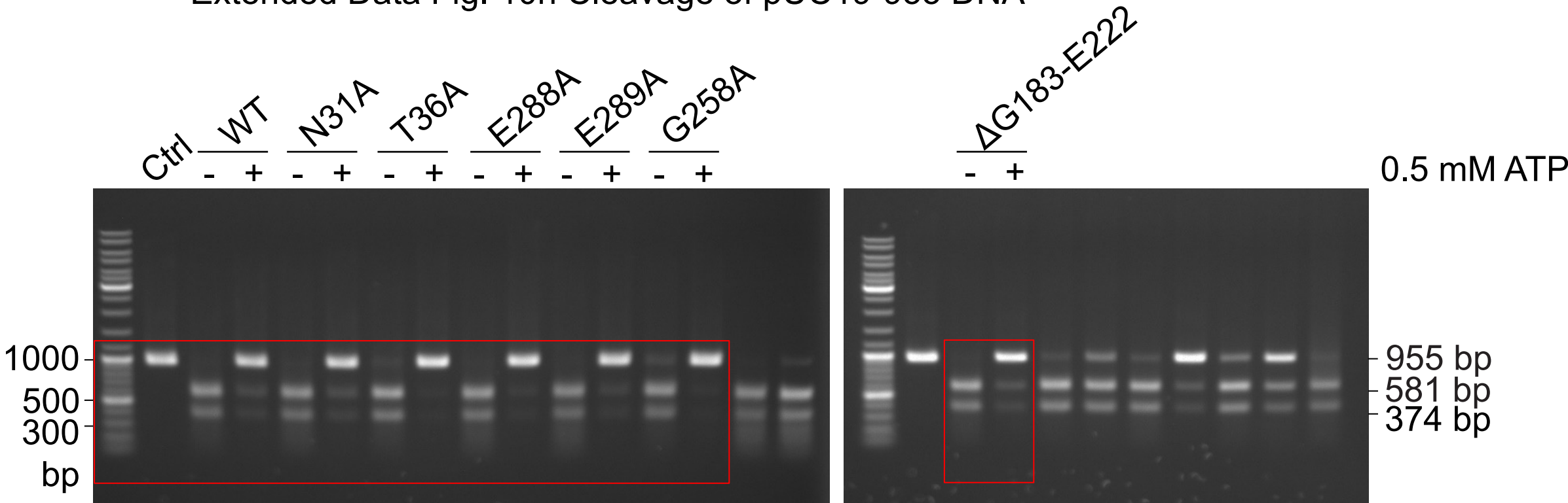
Extended Data Fig. 10h Cleavage of pUC19-955 DNA
