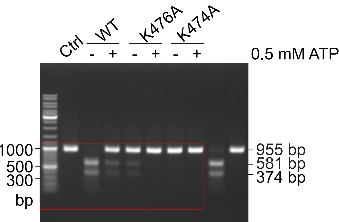
Extended Data Fig. 10j Cleavage of pUC19-955 DNA
