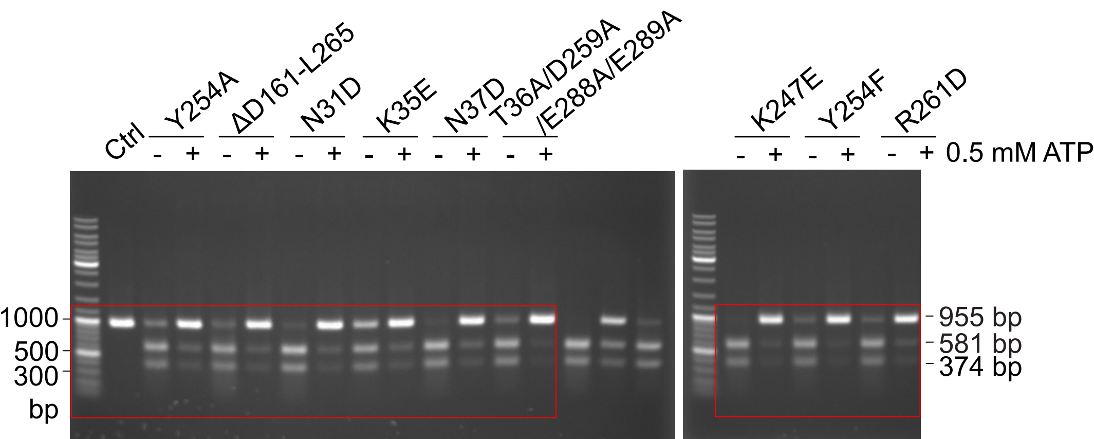
Extended Data Fig. 10k Cleavage of pUC19-955 DNA
