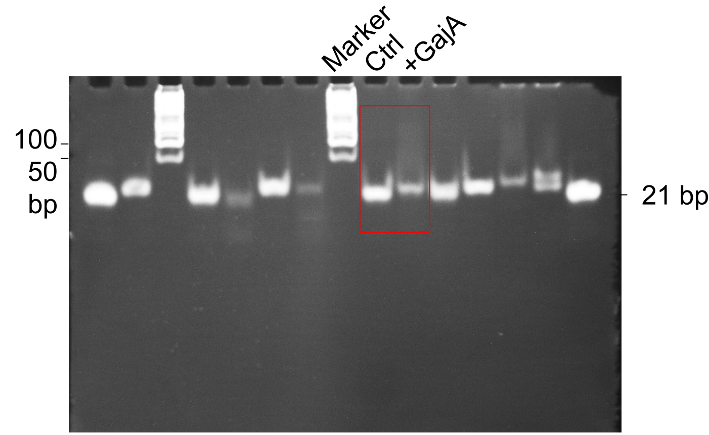
Fig. 2c Binding of 21-bp dsDNA
