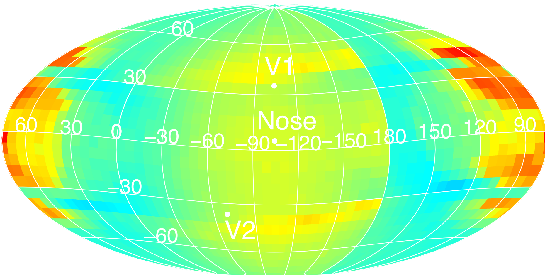
a ESA 3, t_{\text{IBEX}} = 2009\text{-}2011
