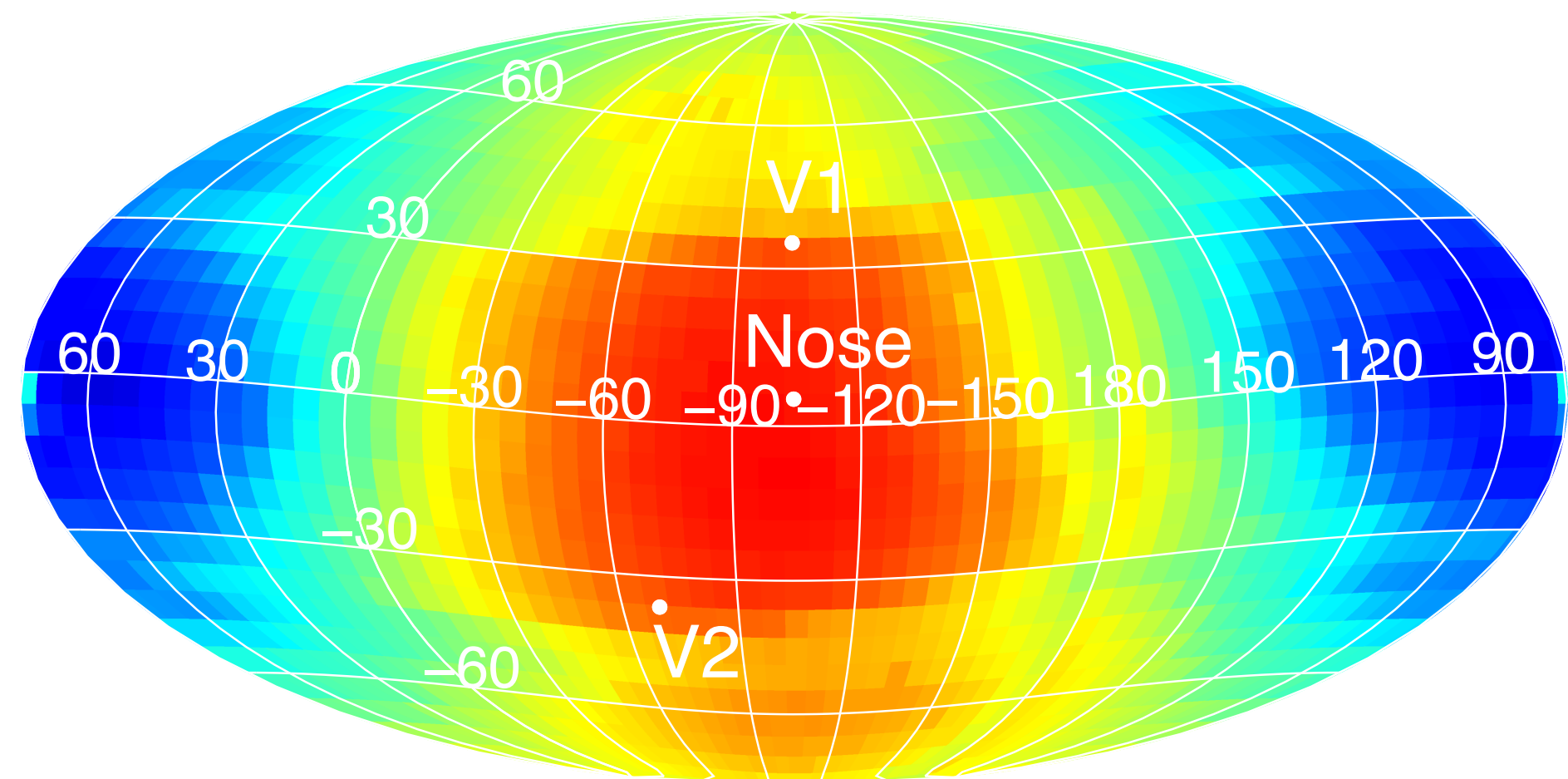
b ESA 3, t_{\text{IBEX}} = 2014\text{-}2016
