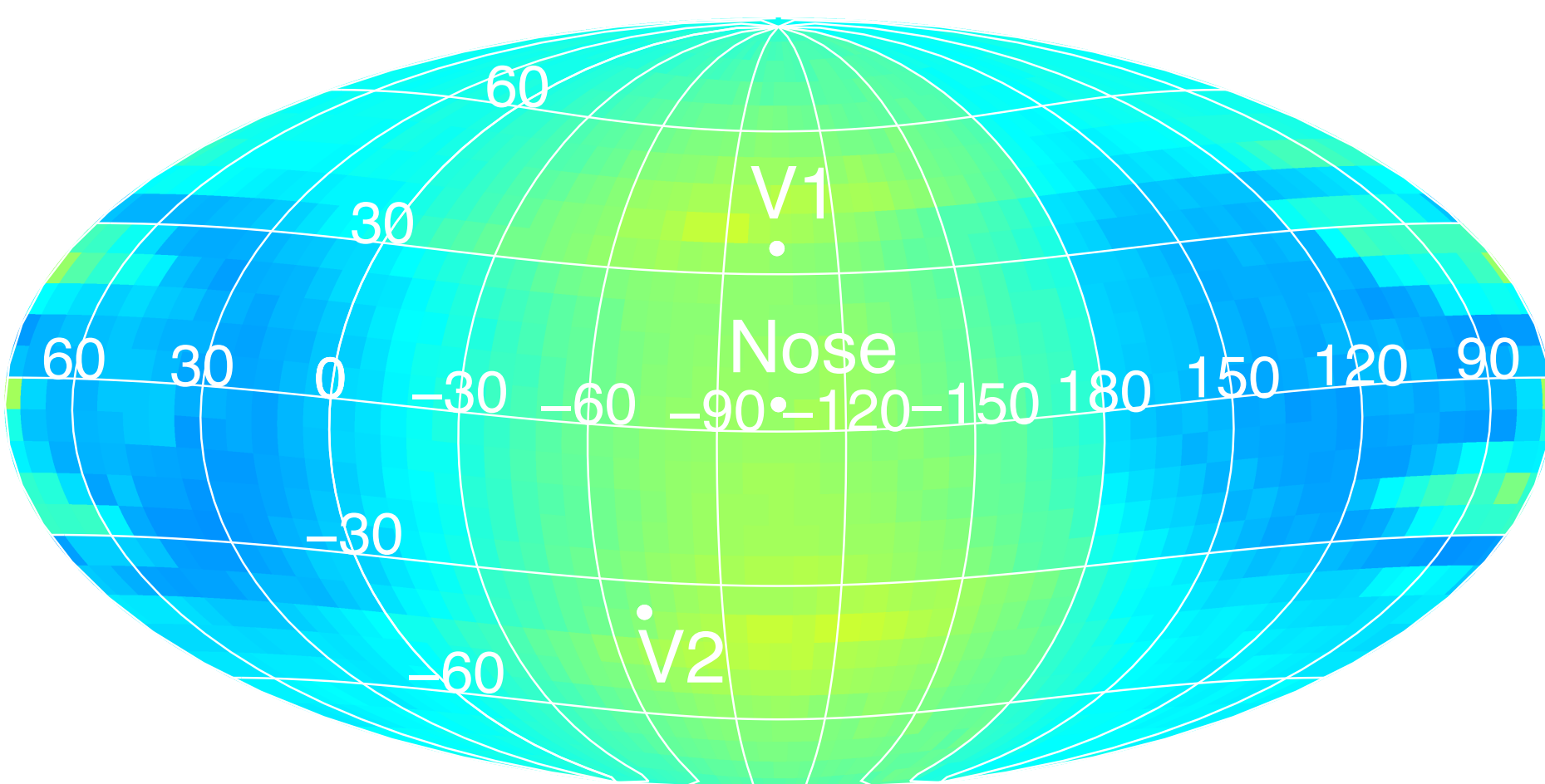
c ESA 6, t_{\text{IBEX}} = 2009\text{-}2011
