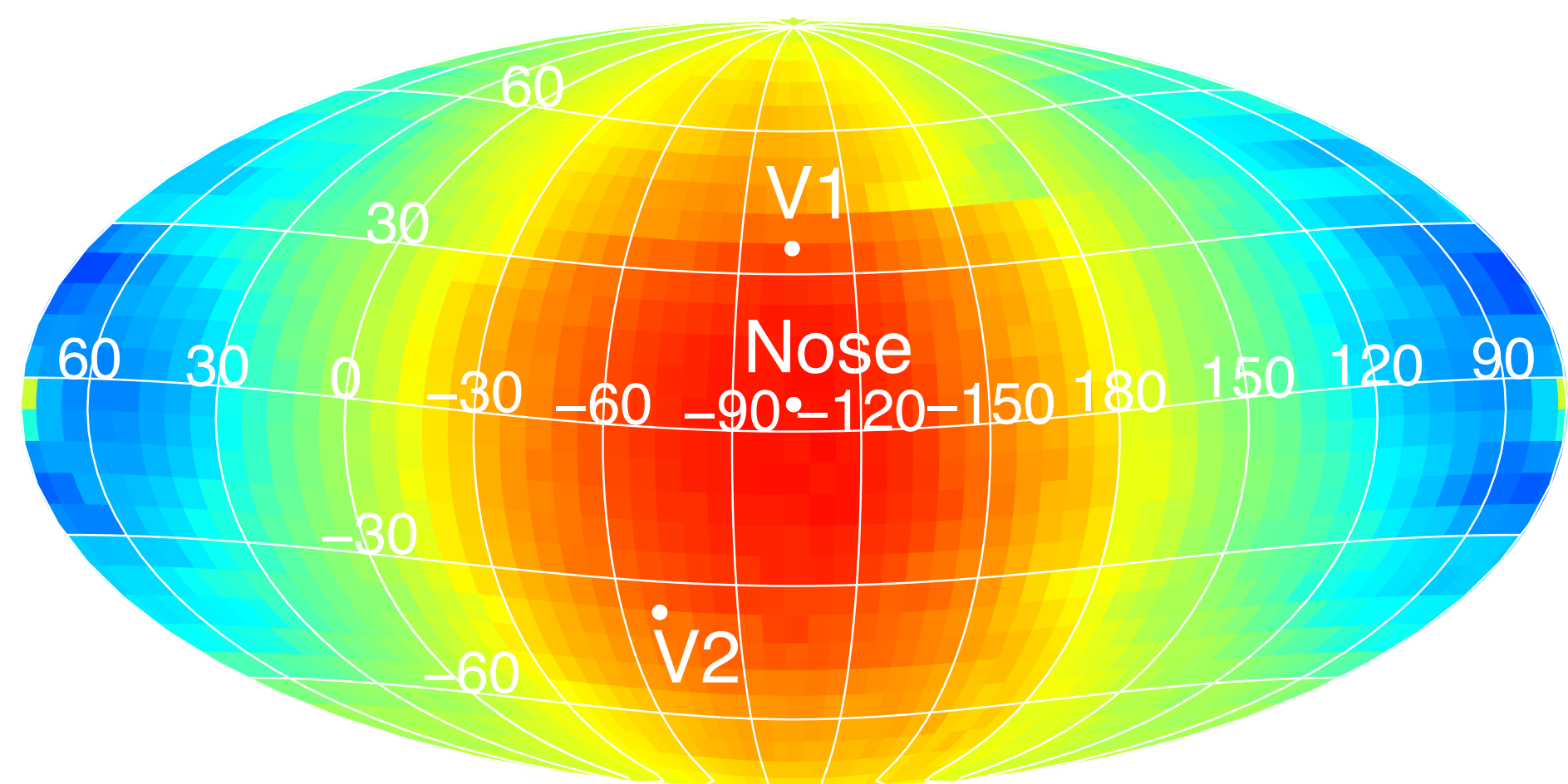
d ESA 6, t_{\text{IBEX}} = 2014\text{-}2016
