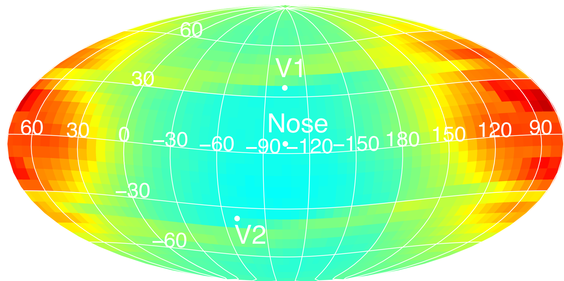
b ESA 3, t_{\text{IBEX}} = 2014\text{-}2016
