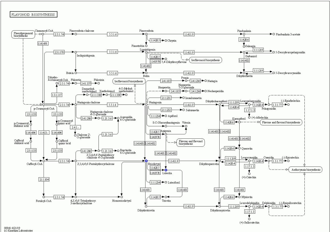
Supplementary Fig. 1 Coordinate down-regulation of metabolites involved in Flavonoid biosynthesis. The metabolic profile in Flavonoid biosynthesis pathway were down-regulated in Z1 vs. Z2. Blue circle indicated down-regulated metabolites.
