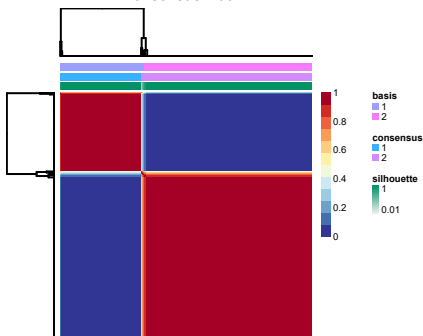
Consensus matrix
