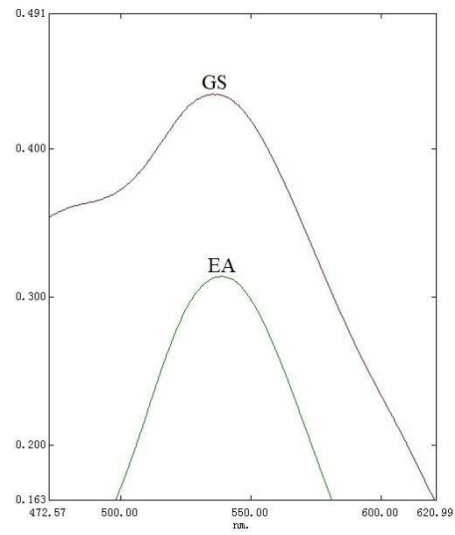
Supplementary Figure 1: Full wavelength scanning of EA in G.sinensis . GS: G.sinensis ; EA: cystic acid.
