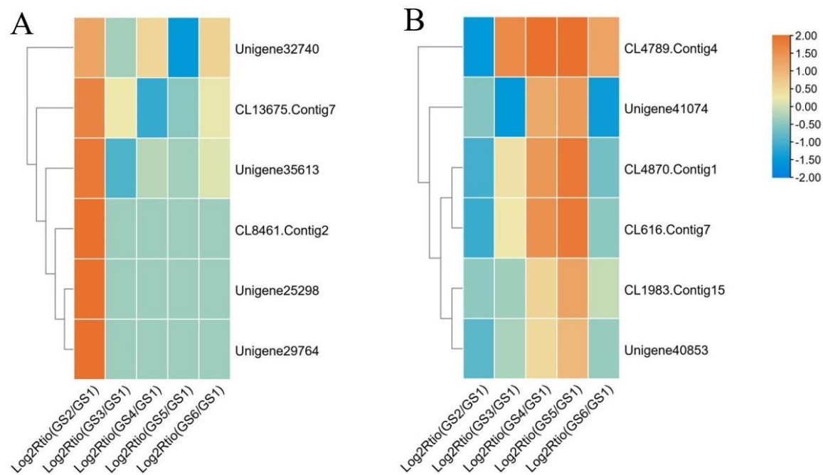
Supplementary Figure 6: Heatmap of Key genes screened by WGCNA. (A) Heatmap of Key genes in gleditsioside biosynthesis by WGCNA. (B) Heatmap of Key genes in pods development by WGCNA.
