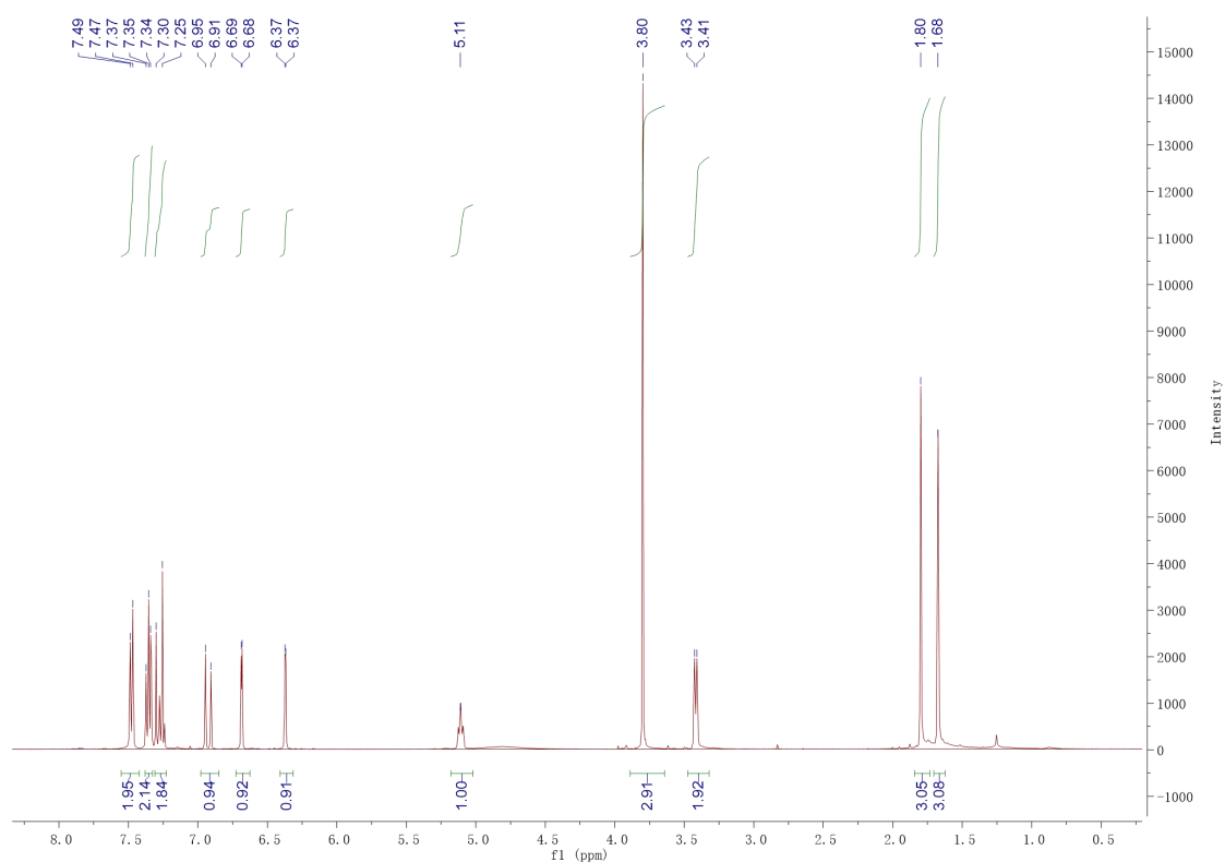
Fig. S4. The ^1\text{H} NMR spectrum of LLA in \text{CDCl}_3 , 400 MHz
