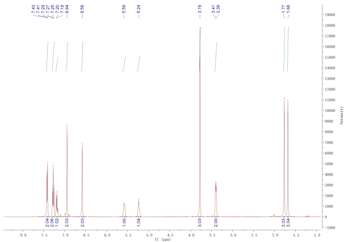
Fig. S7. 1 H NMR spectrum of LLC in CDCl 3 , 400 MHz
