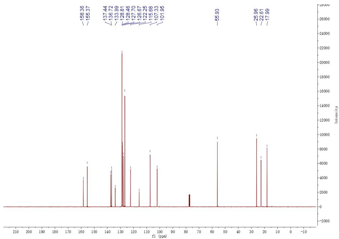
Fig. S8. The 13 C NMR spectrum of LLC in CDCl 3 , 100 MHz
