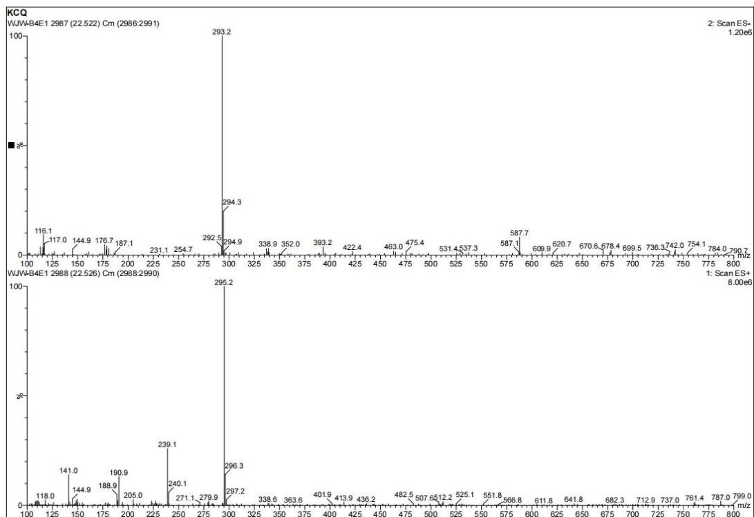
Fig. S6. The HRMS spectrum of LLA
