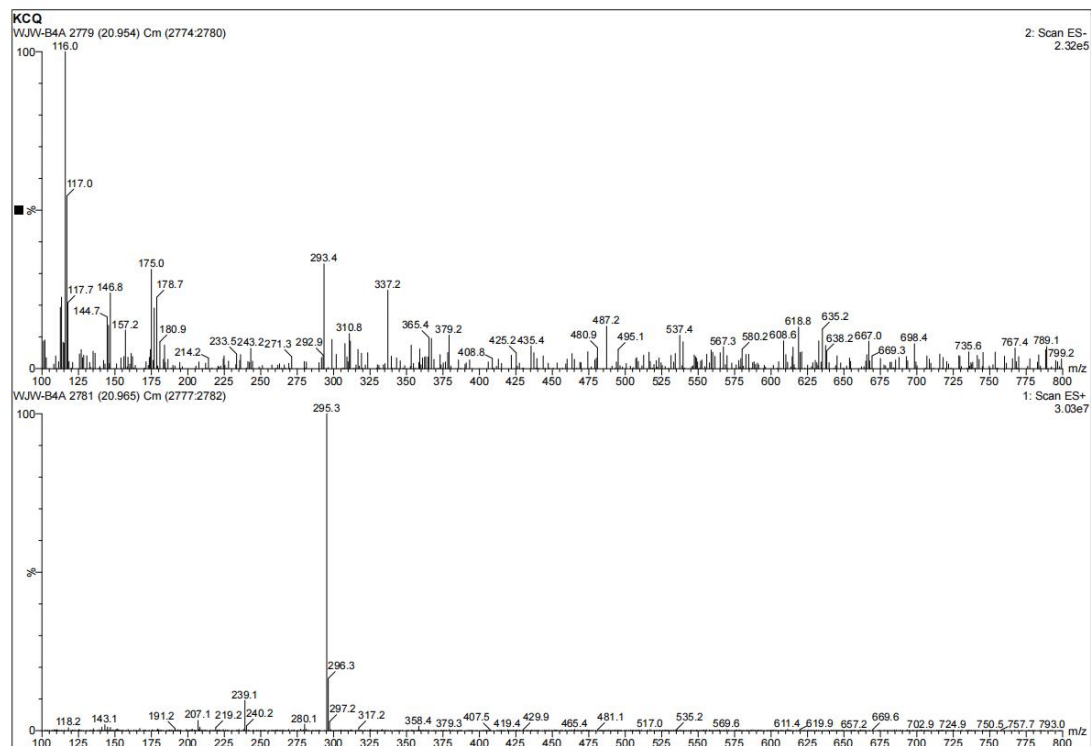
Fig. S9. The HRMS spectrum of LLC
