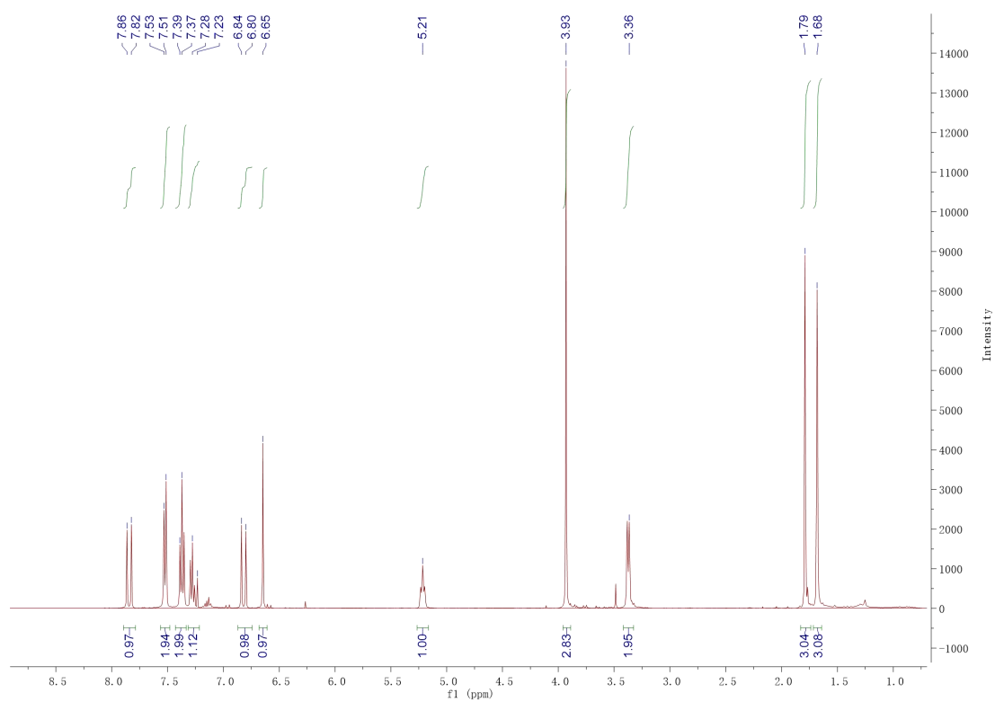
Fig. S1. The 1 H NMR spectrum of CSA in CDCl 3 , 400 MHz
