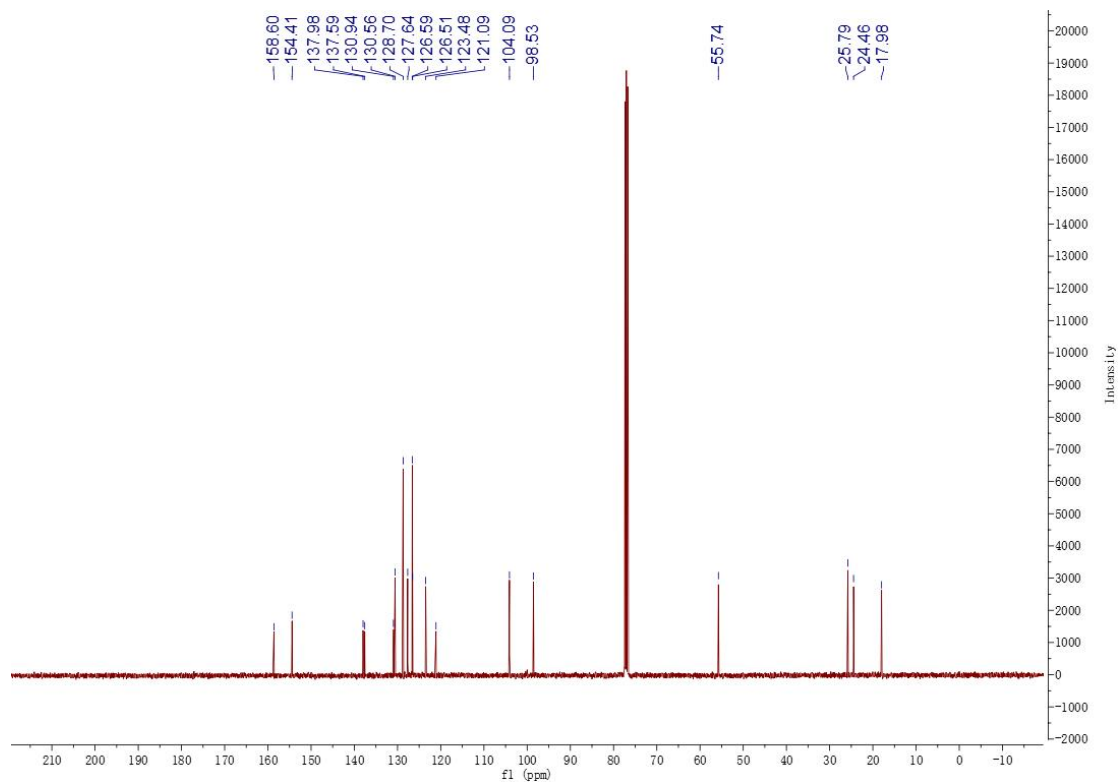
Fig. S5. The ^{13}\text{C} NMR spectrum of LLA in \text{CDCl}_3 , 100 MHz
