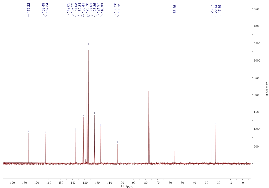
Fig. S2. The 13 C NMR spectrum of CSA in CDCl 3 , 100 MHz
