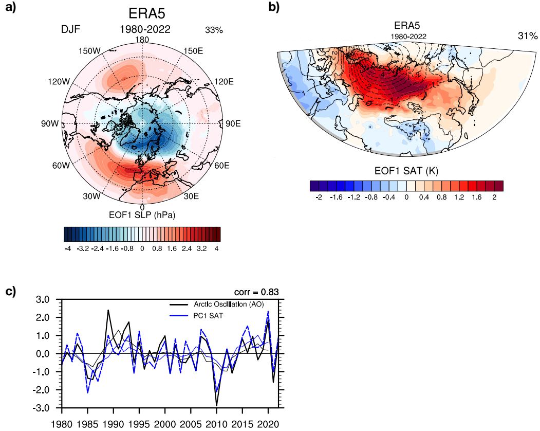
Fig S1 In the ERA5 reanalysis for the period 1980 to 2022 a) The EOF1 of observed winter (December-to-February) Northern Hemisphere (NH, 20°N-90°N, 180°W-180°E) SLP variability (known as Arctic Oscillation, AO) in hPa. b) the EOF1 of the observed winter Eurasian SAT variability in Kelvin (in shading) and contours show the associated sea level pressure anomaly, representing the AO. The top right of the figures mentions the explained variances. c) Associated time series of the PC1 NH SLP variability (in black) and the PC1 of the Eurasian SAT variability (in blue). The thin smoother time series represent the respective 5-year running means.
