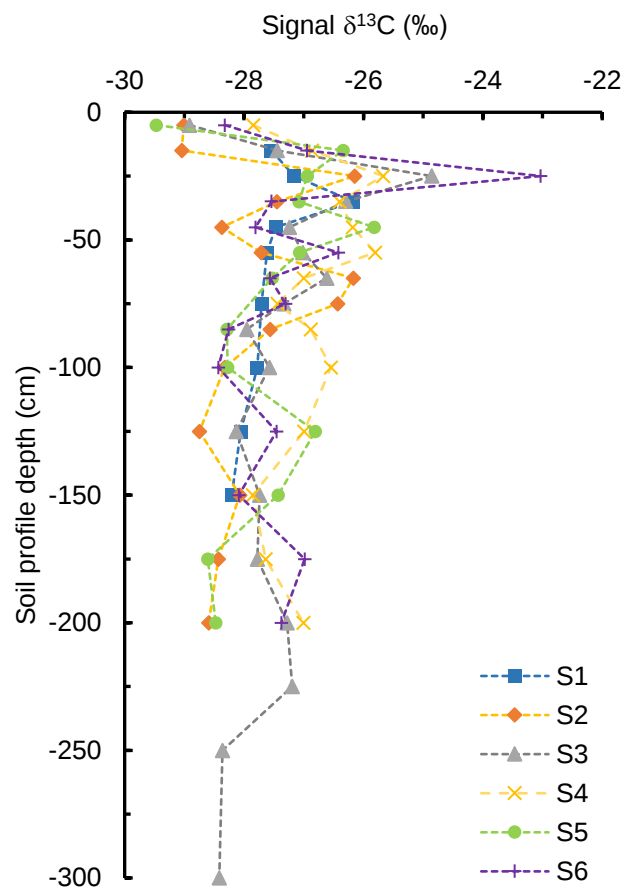
Fig. 4S Isotopic shift of \delta^{13}\text{C} of soil profiles from LRS (n=6), sampled between October 13, 2020 (S1, S2 and S3) and February 5, 2021 (S4, S5 and S6)
