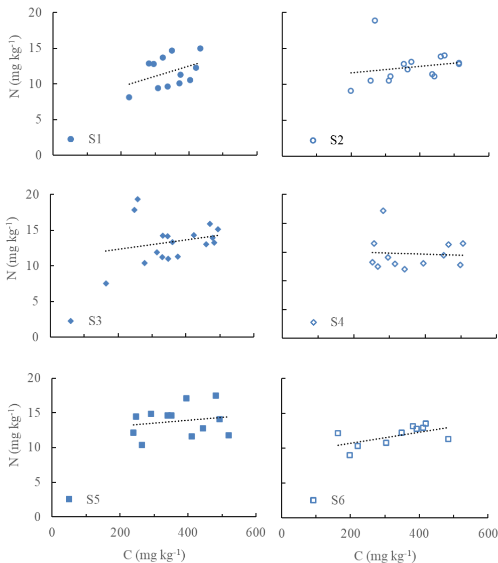
Fig. 3S Pearson correlation between total C and N in the soil profile. Positive at S6, the Cuba palm islet (0.59), moderate at S1 (0.40) and weak in the S2 (0.20), S3 (0.22), S5(0.18). The Pearson correlation was negative and weak in S4 (-0.05)
