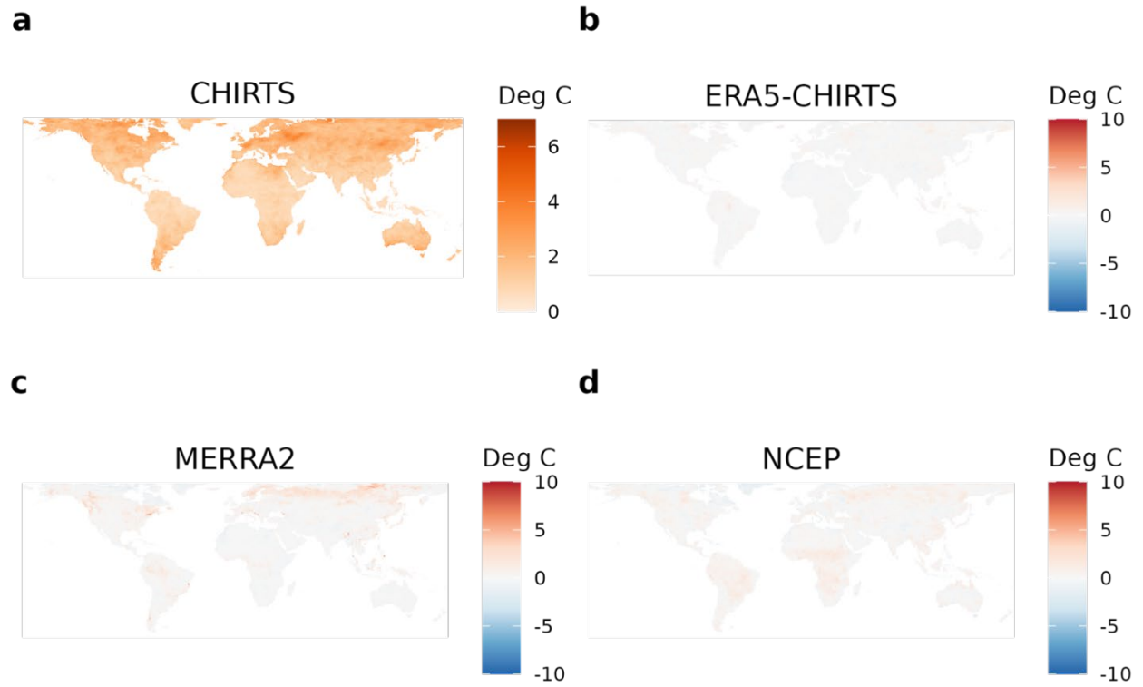
Figure SI-1: Length of the tail of daily maximum temperatures 1983-2015, calculated as the 99.9th percentile minus the 99.5th percentile. Absolute values are shown in (a) for the CHIRTS dataset, and the difference between the reanalysis and CHIRTS is shown for (b) ERA5, (c) MERRA2, and (d) NCEP.
