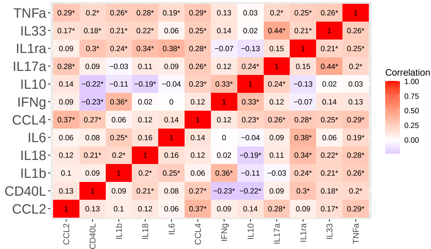
Correlation Heatmap
