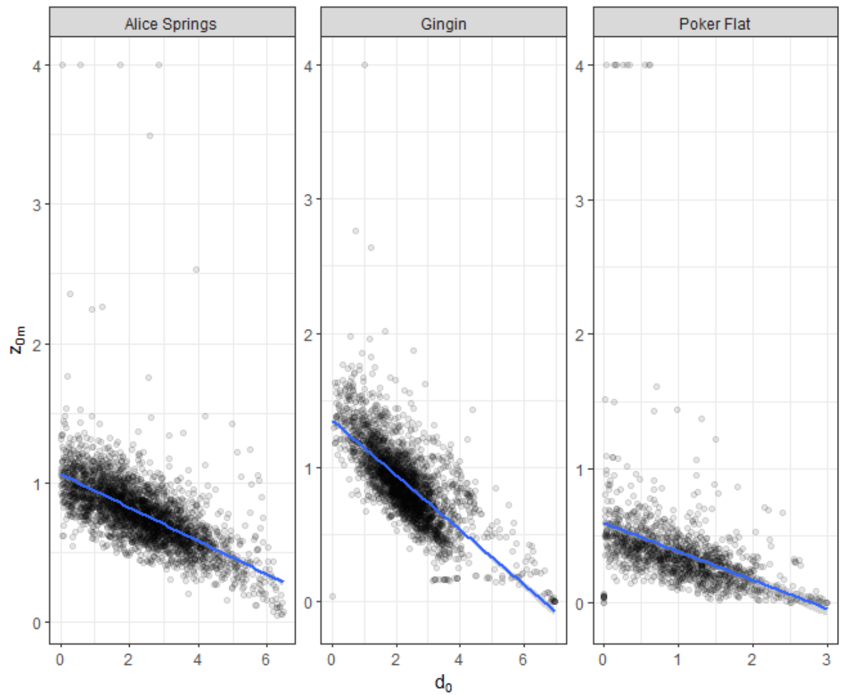
FIGURE S4: RELATIONSHIP BETWEEN d_0 AND z_{0m} AT SITES WHERE THEY ARE CALCULATED SIMULTANEOUSLY
