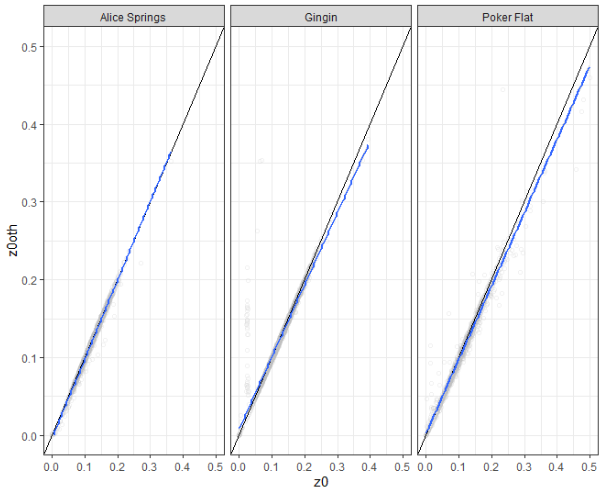
FIGURE S3: COMPARISON OF z_{0m} FROM USING FIXED d_0 (Y-AXIS) AND WITH VARIABLE d_0 (X-AXIS) FOR THREE SITES WITH MORE THAN 2 SENSORS
