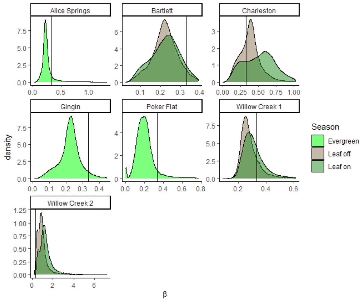
FIGURE S8: PROBABILITY DENSITY FUNCTION OF \beta MEASURED AT DIFFERENT SITES AND SEASONS. THE VERTICAL LINE REPRESENTS \beta = 1/3 WHICH IS ESTIMATED TO BE ITS MAXIMUM THEORETICAL VALUE.
