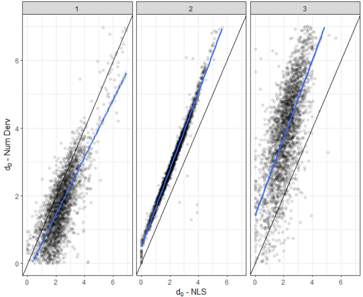
FIGURE S2: NUMERICAL DERIVATIVE (Y-AXIS) AND NLS d_0 COMPARISON FOR THREE DIFFERENT HEIGHTS (GIVEN AS 3 DIFFERENT PANELS) FOR GINGIN
