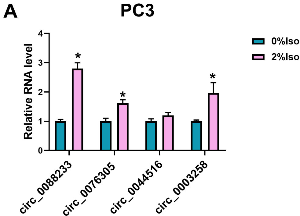
Fig. S1 The screening of circ_0088233. (A) The expression of circ_0088233, circ_0076305, circ_0044516 and circ_0003258 in PC3 cells treated with or without Iso was examined by qPCR. * P < 0.05 , ANOVA was used for difference comparison.
