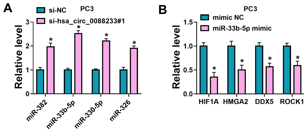
Fig. S2 The screening of miR-33b-5p and HIF1A. (A) The expression of miR-382, miR-33b-5p, miR-330-5p and miR-326 in PC3 cells with circ_0088233 knockdown was checked by qPCR. (B) The expression of HIF1A, HMGA2, DDX5 and ROCK1 in PC3 cells overexpressing miR-33b-5p was checked by qPCR. * P < 0.05 , ANOVA was
