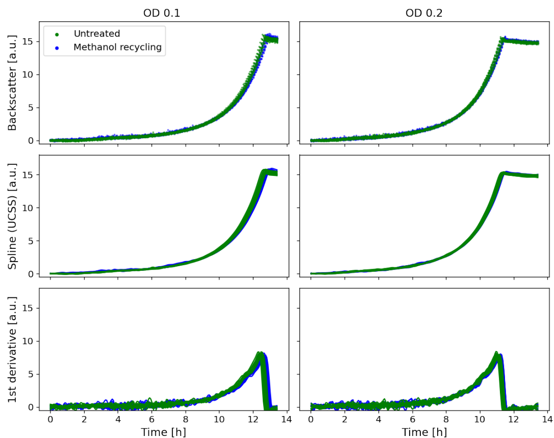
Figure S4: Exemplary spline analysis for C. glutamicum .
