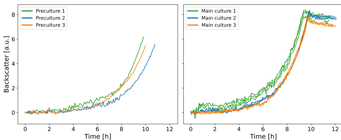
Figure S8: Backscatter trajectories for LipA in strategy with replicates spread over several batches.
