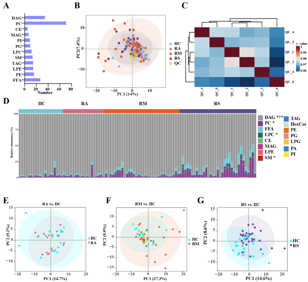
Figure S3. (A) The number of identified lipids subclasses. (B) The PCA score plot shows the clustering of quality control (QC) samples from recovered asymptomatic patients (RAs), recovered moderate patients (RMs), and recovered severe and critical patients (RSs), and healthy controls (HCs). (C) The correlation coefficient of QC samples was indicated with Pearson correlation. (D) This graph represents the average percentage of lipids subclasses of each sample from HCs, RAs, RMs, and RSs. (E–G) PCA score plots of lipid profiles detected in plasma sEVs in RAs (E), RMs (F), and RCs (G) compared with HCs, respectively. p-value: * p < 0.05 ; ** p < 0.01 ; *** p < 0.001 .
