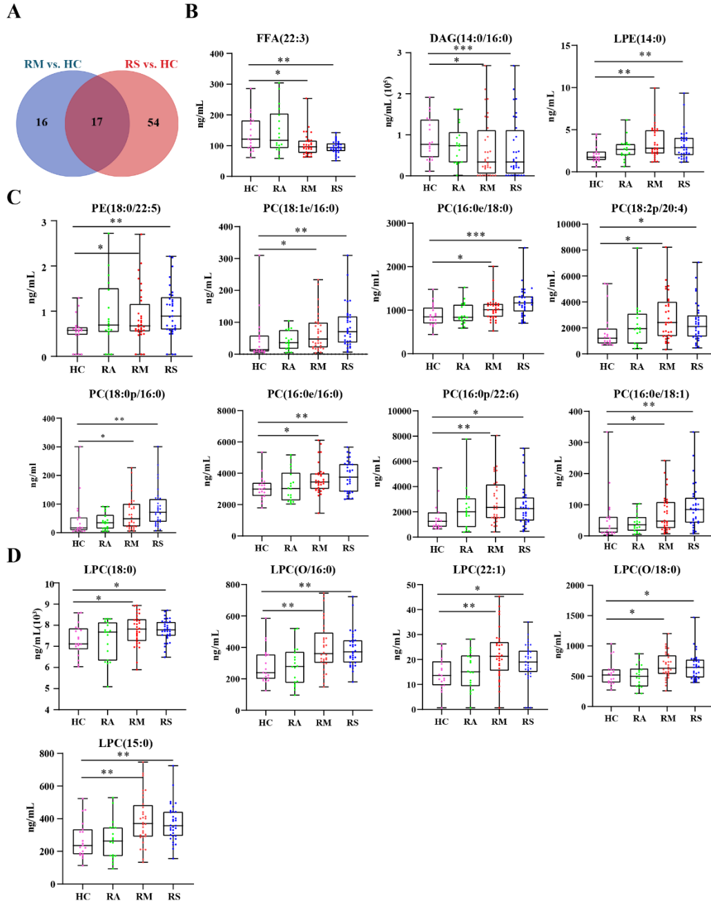
Figure S4. Significantly altered lipids in RM and RS compared to HCs. (A) Venn diagram showing the number of significantly changed lipids in recovered moderate patients (RMs) and recovered severe and critical patients (RSs) relative to healthy controls (HCs). (B–D) The significance of comparisons of the four groups was determined by the Kruskal-Wallis test (data with non-normal distribution) or one-way ANOVA (data with normal distribution) and indicated as an absolute overall p-value. * p < 0.05 ; ** p < 0.01 ; *** p < 0.001 .
