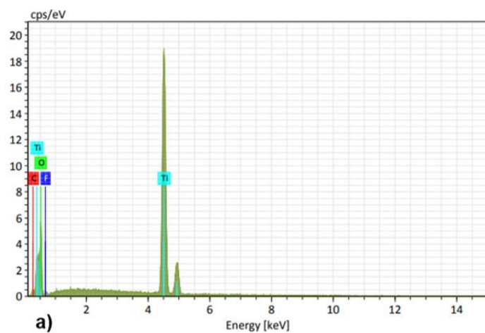
FigS2 a) EDS analysis and b) EDS mapping analysis of the TiO 2 NTs electrode.
