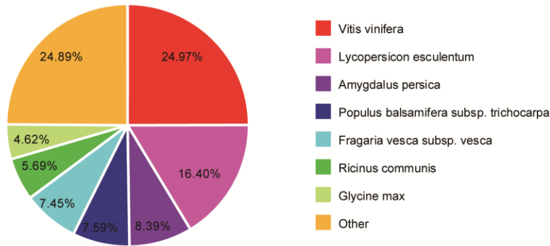
Supplementary Fig 1. Comparative results of unigenes public database function annotations
