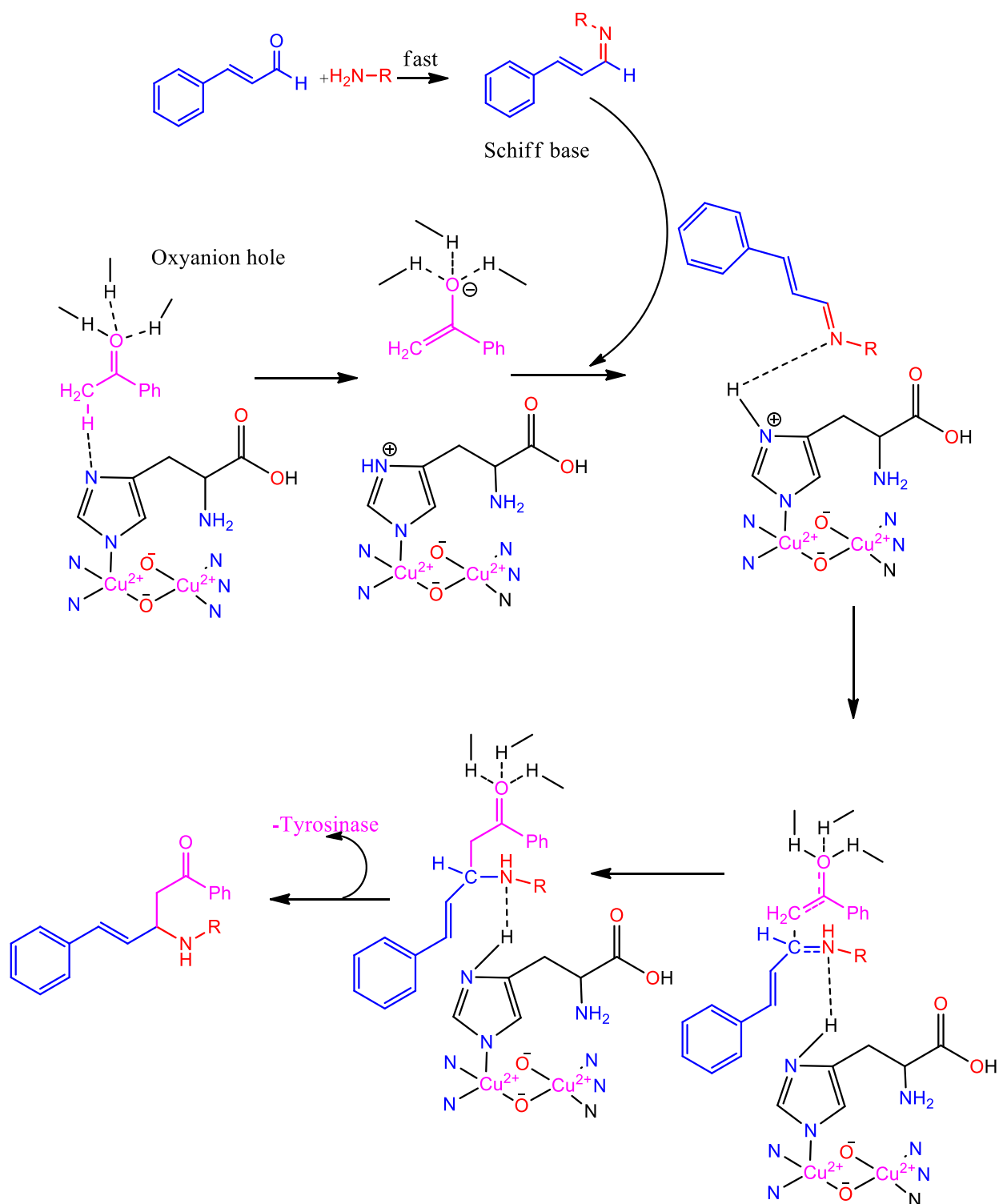
Scheme 2. Proposed mechanism of Mannich base derivative formation.
