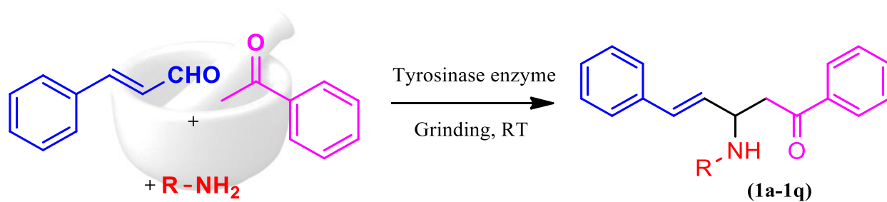
Scheme 1. Synthetic route of Mannich base derivative preparation.
