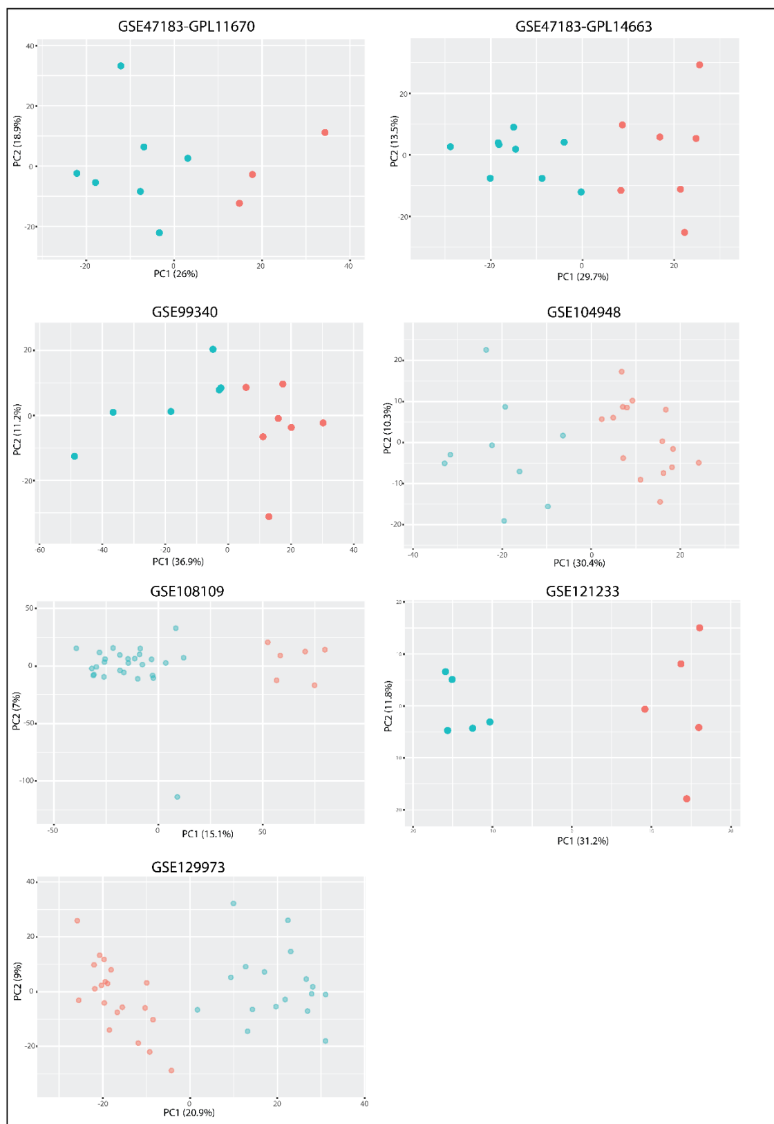
Figure S1: PCA plots for each of datasets included in the meta-analysis
