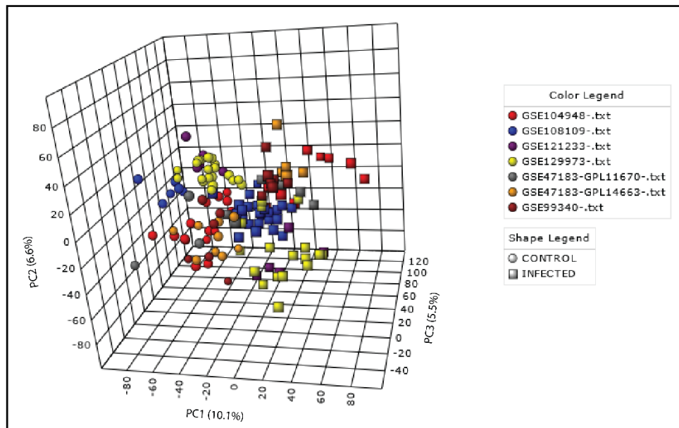
Figure S2: Three-dimensional PCA plot to ensure the separation of the case and control samples after batch effect removal
