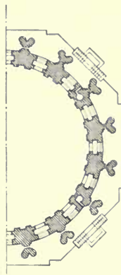
PLAN OF PERISTYLE OF EXISTING DOME BY MICHAELANGELO.
