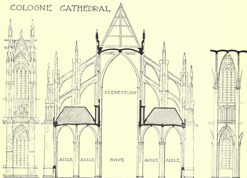
EXTERIOR ELEVATION OF AISLE WALL & CLERESTORY
