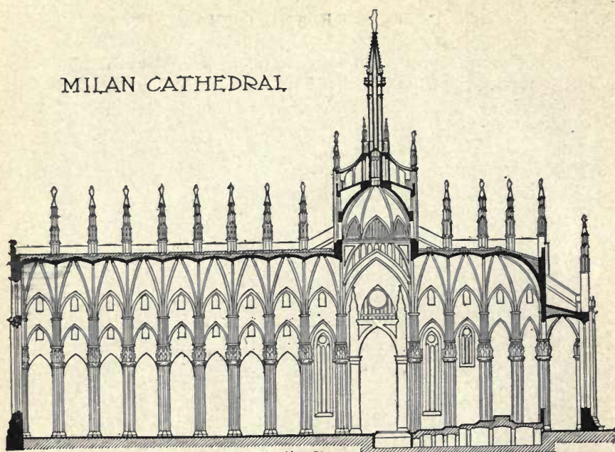
LONGITUDINAL SECTION, (a)
