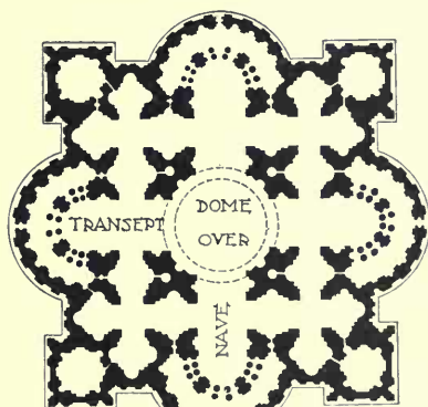
PLAN OF ST. PETERS BY PERUZZI AD 1520.
