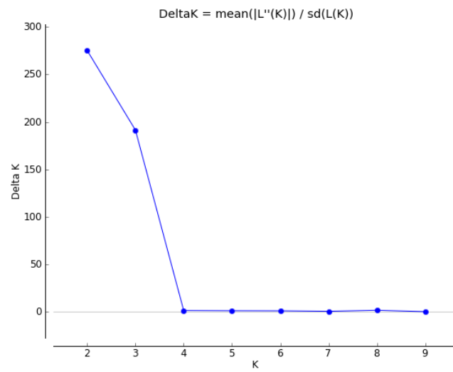
Figure S.1. Optimum number of cluster observed from STRUCTURE analysis.
