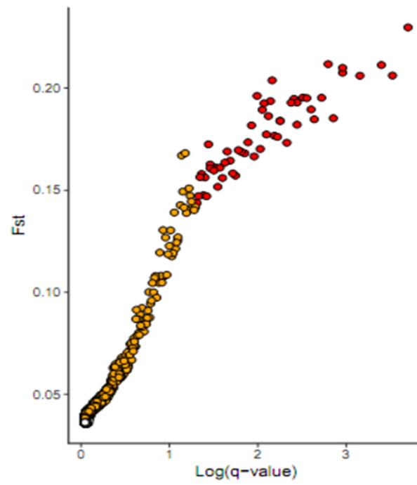
Figure S.3. Outlier locus distribution (red spot) acquired from BayeScan.
