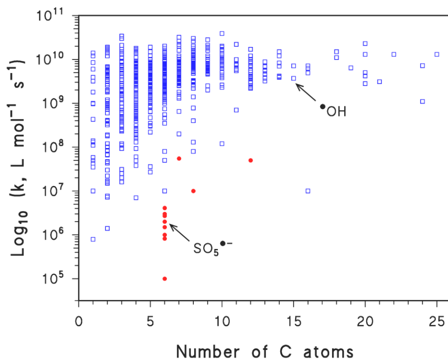
Figure S3. Second-order reaction rate constants of \bullet\text{OH} and \text{SO}_5^{\bullet-} with organic compounds, ordered according to the number of C atoms, from: Buxton et al. (1988), Neta et al. (1988).
