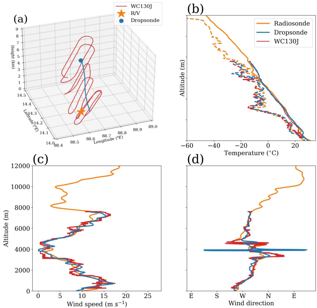
Figure S1: (a) Descents of WC130J aircraft and dropsonde on 17 June 2018. The star shows location of R/V Thomas G. Thompson in the Bay of Bengal. (b) Dry bulb temperature (solid) and dewpoint (dashed) profiles from dropsonde (0757 UTC), radiosonde (0521 UTC) and WC130J onboard sensors (0757 - 0934 UTC). (c), (d) Same as (b) but show wind speed and wind direction, respectively. The aircraft descended to an altitude of 274 m above sea level.
